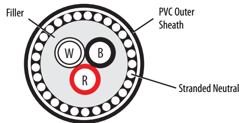
Figure 10 - European Style Multi-conductor Cable
