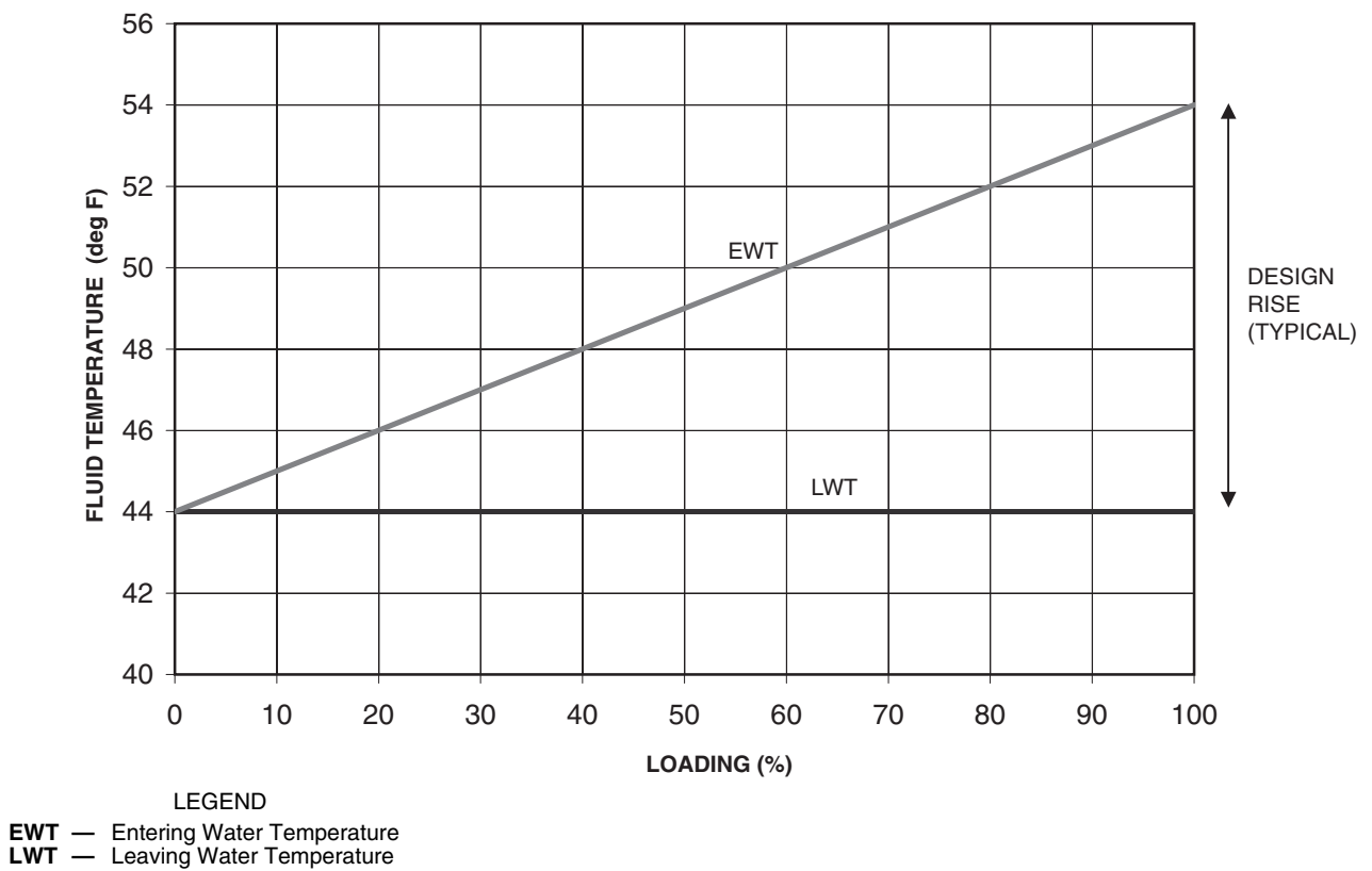
Fig. 16 — Chilled Water Temperature Control
