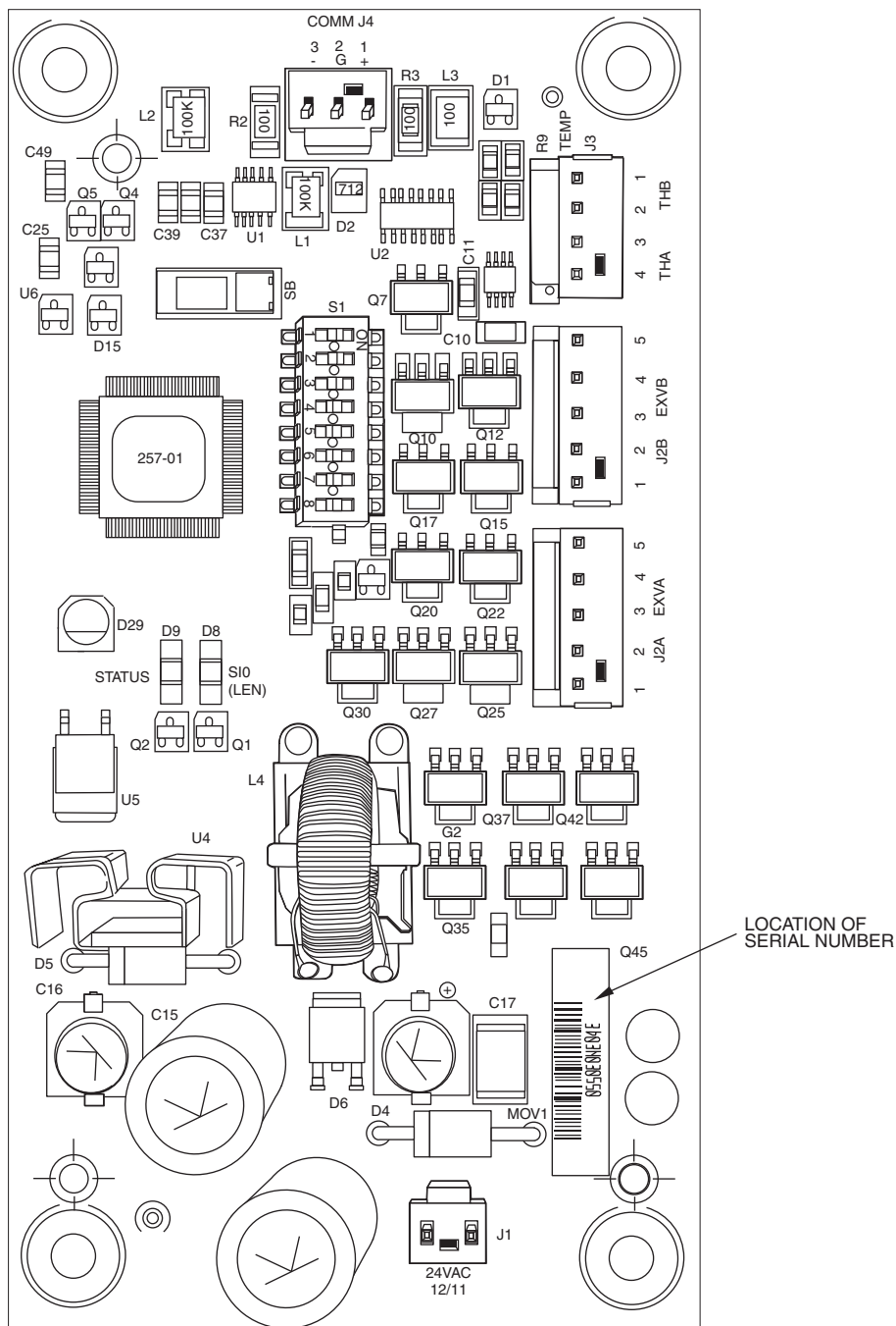
Fig. 5 — EXV Board
