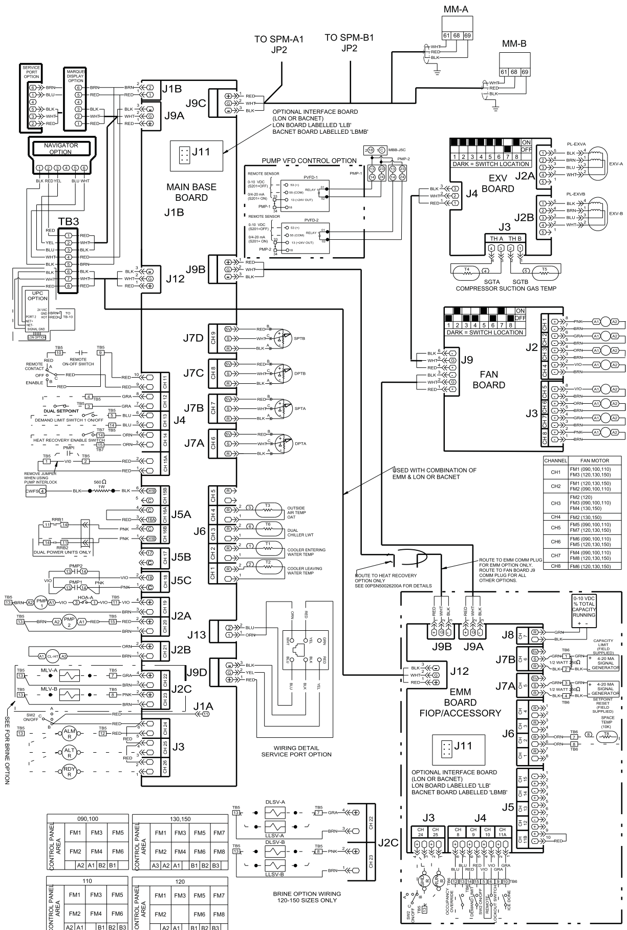
→ Fig. 39 — Control Schematic, 30RB090-150
