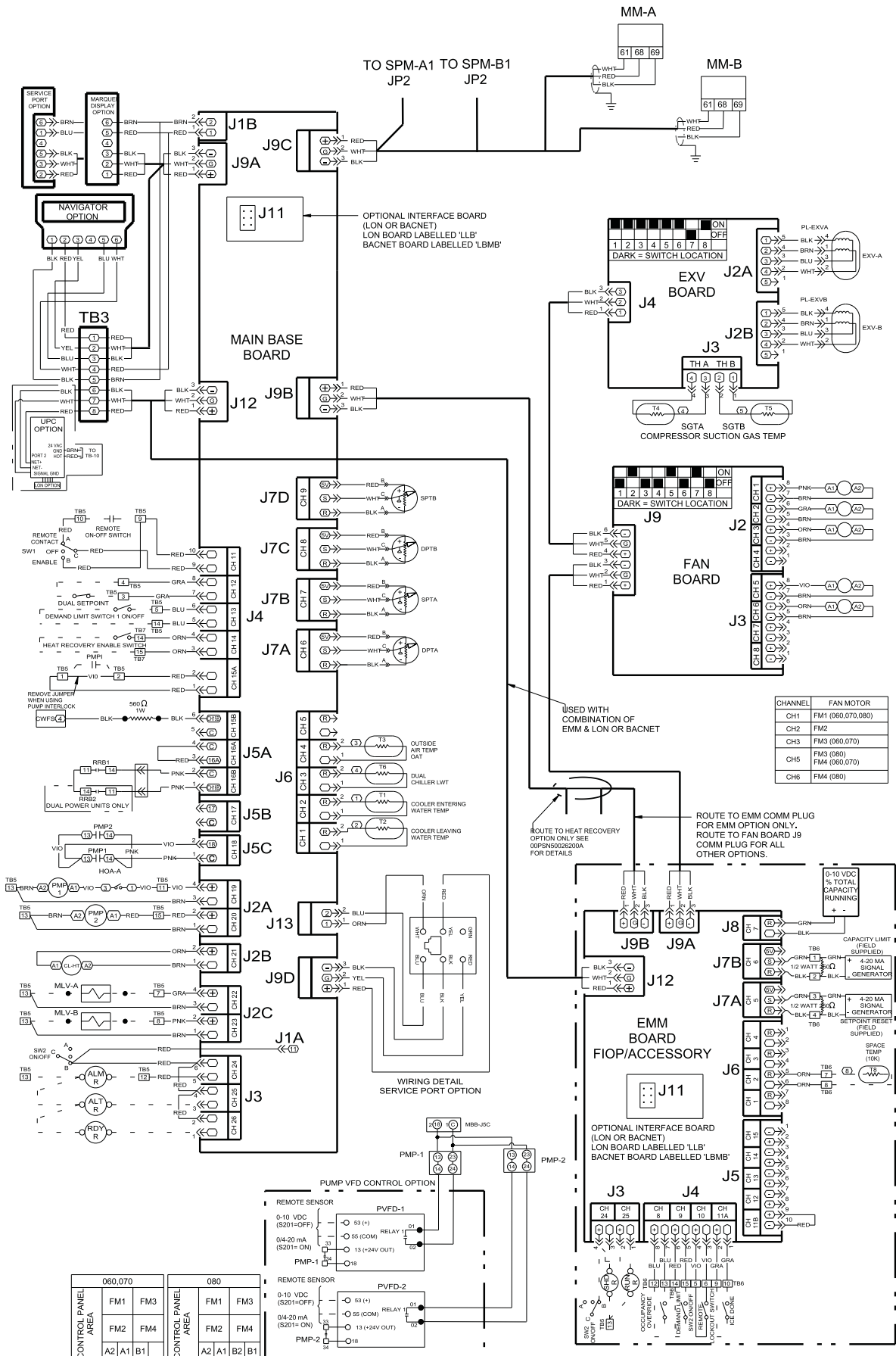
→ Fig. 38 — Control Schematic, 30RB060-080
