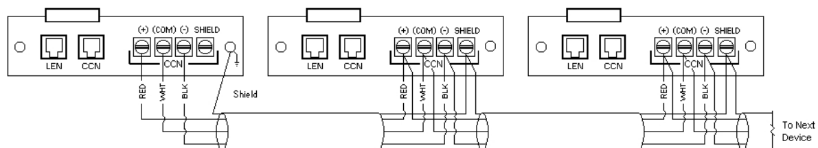
Fig. 10 — ComfortLink CCN Communication Wiring
