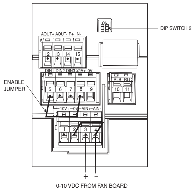
Fig. H — Low Ambient Temperature Control Signal Wiring
