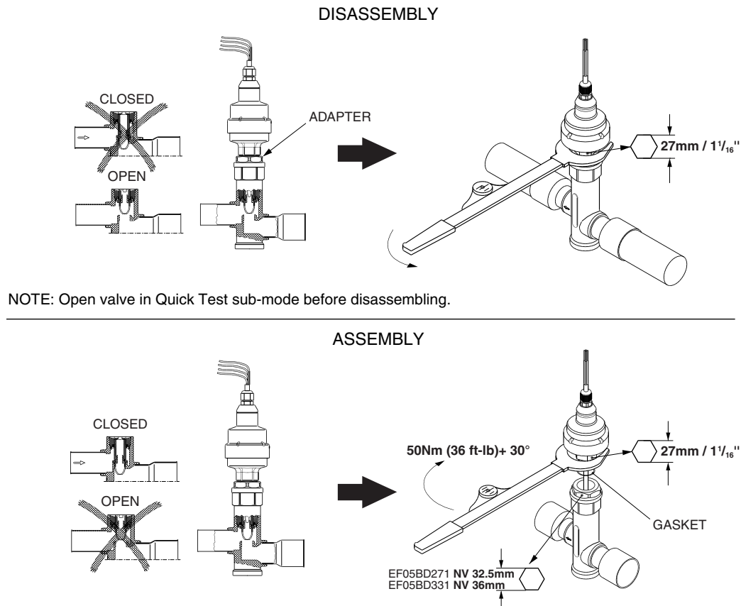
Fig. 27 — Disassembly and Assembly of EXV Motor
