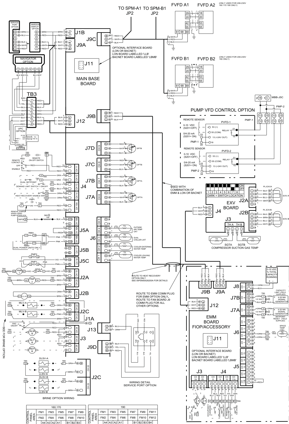
→ Fig. 43 — Control Schematic, 30RB160-190 with HEVCF Option
