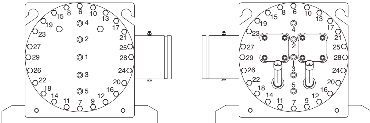
Fig. 31 — Bolt Tightening Sequence, 30RB110-130
