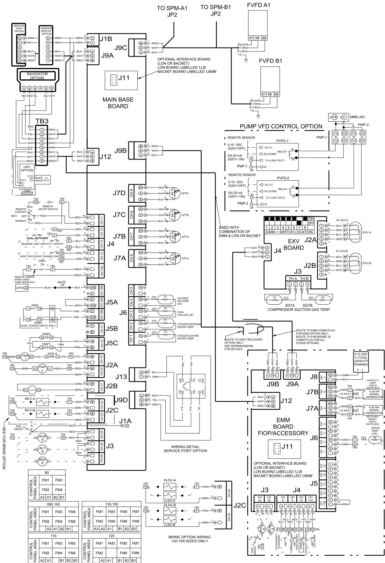
→ Fig. 42 — Control Schematic, 30RB080-150 with HEVCF Option
