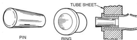
Fig. 28 — Elliott Tube Plug
