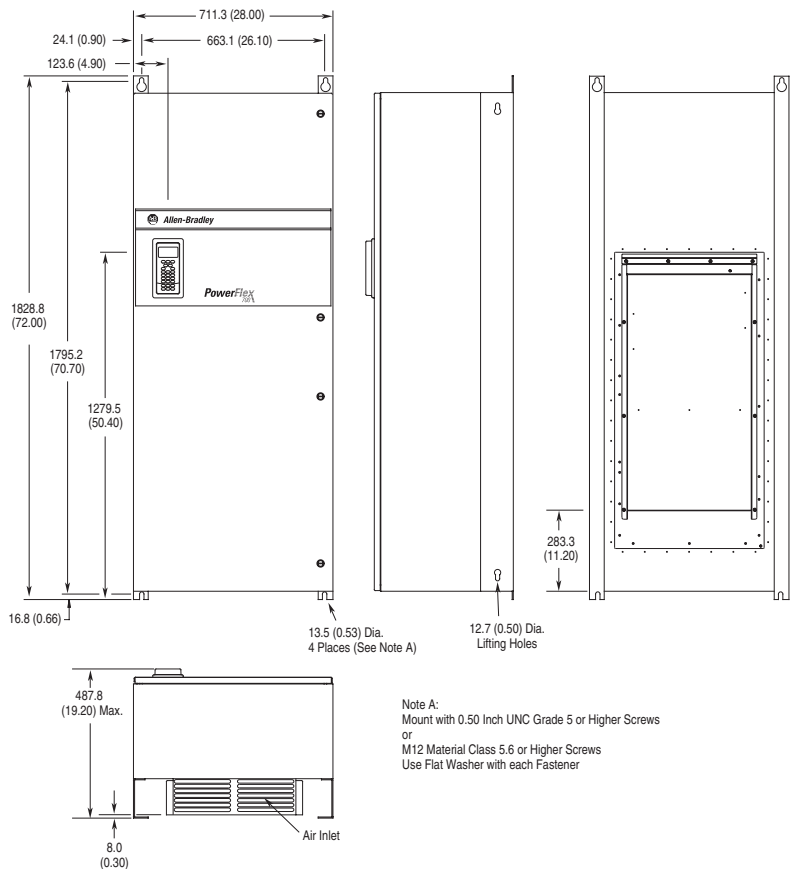
Figure A.11 Frame 6 NEMA Type 12 Standalone
