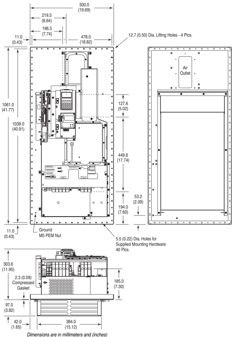
Figure A.9 Frame 5 NEMA Type 12 Flange Mount
