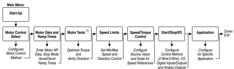
Figure 2.2 Start Up Menu
