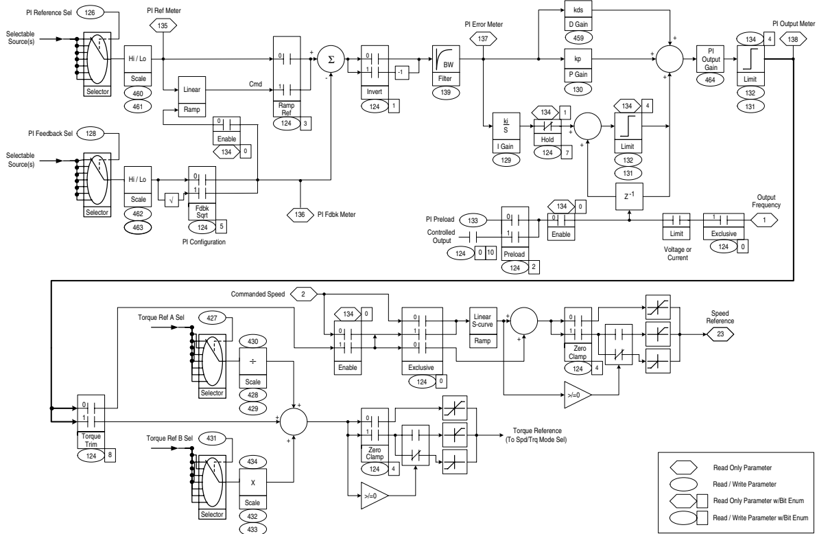
Figure C.13 Process Trim
