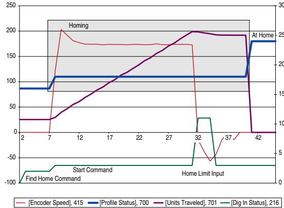
Figure C.5 Homing to Marker
