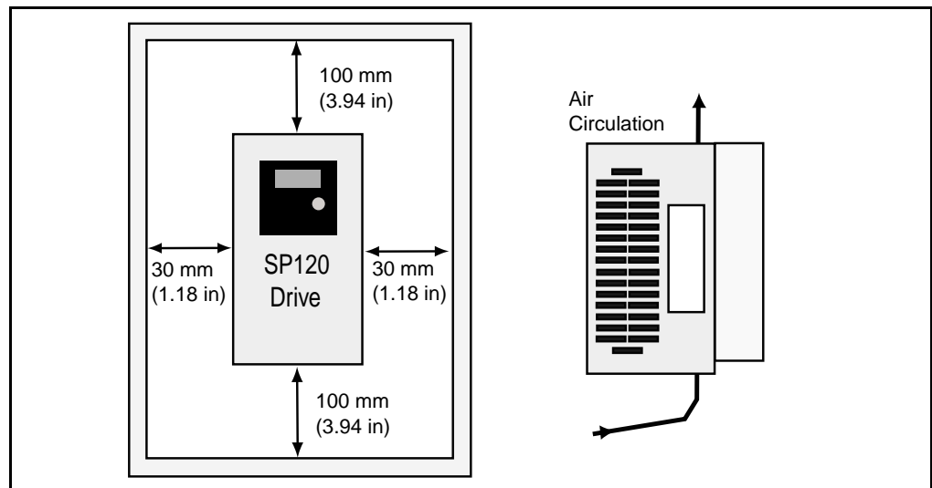
Figure 2.1 – Minimum Airflow Clearances
