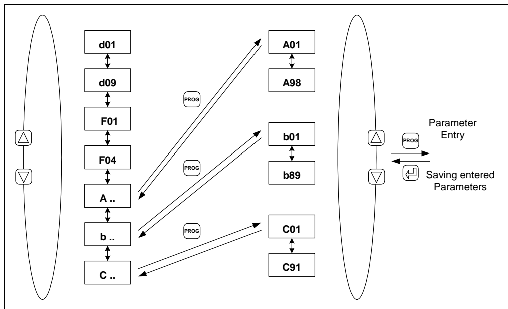
Figure 3.1 – Programming Overview
