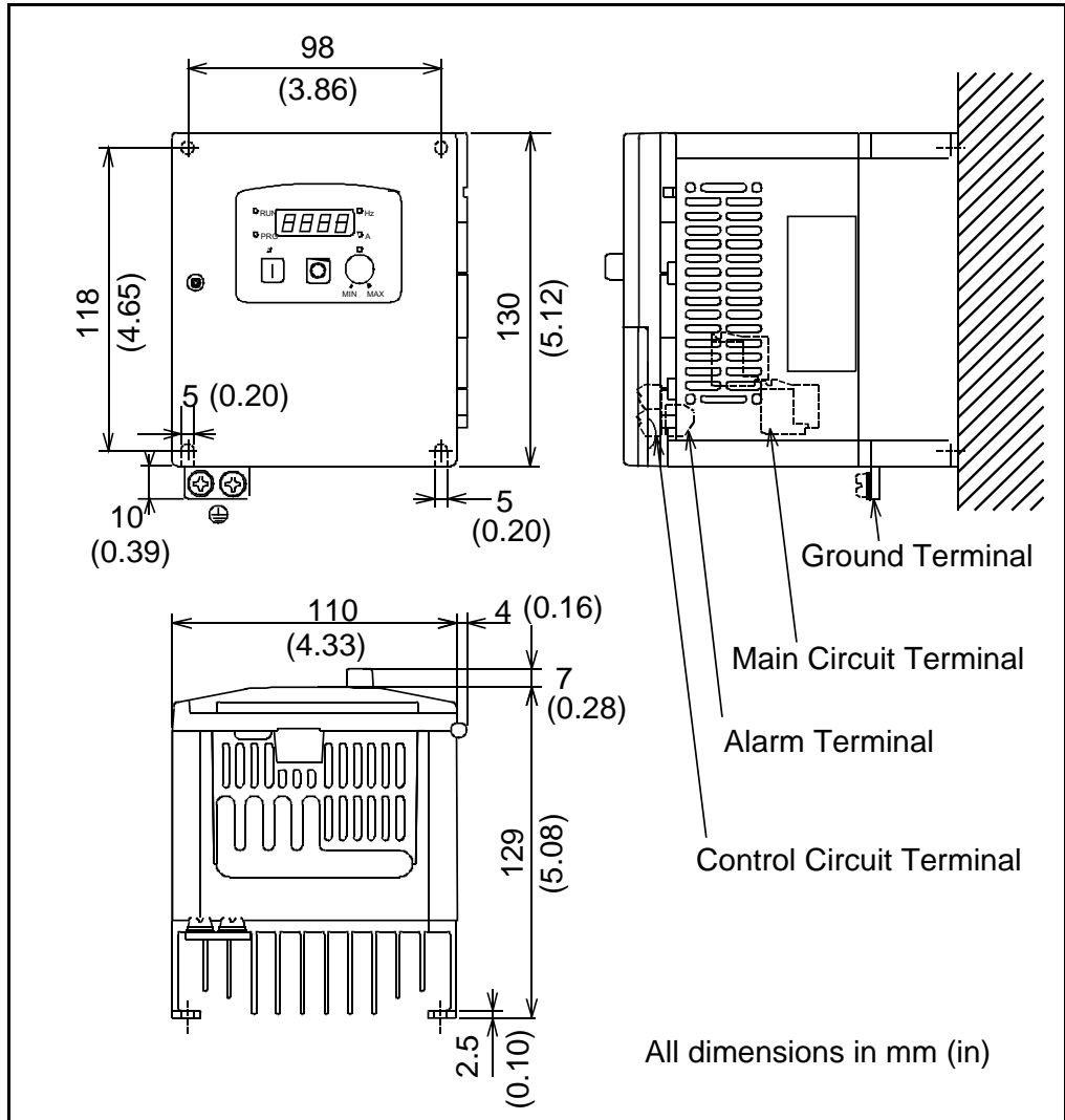
Figure A.2 – S12-204P0 / 205P0 / 401P5 Dimensions
