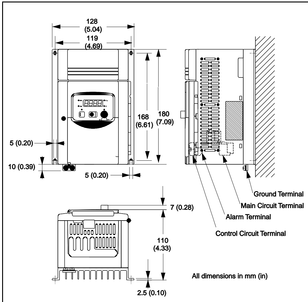
Figure A.6 – S12-104P0 Dimensions
