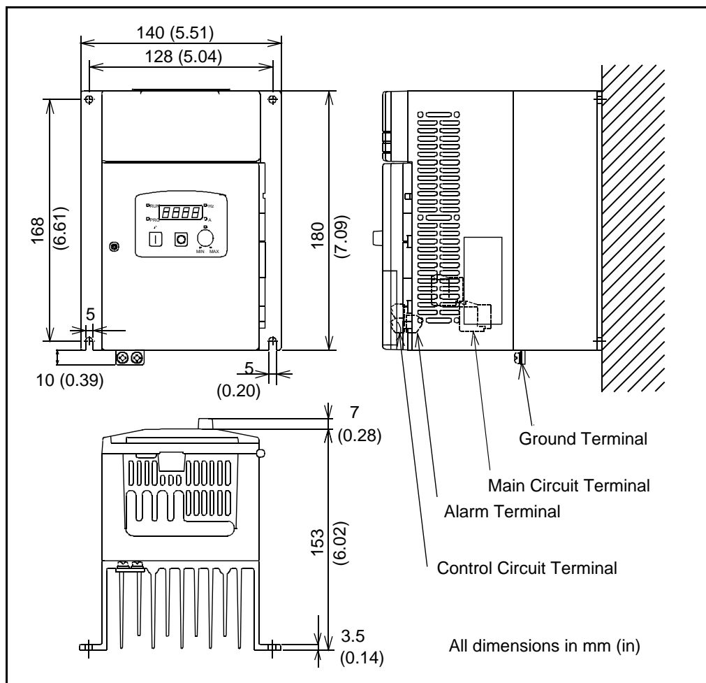
Figure A.3 – S12-207P1 Dimensions
