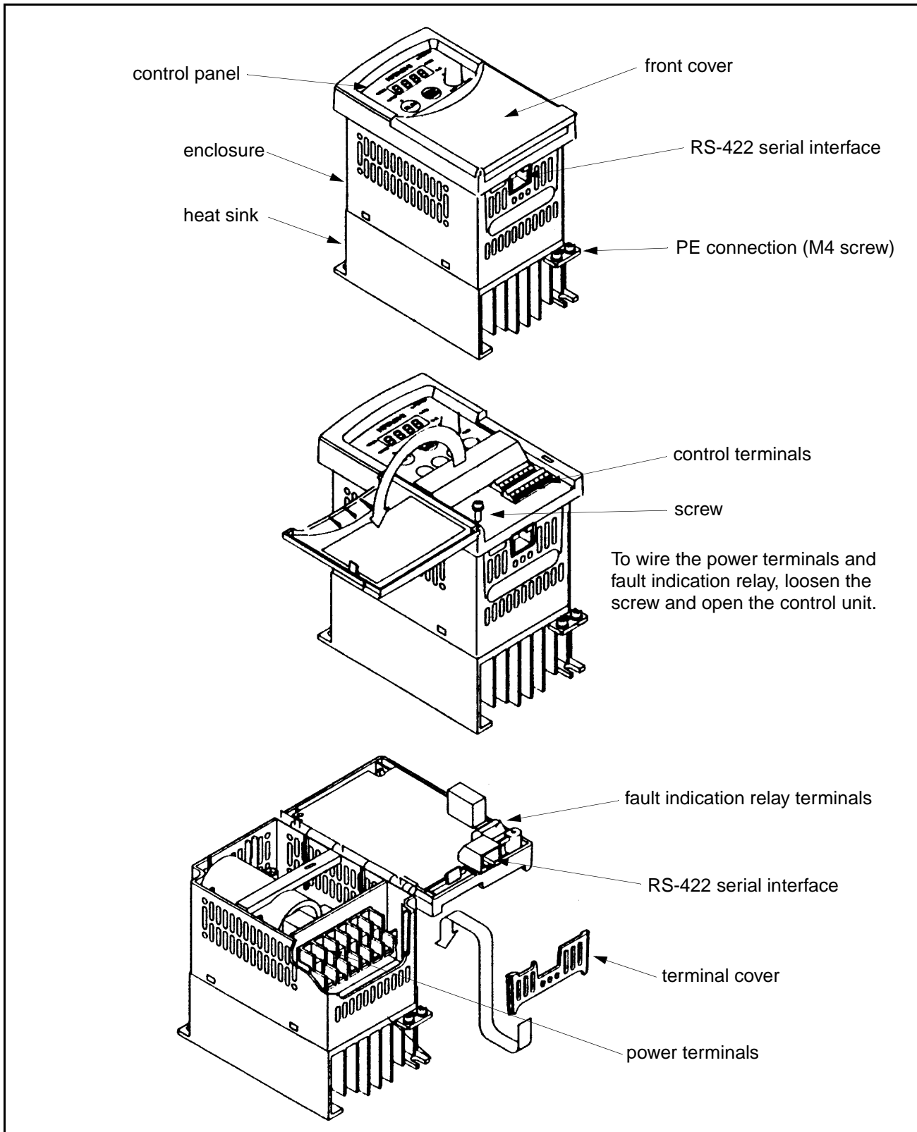
Figure 1.3 – Drive Features
