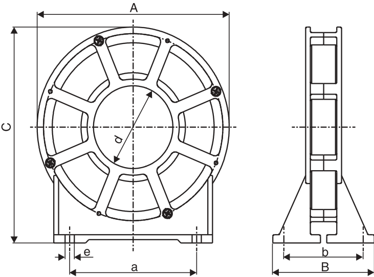
Figure 36: Dimensions, HD
