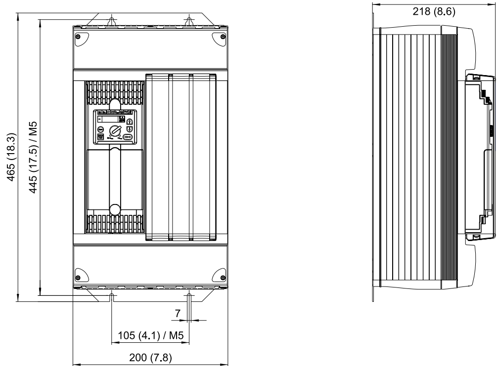
Figure 29: Dimensions, MOVITRAC® 07 size 3
