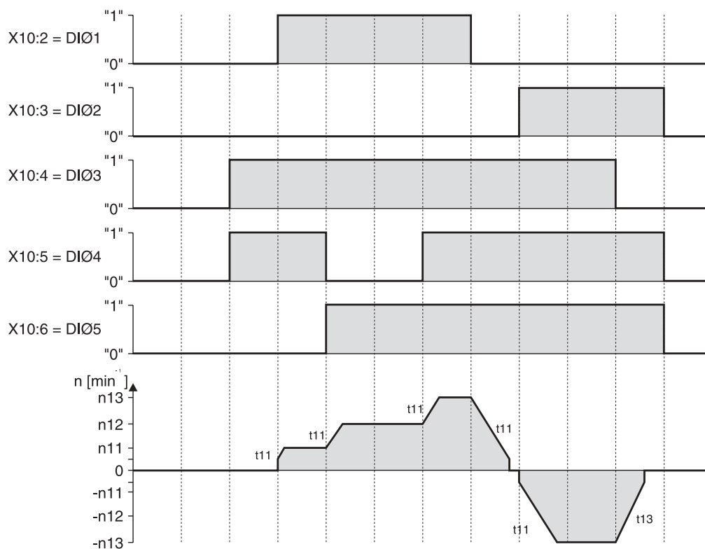
Figure 83: Travel cycle with internal fixed setpoints
