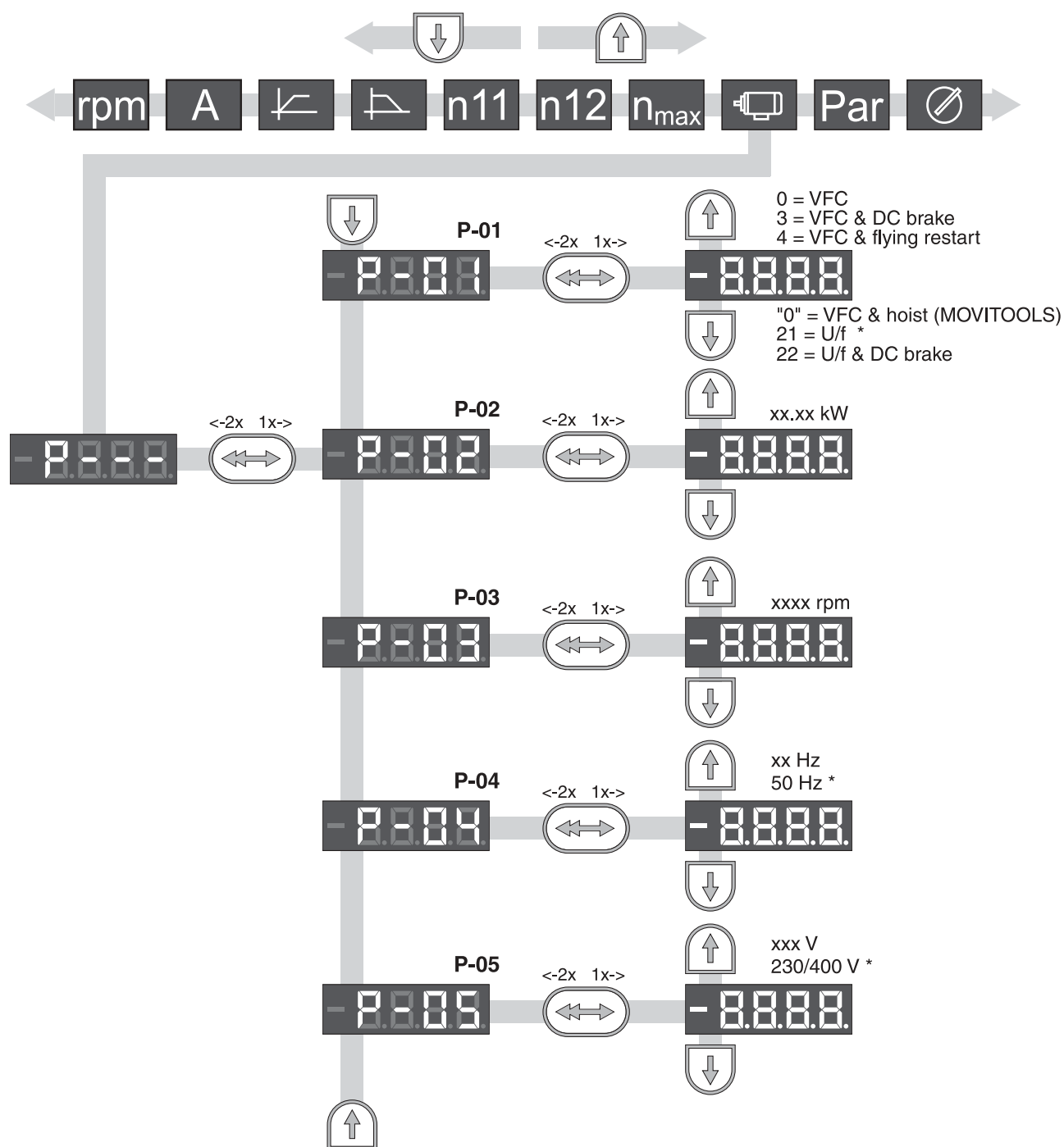
Figure 82: Startup with the integrated operating panel (2x = double-click / * = factory setting)
