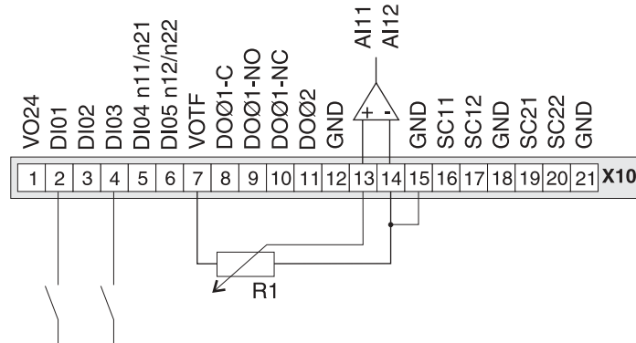
Figure 61: External setpoint potentiometer with DI01 = CW/STOP / DI02 = CCW/STOP / DI03 = Enable / DO02 = Brake 05324AXX
