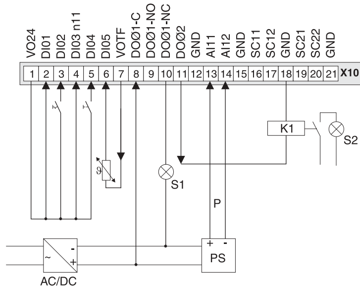
Figure 63: Pressure control connection with DI01 = CCW/STOP / DI02 = Enable / DI04 = Fault reset / DI05 = TF fault / DO01-C and DO01-NO = "Fault" / DO02 = "Pressure reached"
