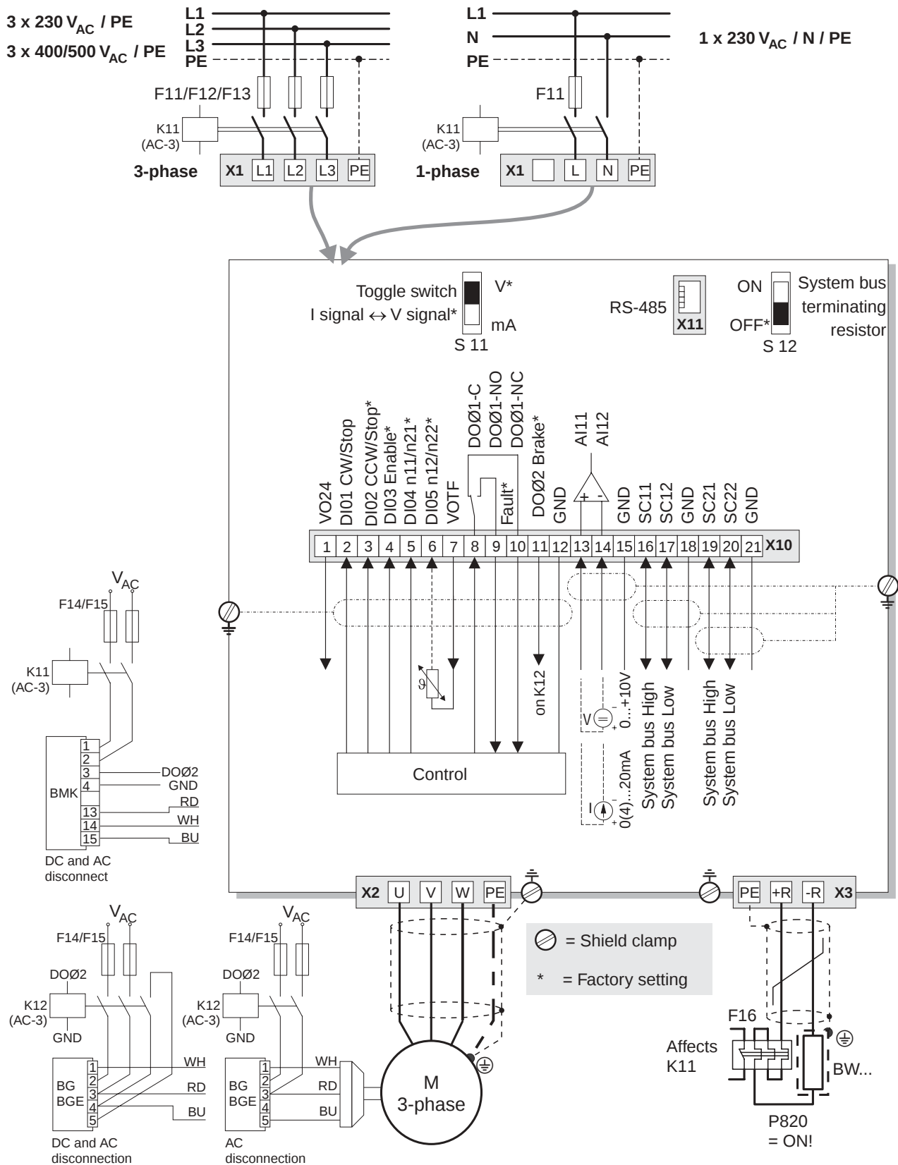
Figure 77: Wiring diagram for size 0
