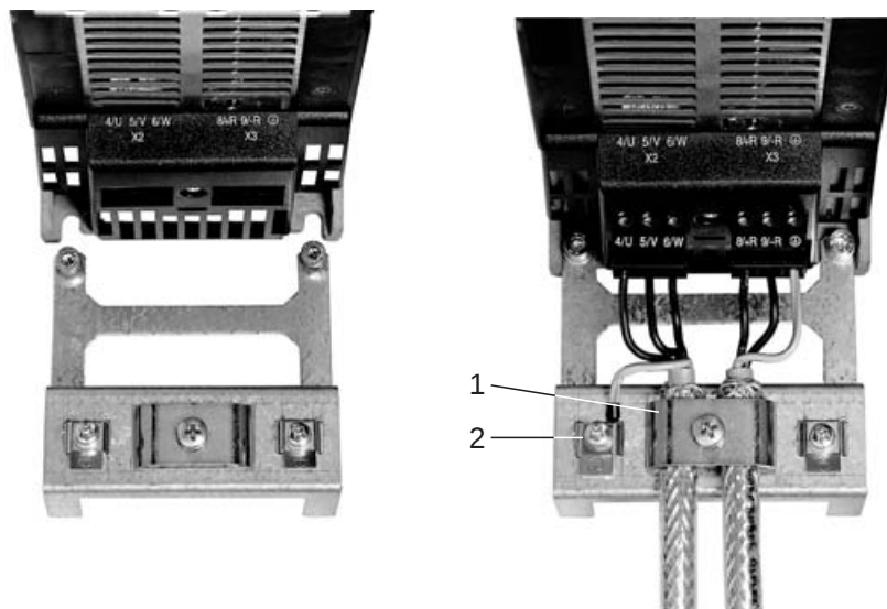
Figure 74: Power shield clamp for MOVITRAC® 07 size 1
