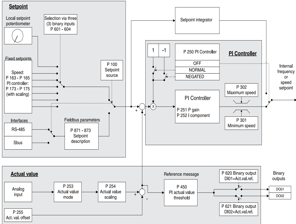
Figure 59: Structural diagram showing the implementation of the PI-controller
