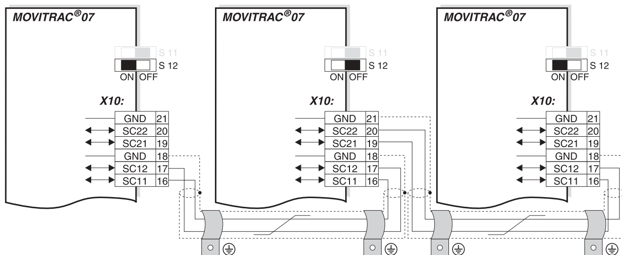
Figure 79: MOVITRAC® 07 system bus connection
