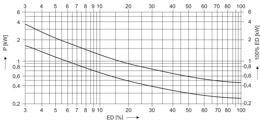
Figure 50: Flat-type 230 V
