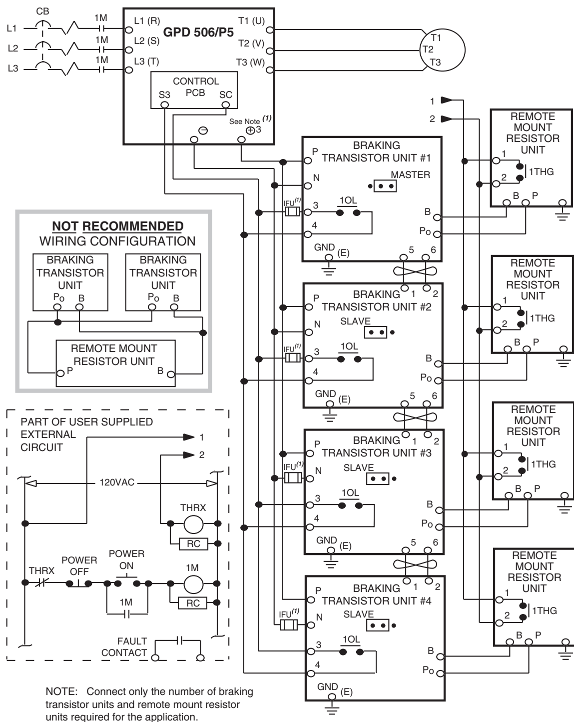
Figure A6-5. Wiring Multiple Braking Transistor Units and Remote Mount Resistor Units to Drive (GPD506V-B506 and -B675 [CIMR-P5M42200F and 43000F], and CIMR-P5M50451F thru 51600F).
