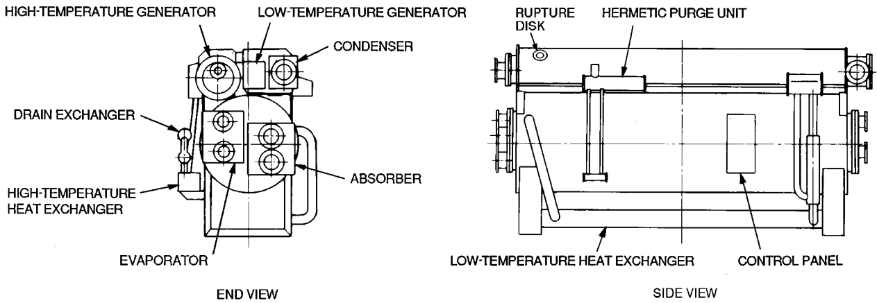
Fig. 3 — 16JT810-880 Machine Components, External Schematic (Typical)
