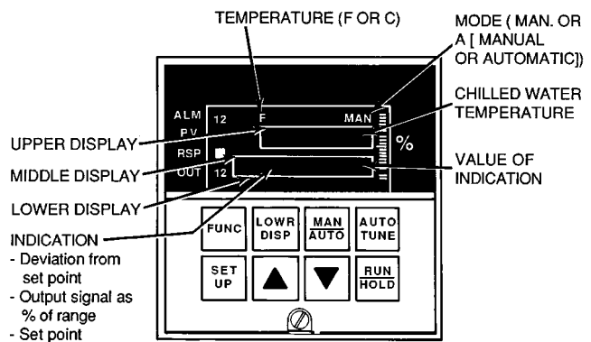
Fig. 21 — Operator Interface
