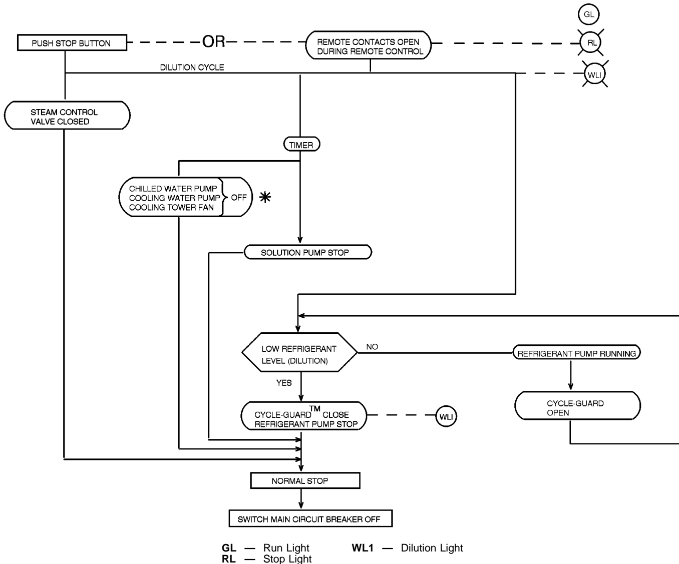
Fig. 15 — Typical Control Sequence, Normal Stop
