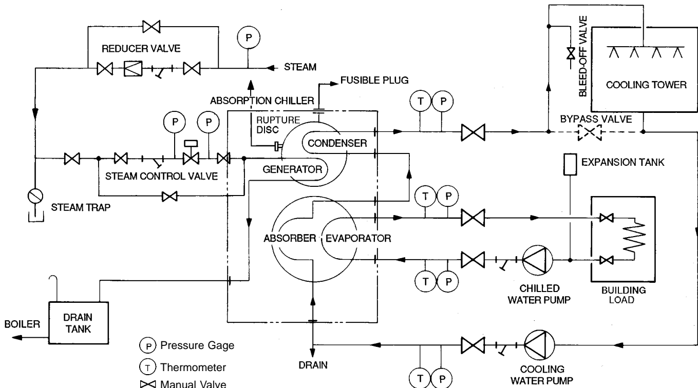
Fig. 19 — Typical Piping
