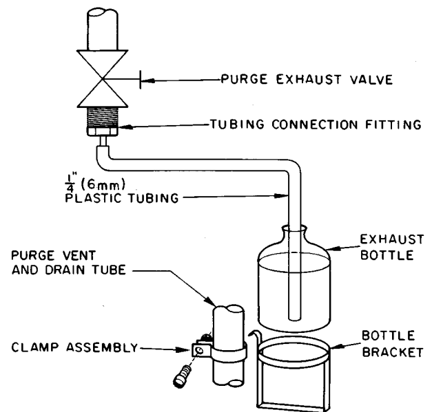
Fig. 25 — Purge Exhaust Assembly
