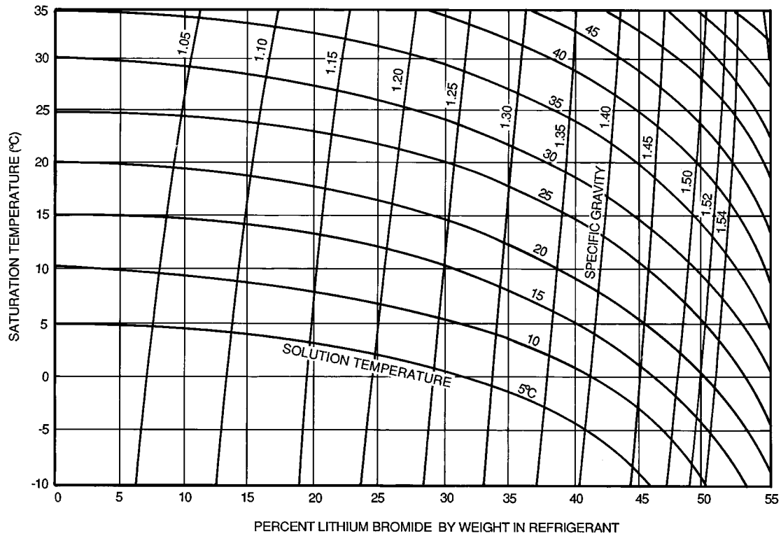
Fig. 26B — Equilibrium Diagram for Lithium Bromide in Refrigerant (C)
