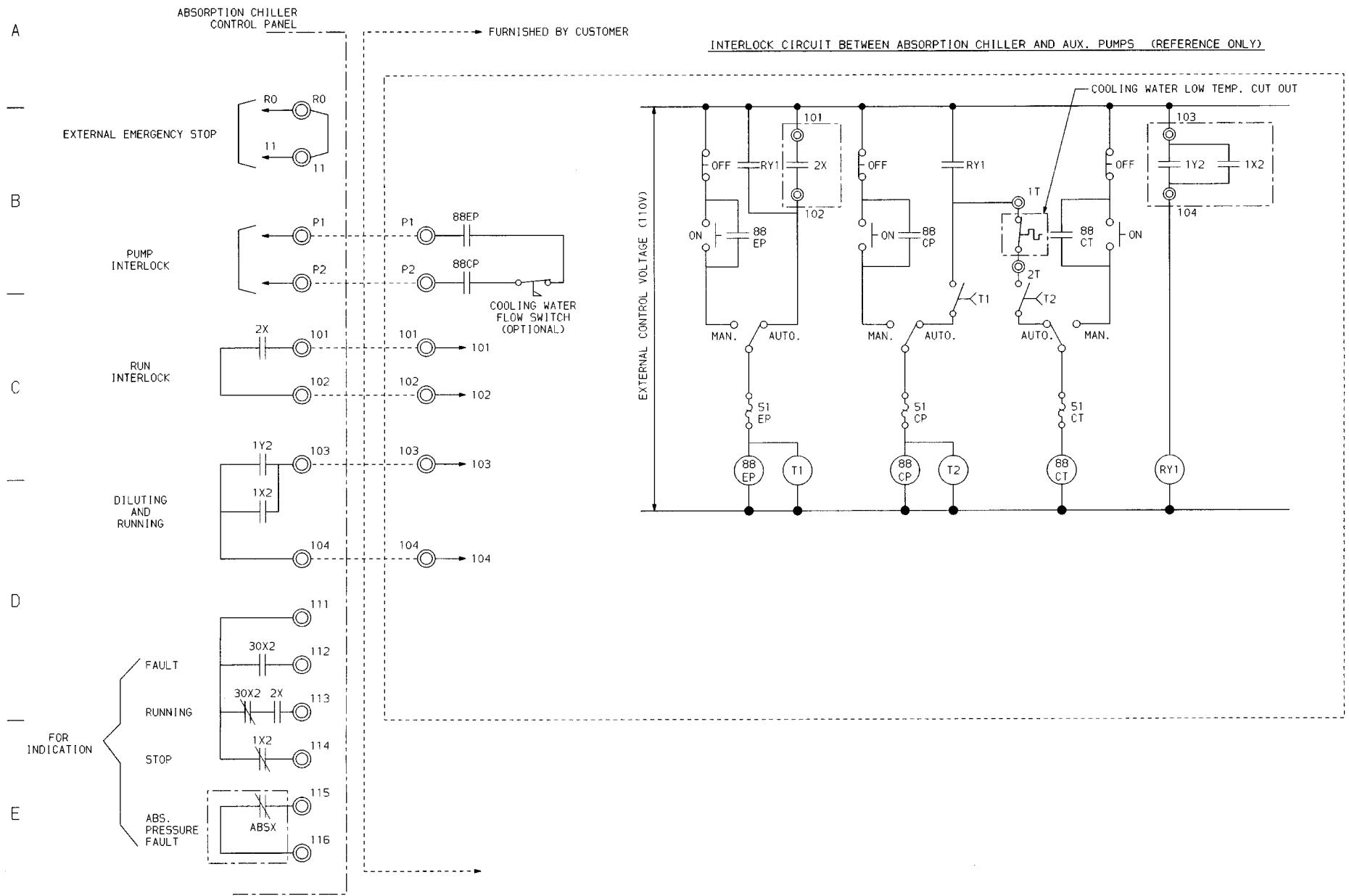
Fig. 11 — Typical Control Wiring
