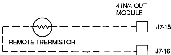
Fig. 29 - Remote Reset from Space or Outdoor-Air Temperature
