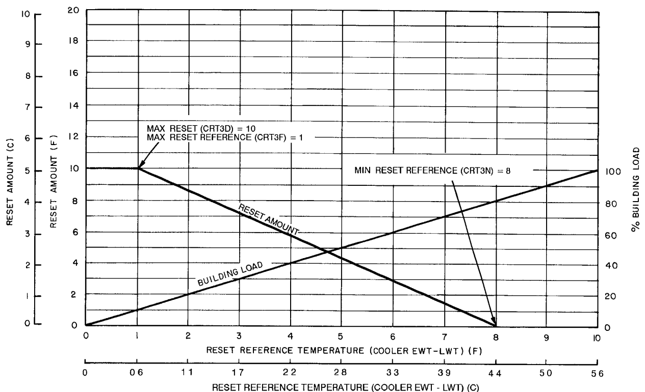
Fig. 5 — Cooling Return Water Reset
