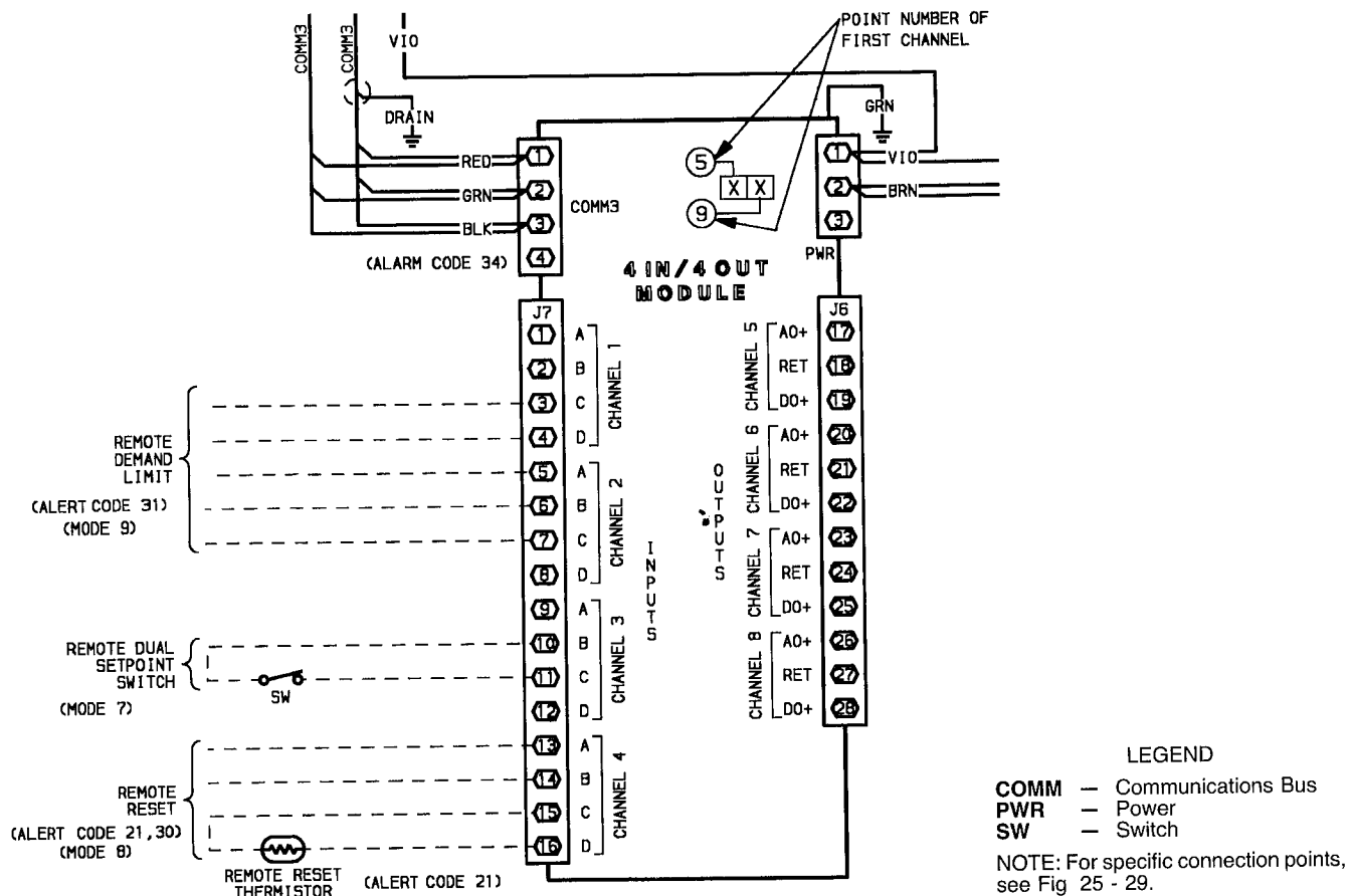
Fig. 6 – Cooling External Temperature Reset
