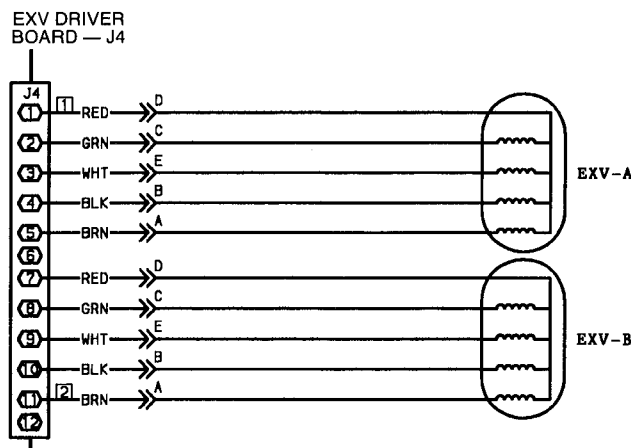
EXV — Electronic Expansion Valve
