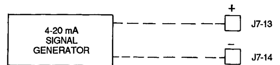
Fig. 31 - Remote Reset from 4-20 mA Signal (Internally Powered)
