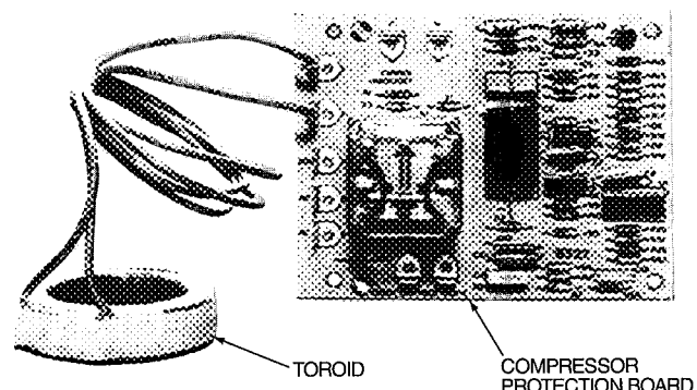
Fig. 2 — Compressor Protection Control Module
