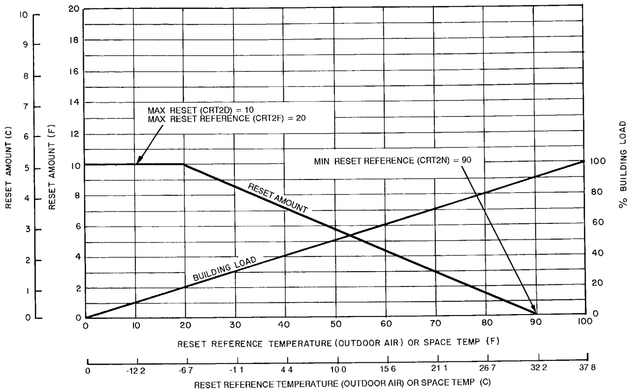
Fig. 6 – Cooling External Temperature Reset
