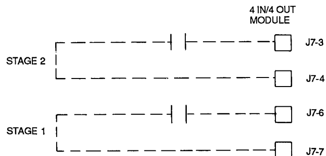
Fig. 26 — Demand Limit — Two External Switch Inputs
