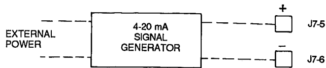
Fig. 27 - Demand Limit - 4-20 mA Signal (Externally Powered)
