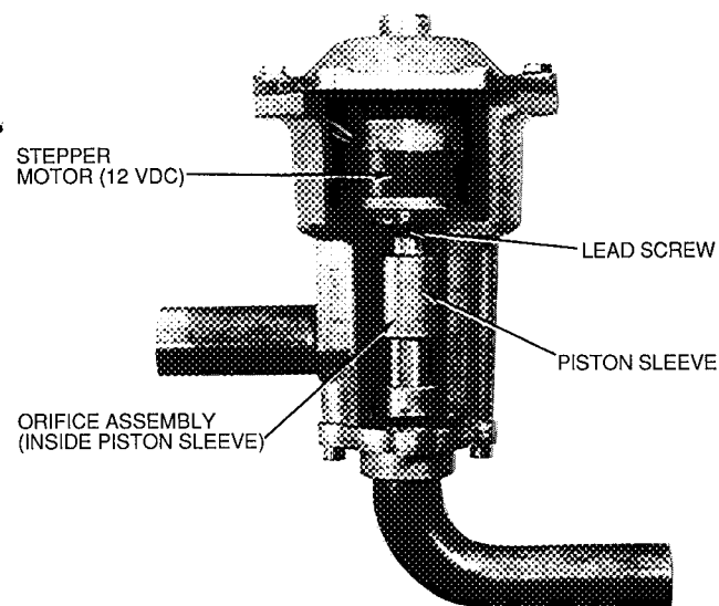
Fig. 12 — Electronic Expansion Valve (EXV)
