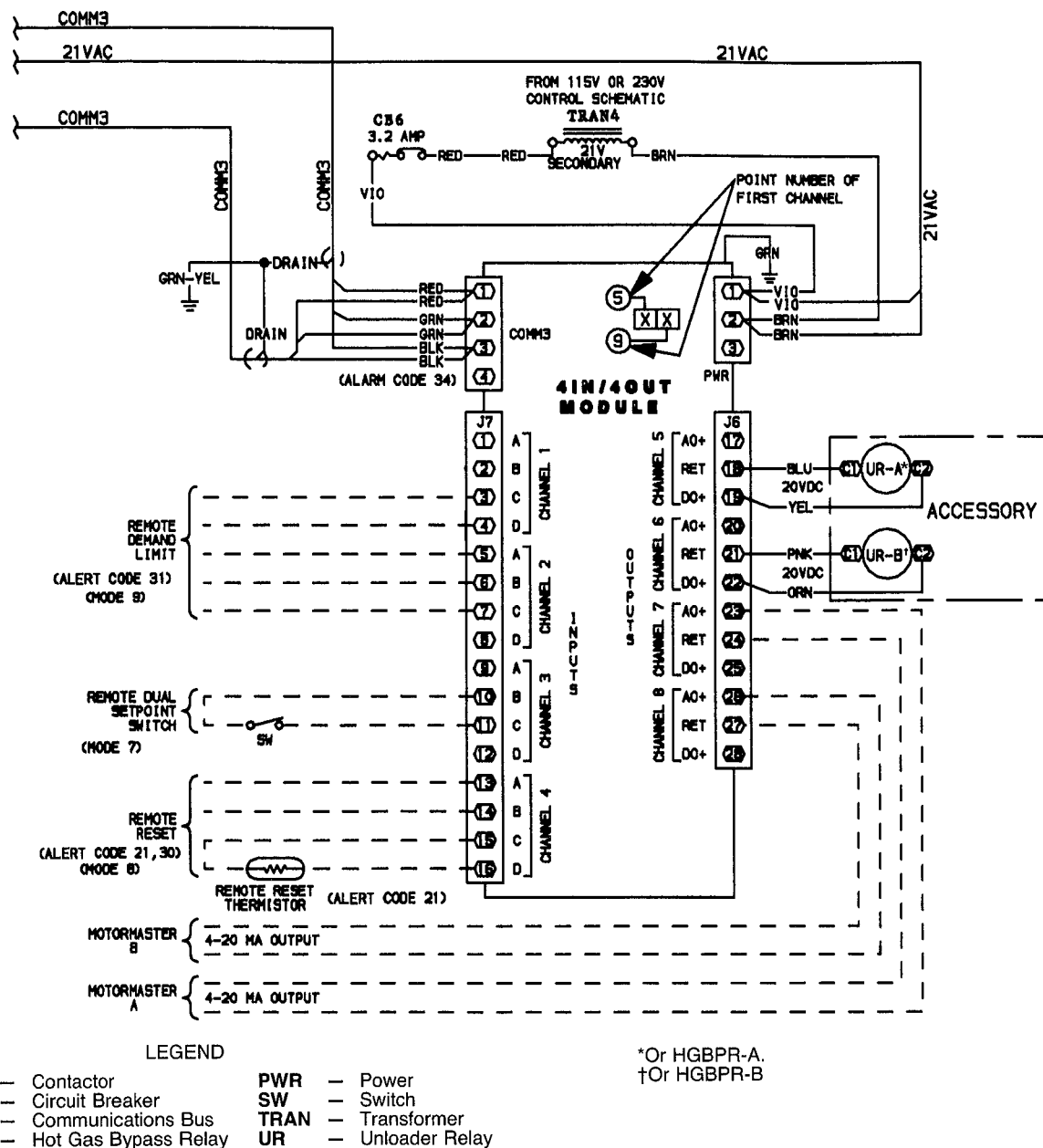
Fig. 25 — Accessory Unloader Control Wiring, 130 (50 Hz), 150-210, and Associated Modular Units
