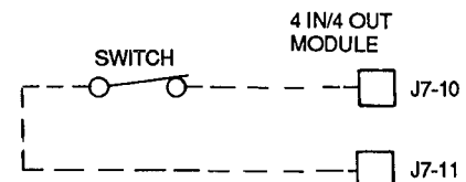
Fig. 33 - Remote Dual Set Point Control
