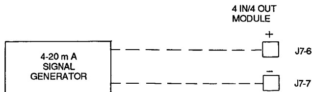
Fig. 28 - Demand Limit - 4-20 mA Signal (Internally Powered)
