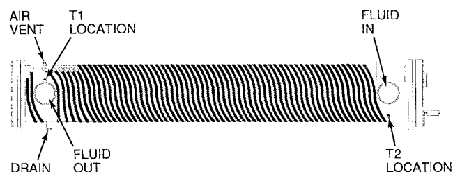
Fig. 31 — Cooler Heater Cables
