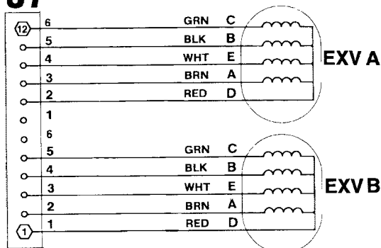
Fig. 28 — Processor Board Connections
