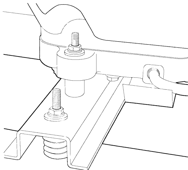
Fig. 9 — Compressor Mounting Bolts
