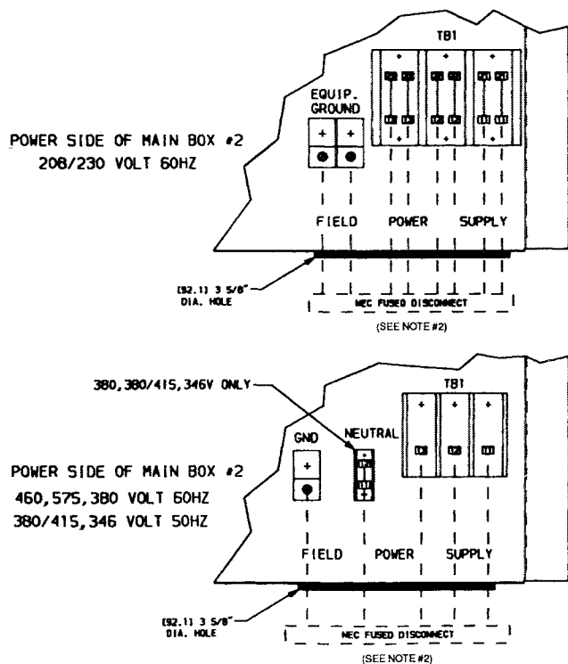
Fig. 13 — Field Power Wiring; Unit Sizes 230B-315B
