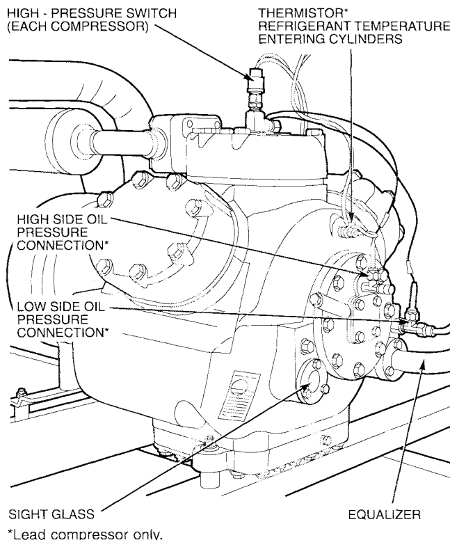
Fig. 16 — Compressor Connections (Lead Compressor Shown)
