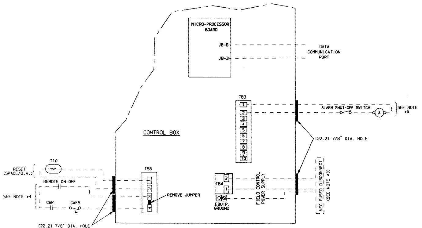
Fig. 15 — Field Control Power Wiring; Unit Sizes 130-210, 230A-315A, 330A/B-420A/B
