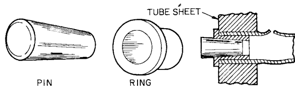
Fig. 23 — Elliott Tube Plug
