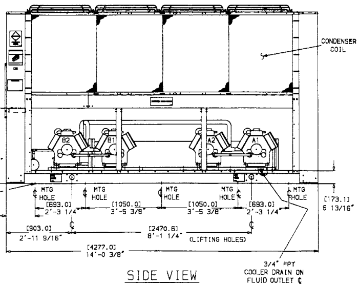
Fig. 2 —Dimensions; 30GT100,110,270B-315B
