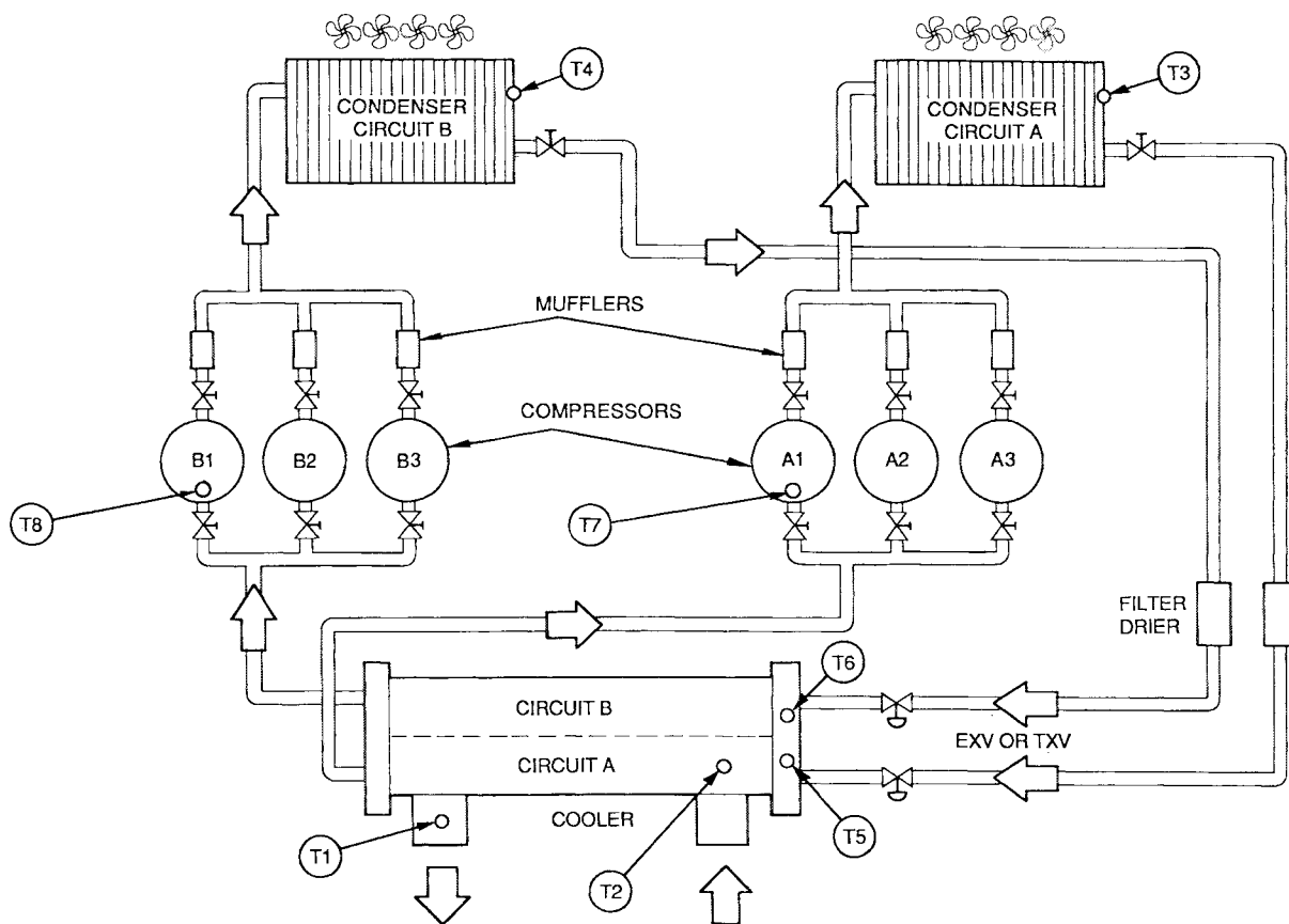
Fig. 19 — Typical Thermistor Locations
