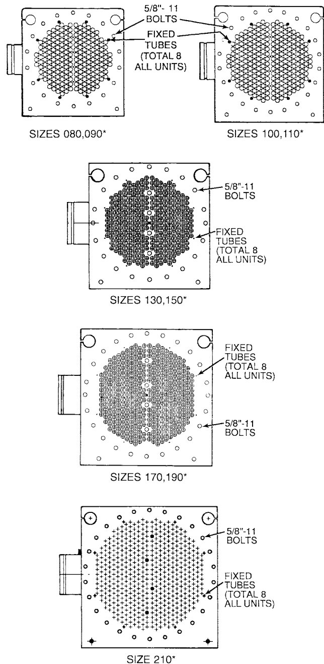
Fig. 22 — Typical Tube Sheets, Cover Off (Non-Removable Tubes)
