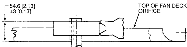
Fig. 26 — Condenser Fan Adjustment, Units with High Static Fan Option
