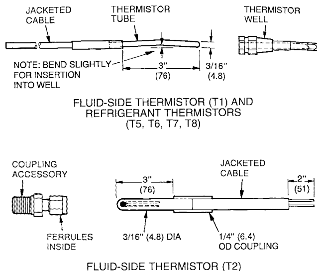
Fig. 29 — Thermistors
