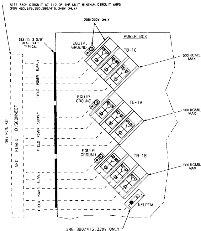
Fig. 11 — Field Power Wiring; Unit Sizes 130-210
