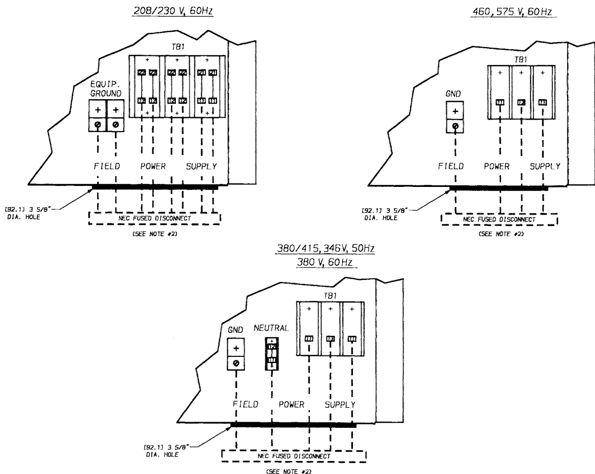
Fig. 10 — Field Power Wiring; Unit Sizes 080-110
