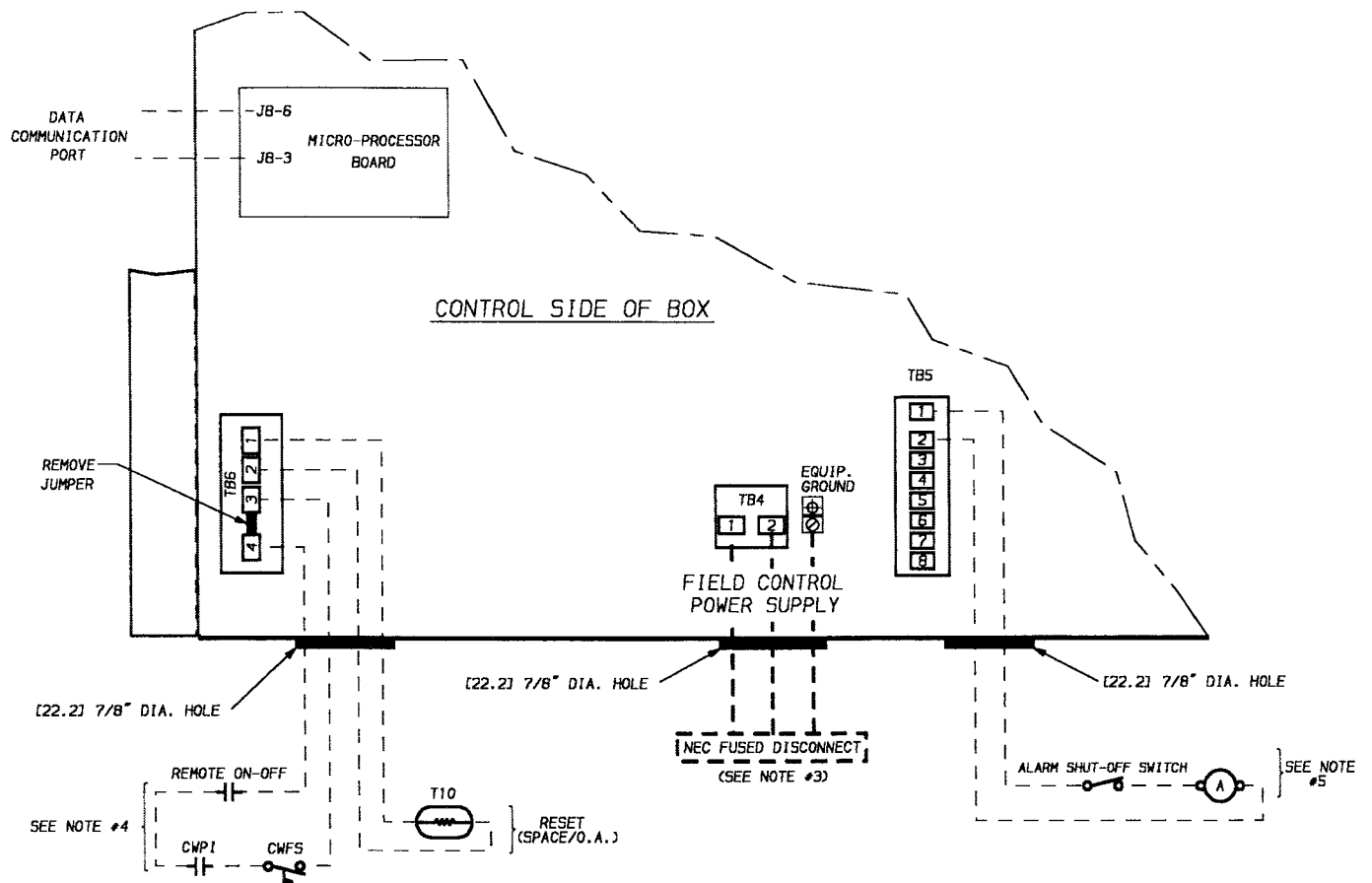
Fig. 14 — Field Control Power Wiring; Unit Sizes 080-110, 230B-315B
