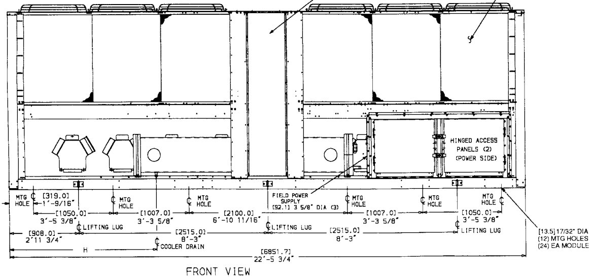
Fig. 4 — Dimensions; 30GT190,210,290A,315A,360A/B (60 Hz), 390A/B, 420A/B
