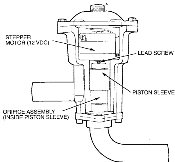
Fig. 27 — Electronic Expansion Valve (EXV)
