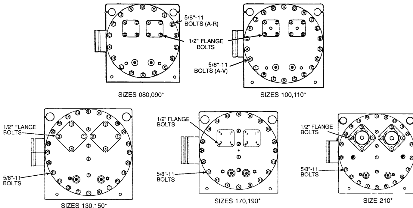
Fig. 24 — Cooler Head Bolt Tightening Sequence (Typical Tube Sheet)
