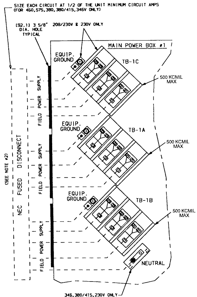
Fig. 12 — Field Power Wiring; Unit Sizes 230A-315A, 330A/B-420A/B
