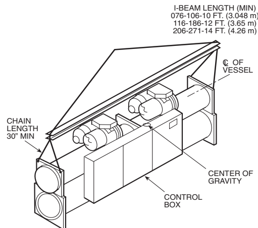
Fig. 12 — Unit Rigging (Size 076-186 Shown, Larger Sizes Similar)
