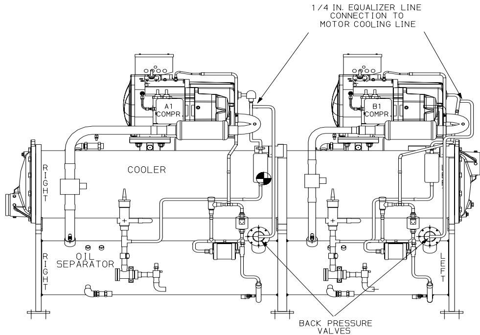
Fig. 18A — 30HXA Units Back Pressure Valve Equalizer Line Connection (076-186 Sizes Shown)
