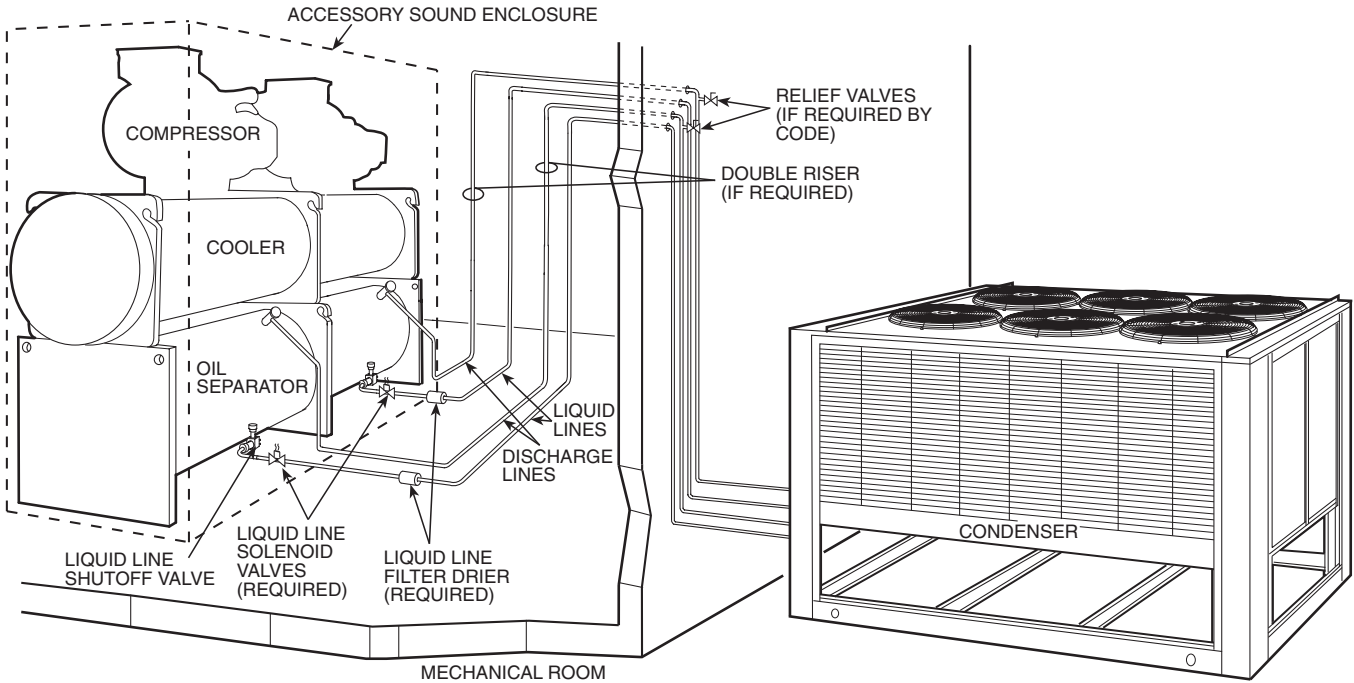
Fig. 14A — Typical 30HXA Refrigerant Piping to Remote Condenser (076-186 Sizes Shown)
