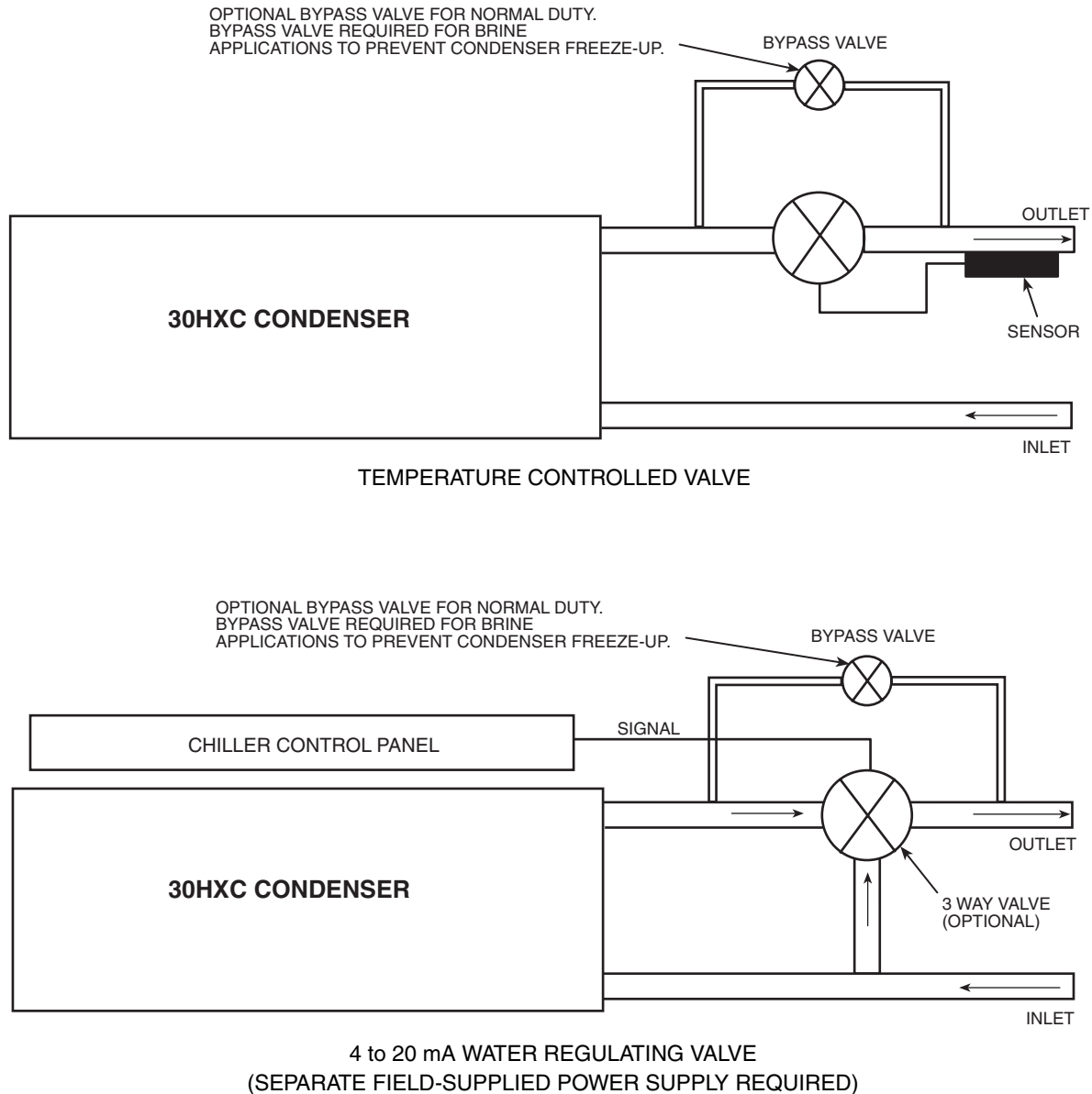
Fig. 19 — Condenser Temperature Regulating Valve Installation
