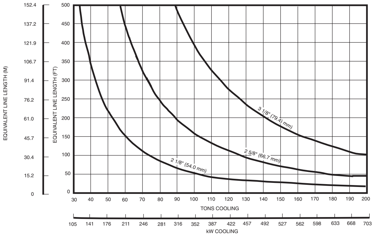
Fig. 15 — R-134a Liquid Line Sizing, 30HXA Units
