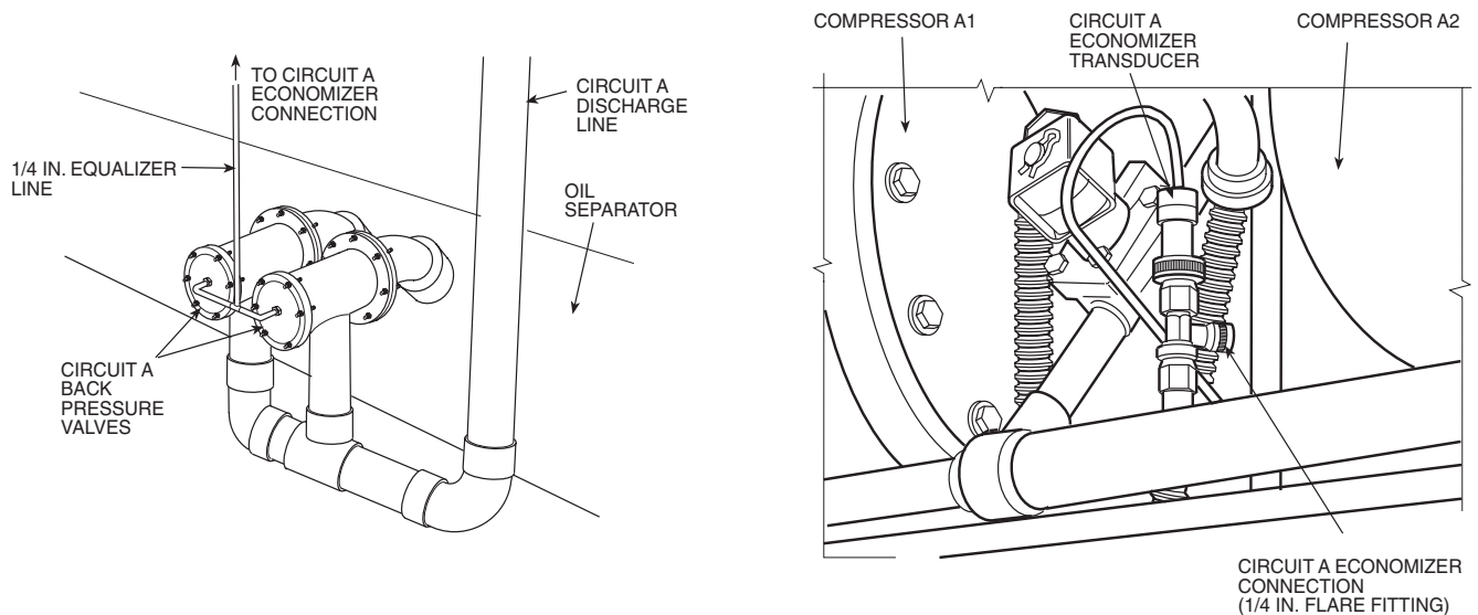
Fig. 18B — 30HXA206-271 Back Pressure Valve Equalizer Line Connection (Circuit A)
