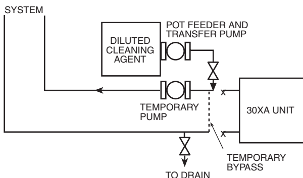
Fig. 27 — Typical Set Up for Cleaning Process
