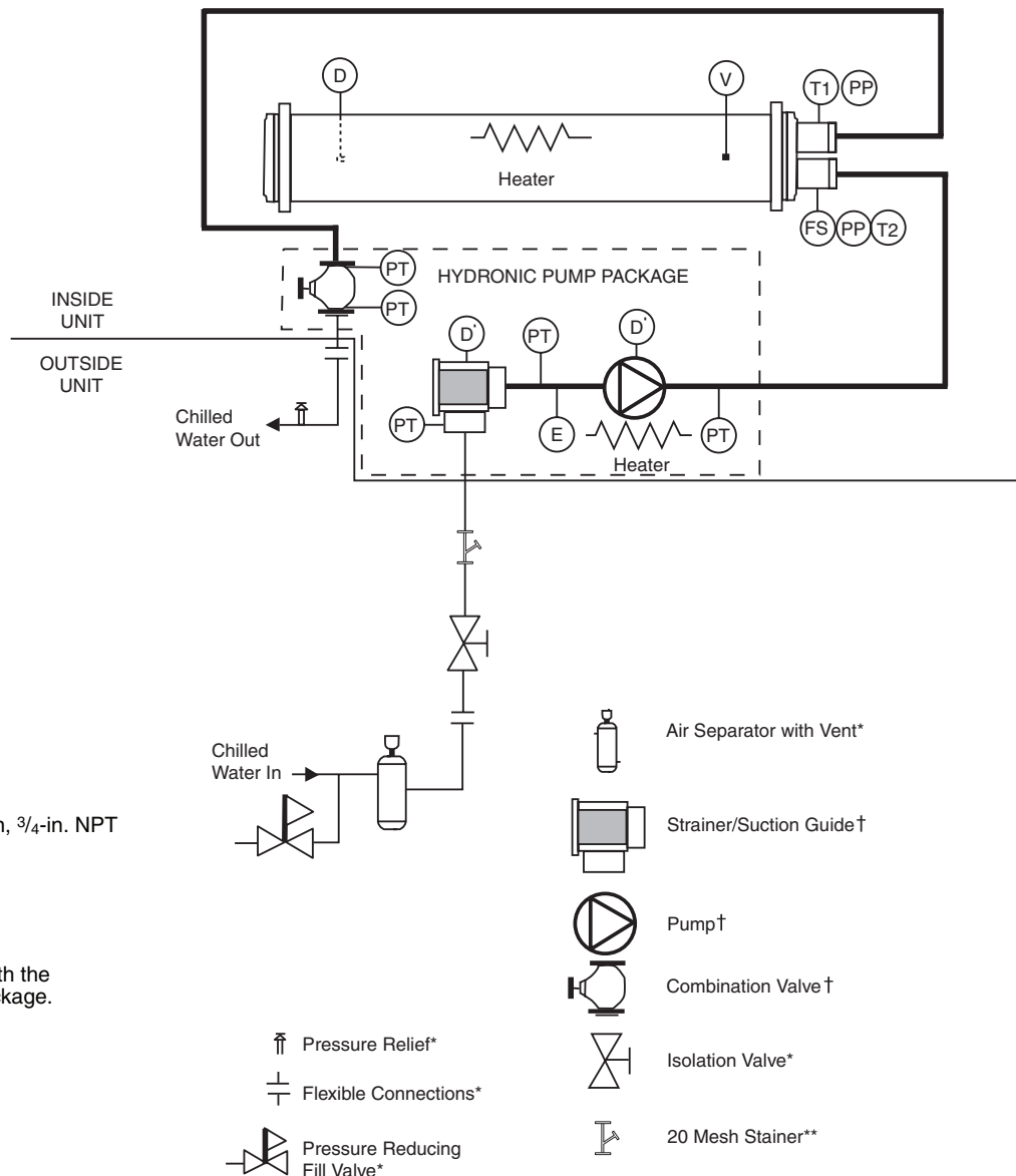
Fig. 20 — Typical Piping Diagram on 30XA Units with Hydronic Package — Single Pump
