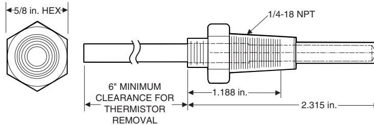
Fig. 35 — Dual Leaving Water Thermistor Well (Part No. OOPPG00008000A)
