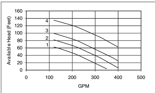
Fig. 29 — 30XA090-160 Single Pump Envelope Curves
