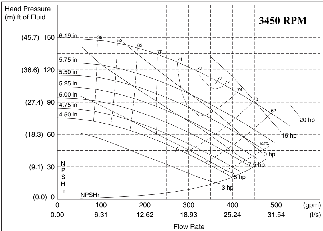
Fig. 31 — Pump Curve I for Hydronic Package Single Pump (Fresh Water)
