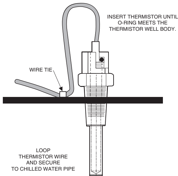
Fig. 36 — Dual Leaving Water Thermistor (Part No. OOPPG00008105A)
