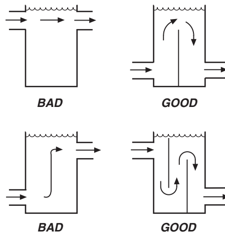
Fig. 23 — Tank Baffling
