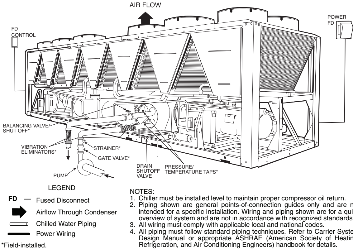
Fig. 15A — 30XA Typical Piping and Wiring (Units without Hydronic Package)
