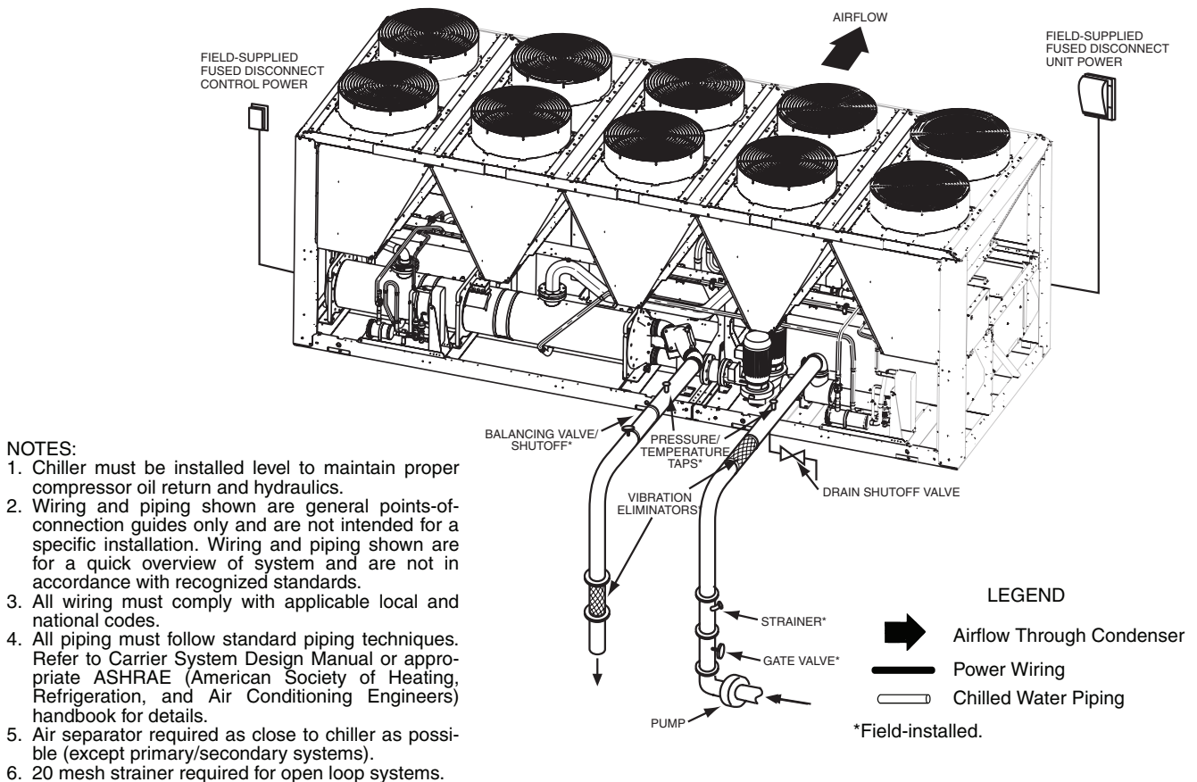
Fig. 15B — 30XA Typical Piping and Wiring (Units with Hydronic Package)
