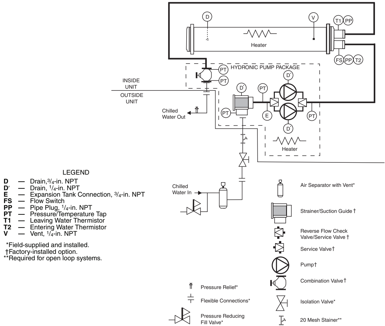
Fig. 21 — Typical Piping Diagram on 30XA Units with Hydronic Package — Dual Pumps
