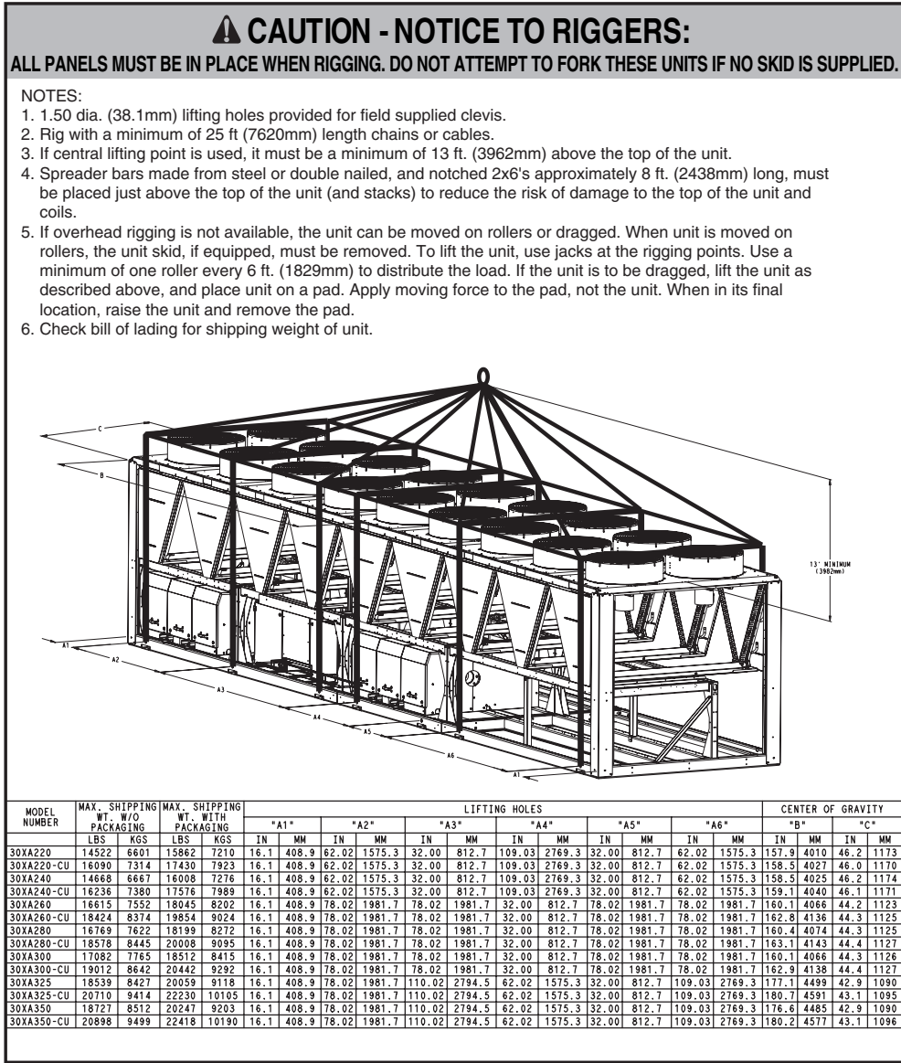
Fig. 13 — Unit Rigging Label Detail 30XA220-350
