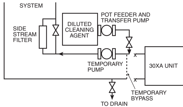
Fig. 28 — Cleaning Using a Side Stream Filter
