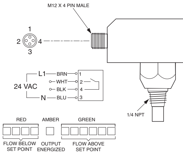
Fig. 38 — Chilled Water Flow Switch LED Display
