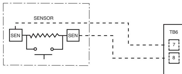
Fig. 28 — Typical Remote Space Temperature Sensor (33ZCT55SPT) Wiring
