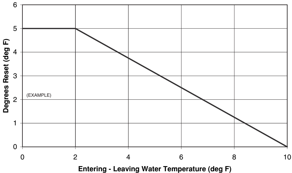
Entering - Leaving Water Temperature (deg F) Fig. 16 — Water Temperature Difference (Delta T) Reset
