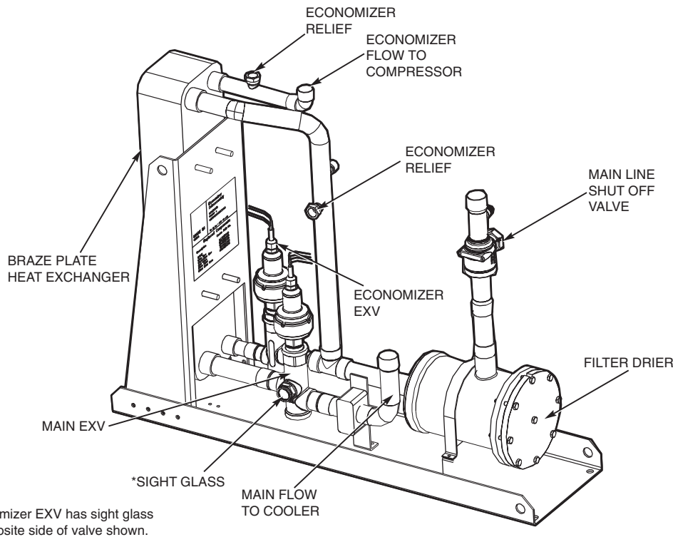
Fig. 30 — Economizer Assembly
