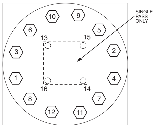
Fig. 37 — Cooler Head Recommended Bolt Torque Sequence
