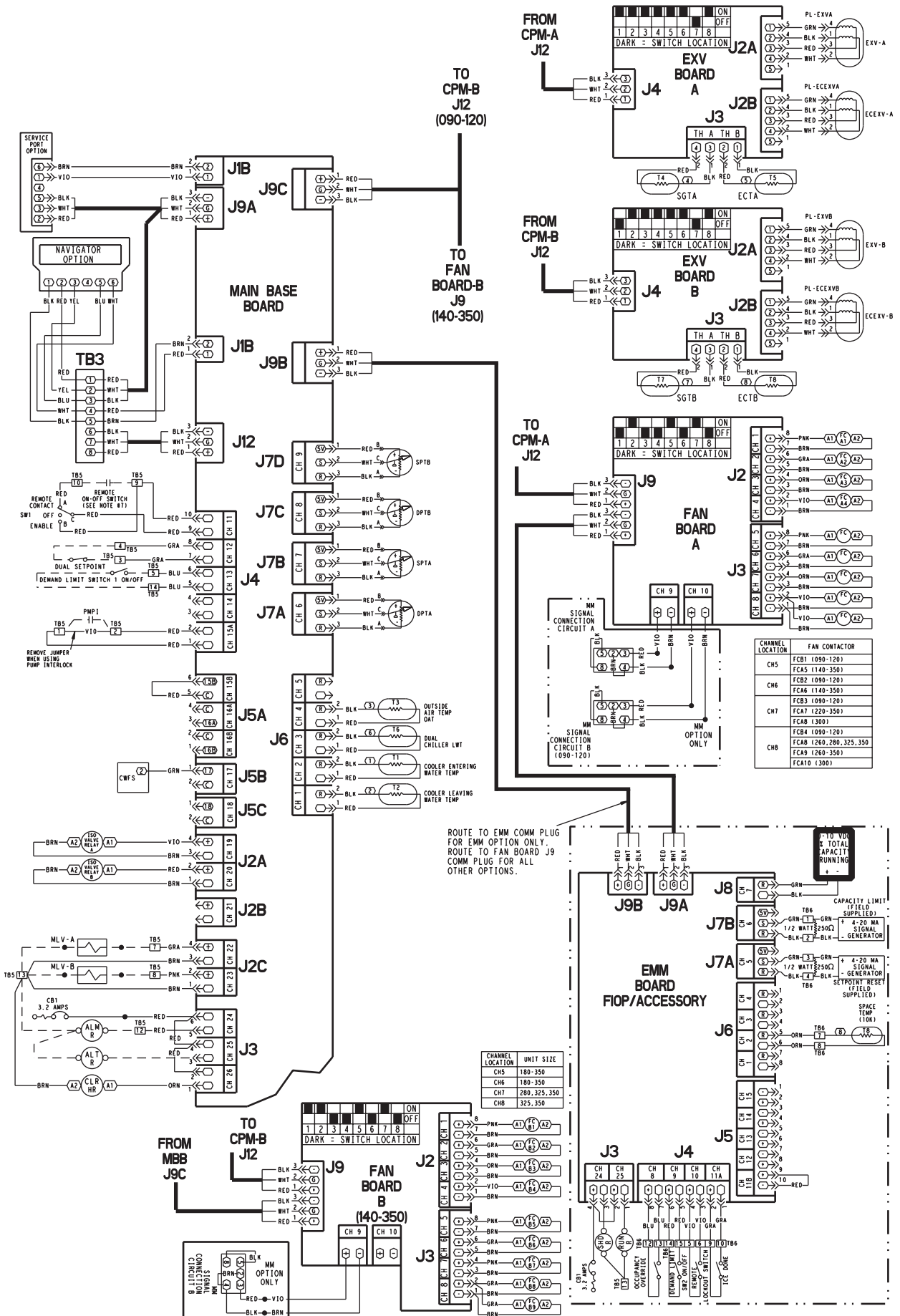
Fig. 43 — 30XA090-350 Low Voltage Control Schematic
