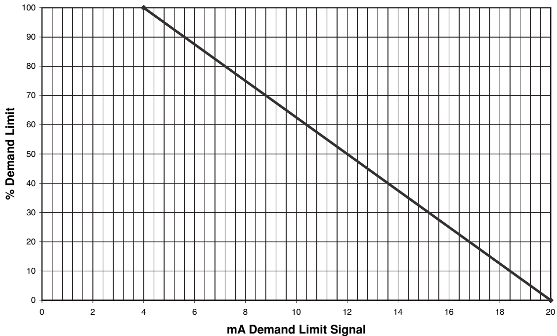
Fig. 21 — Demand Limit
