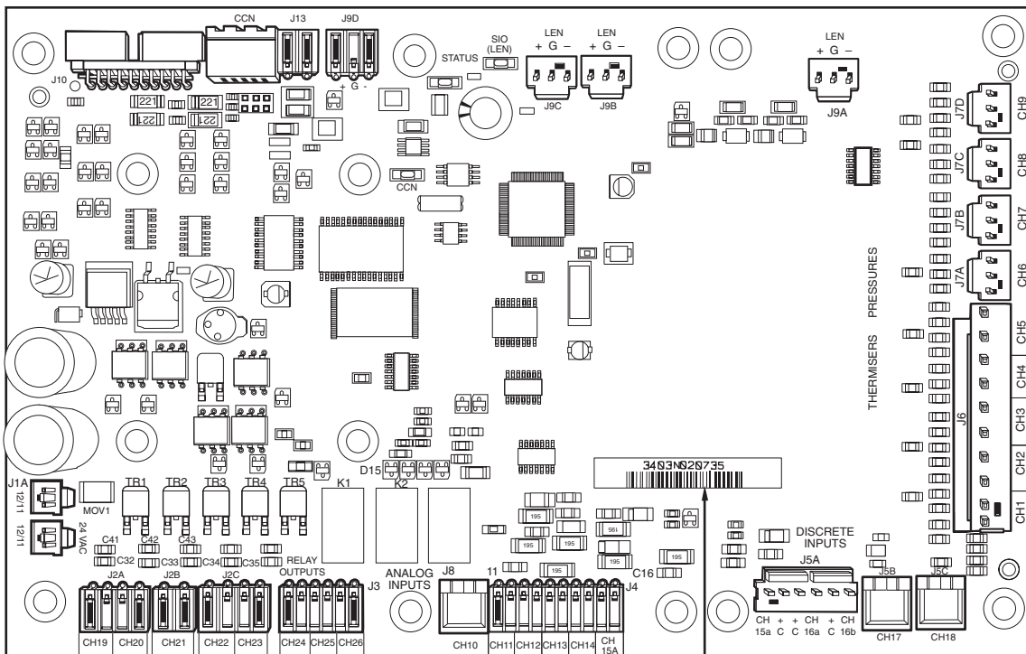
Fig. 2 — Main Base Board
