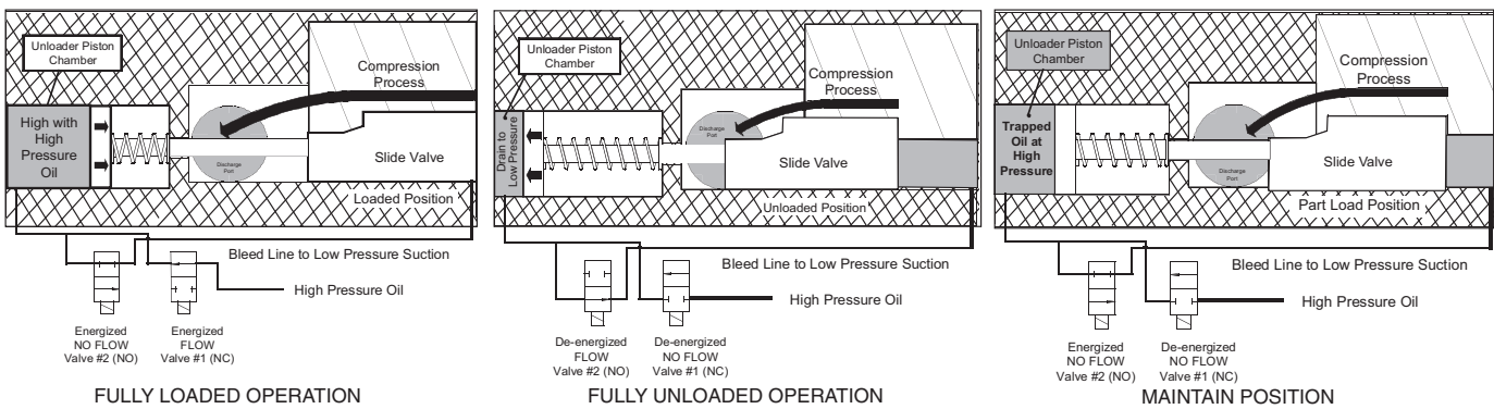
Fig. 33 — Typical 06T Compressor
