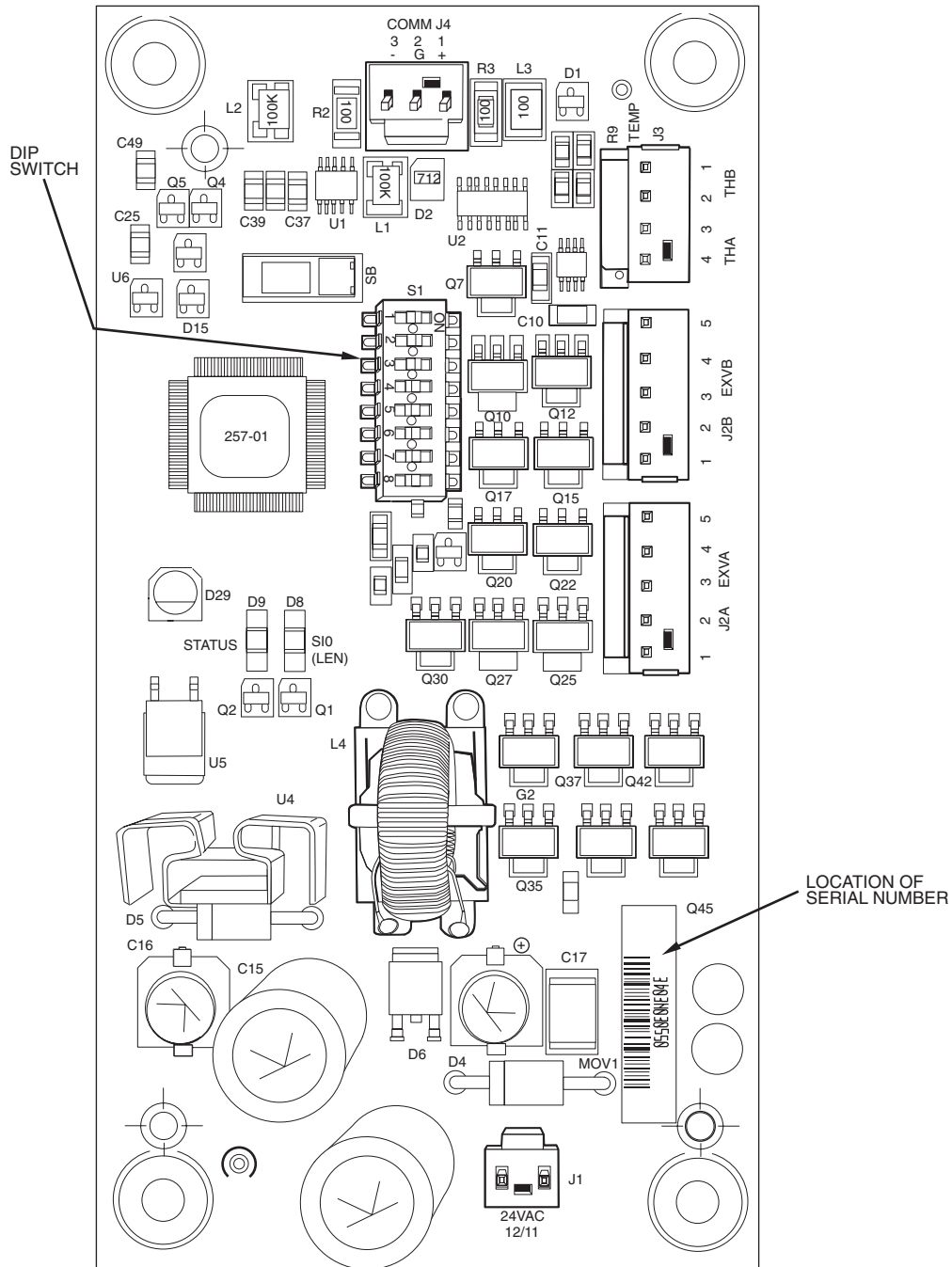
Fig. 4 — EXV Board
