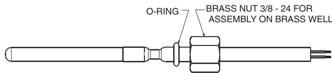
Fig. 26 — 5K Thermistor (Sensor 00PG00008105A, Connector: HY06AM016)
