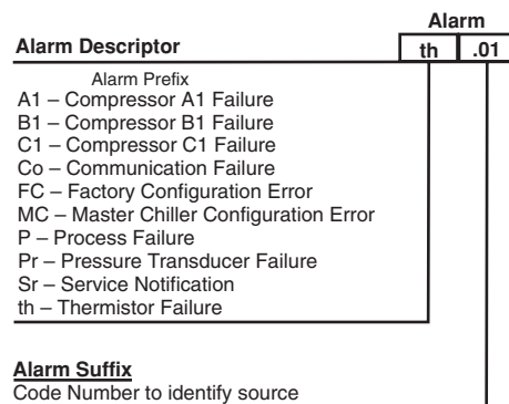
Fig. 41 — Alarm Description
