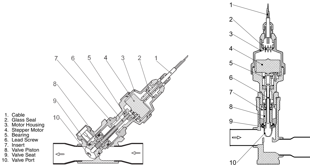
Fig. 31 — Cutaway Views of the Electronic Expansion Valve
