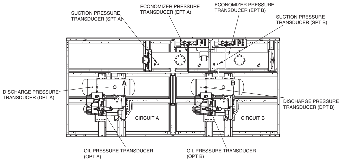
Fig. 29 — Transducer Locations
