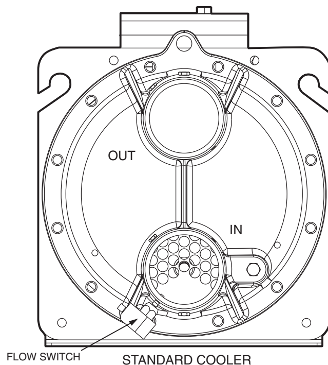
Fig. 39 — Flow Switch
