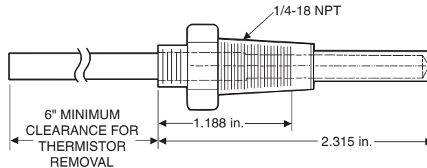
Fig. 27 — Dual Leaving Water Thermistor Well (00PPG0000800A)
