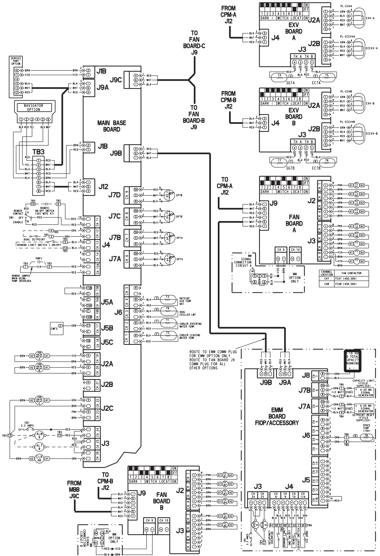
Fig. 44 — 30XA400-500 Low Voltage Control Schematic
