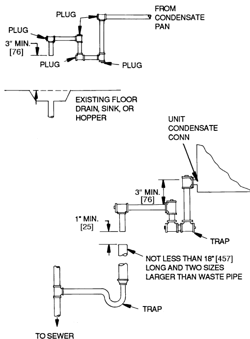
Fig. 13 — Condensate Drains
