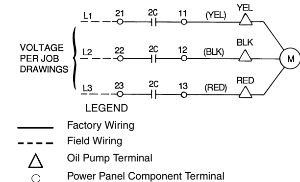
Fig. 36 — Oil Pump Wiring
