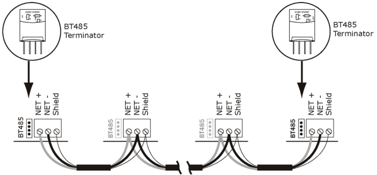
Fig. 40 — Network Wiring
