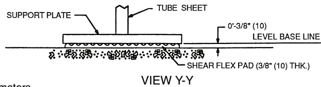
Fig. 13 — Standard Isolation
