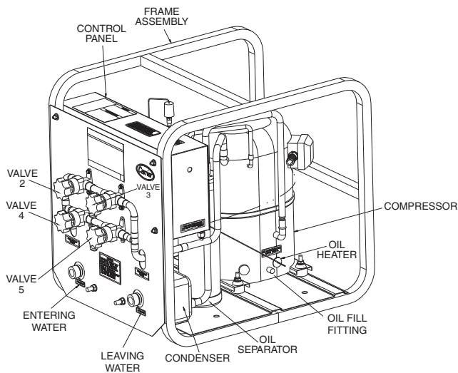
Fig. 24 — Pumpout Unit
