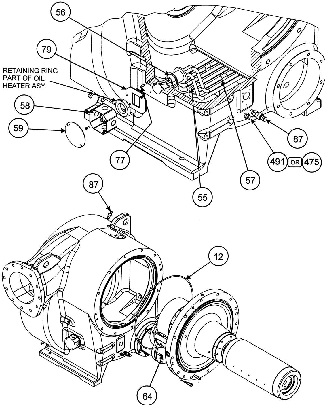
Frame #4 Compressor With Split Ring Diffuser
