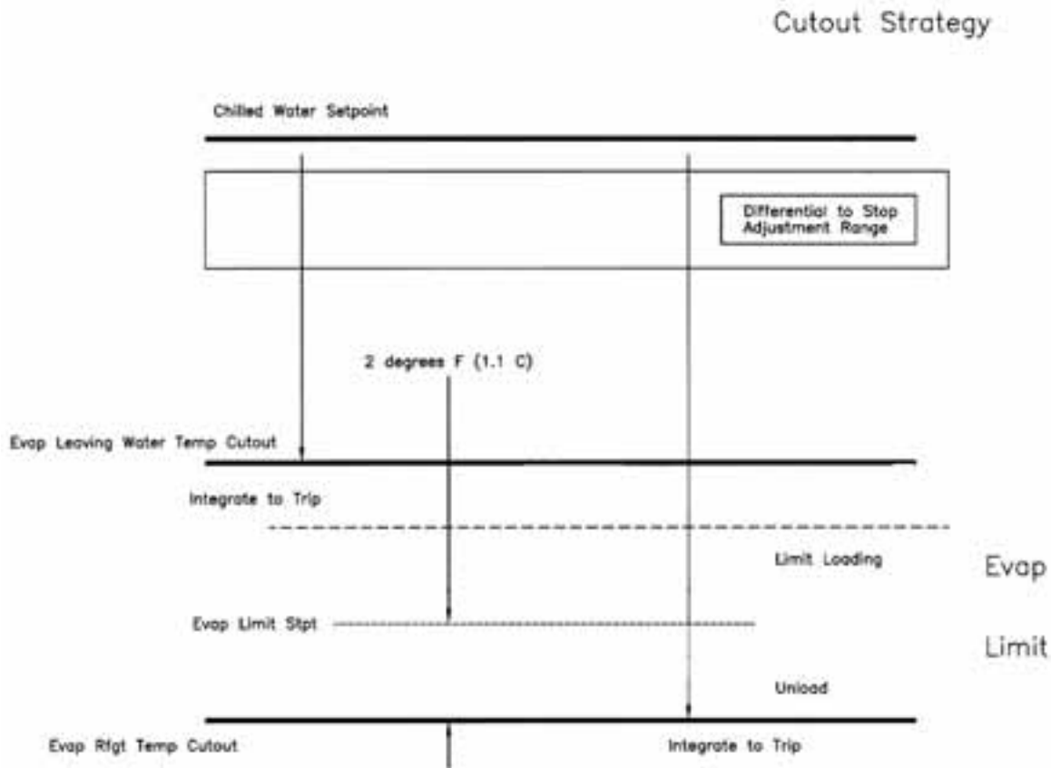
Figure 27. Cutout strategy
