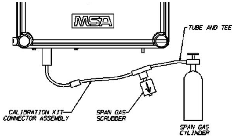
Figure 4-6. Span Calibration
