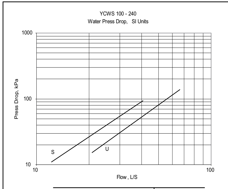
FIGURE 4 - CONDENSER WATER PRESSURE DROP CURVES (SI)
