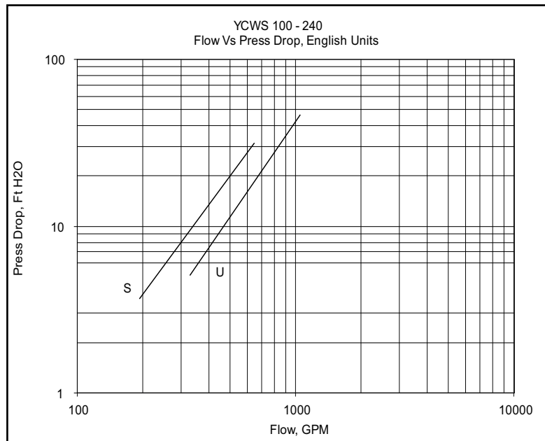
FIGURE 3 - CONDENSER WATER PRESSURE DROP CURVES (ENGLISH)
