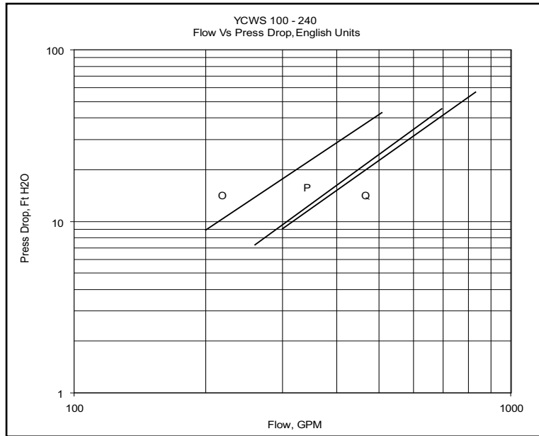
FIGURE 1 - COOLER WATER PRESSURE DROP CURVES (ENGLISH)
