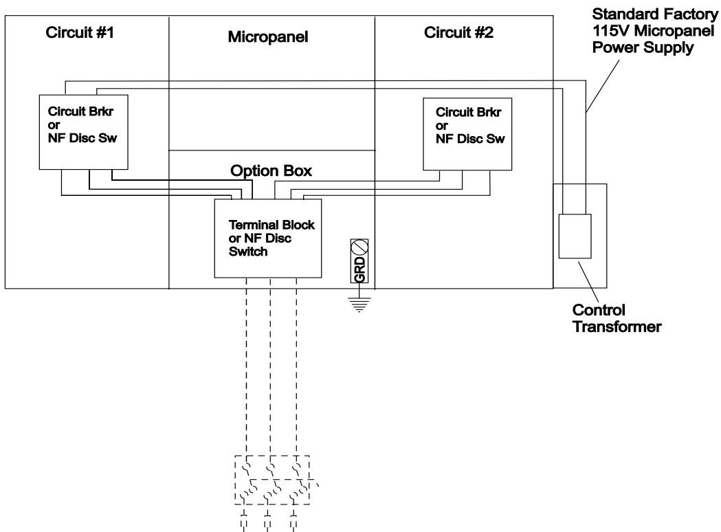
FIGURE 10 - SINGLE POINT POWER SUPPLY WITH INTERNAL CIRCUIT BREAKER OR NON-FUSED DISCONNECT SWITCH
