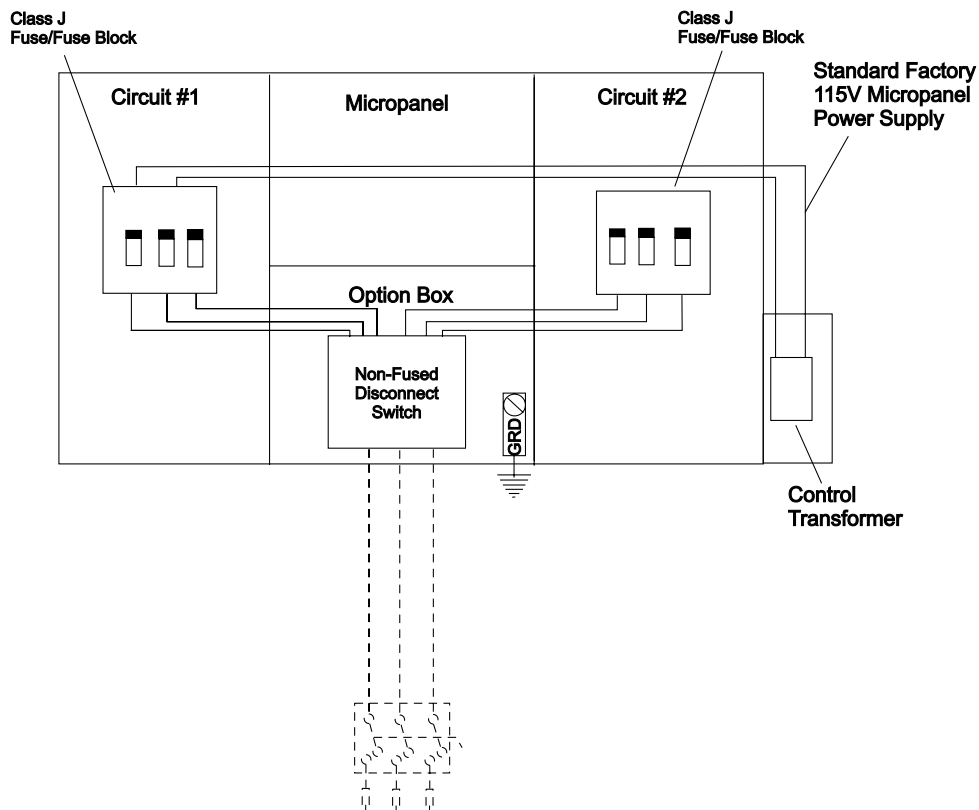
FIGURE 11 - OPTIONAL SINGLE POINT POWER SUPPLY WITH INTERNAL CLASS J FUSES/BLOCK
