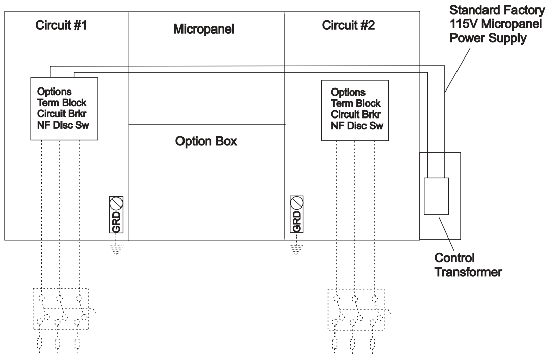
FIG. 13 – MULTI POINT POWER SUPPLY CONNECTION - STANDARD UNIT
