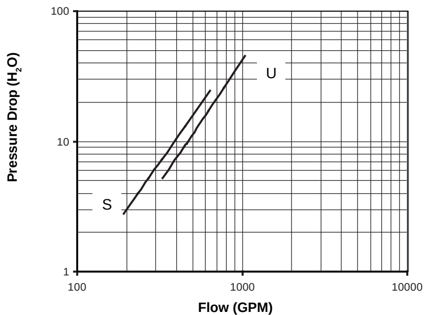
FIG. 23 – COOLER WATER PRESSURE DROP CURVES (ENGLISH)
