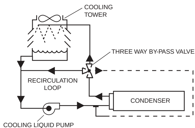
FIG. 11 – TYPICAL CONDENSER FLOW DIAGRAM
