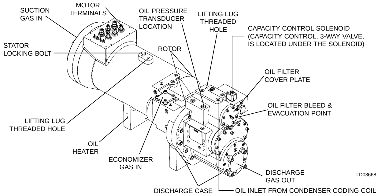
FIG. 2 – SCREW COMPRESSOR
