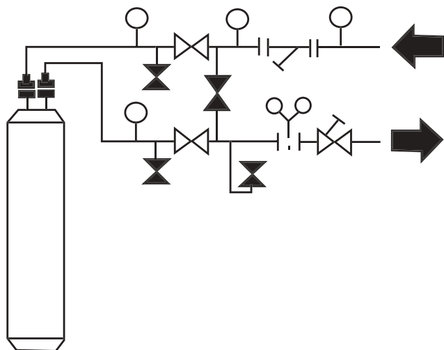
FIG. 9 – COOLER CONNECTIONS
