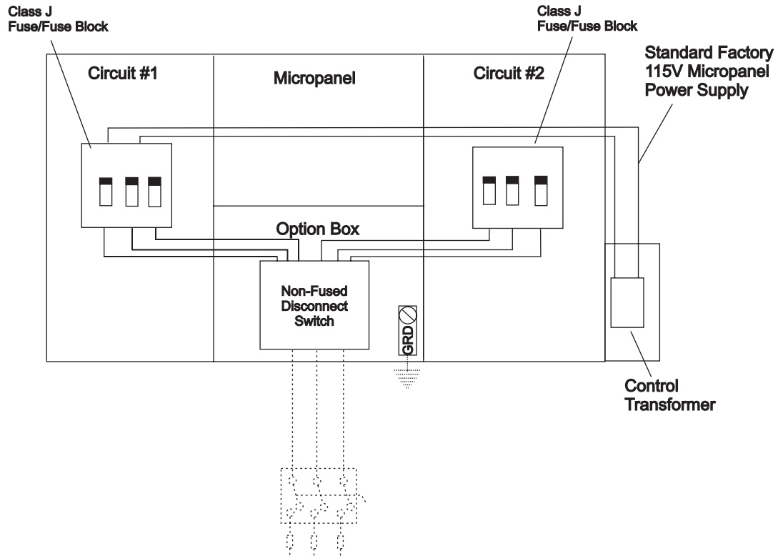
FIG. 15 – OPTIONAL SINGLE-POINT POWER SUPPLY WITH INTERNAL CLASS J FUSES/BLOCK
