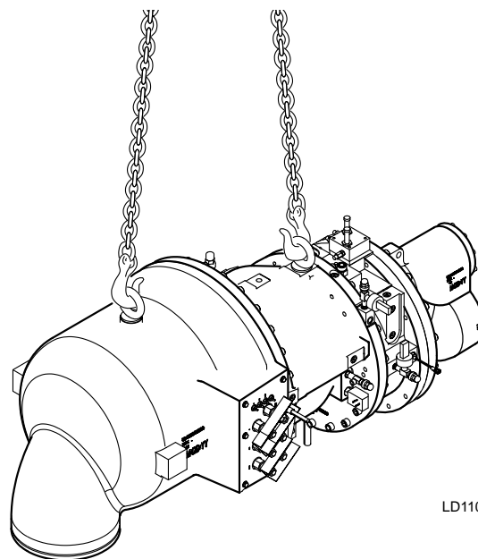
FIG. 6 – RIGGING COMPRESSOR ASSEMBLY
