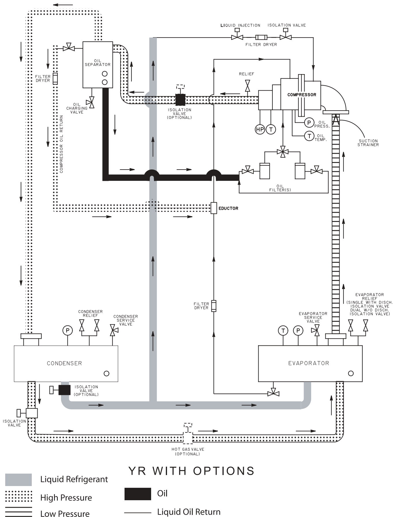
FIG. 16 – YR SCREW CHILLER SYSTEM SCHEMATIC – DESIGN LEVEL “C” (CONT'D)
