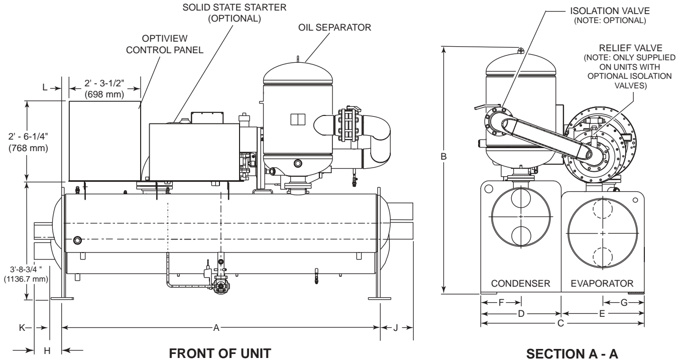
FIG. 2 – COMPRESSORS – EVAPORATOR, CONDENSER AND WATER BOXES DIMENSIONS
