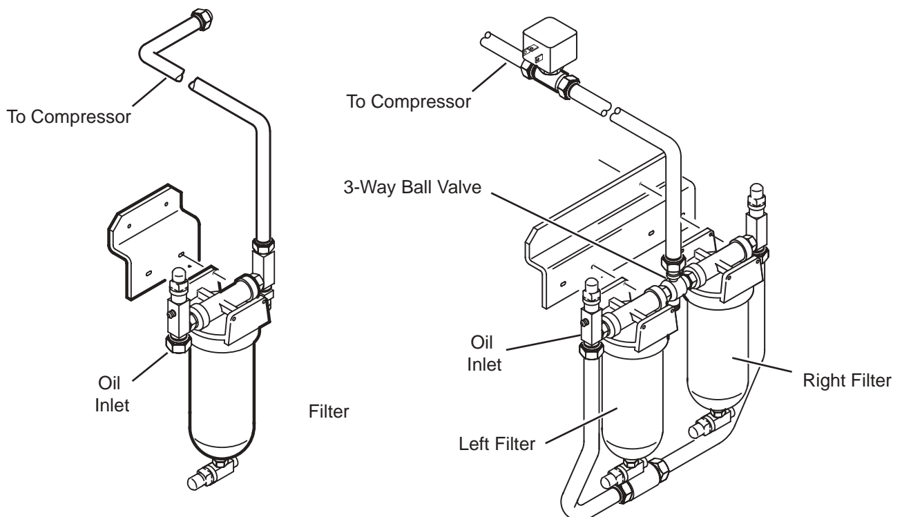
FIG. 21 – OIL FILTERS
