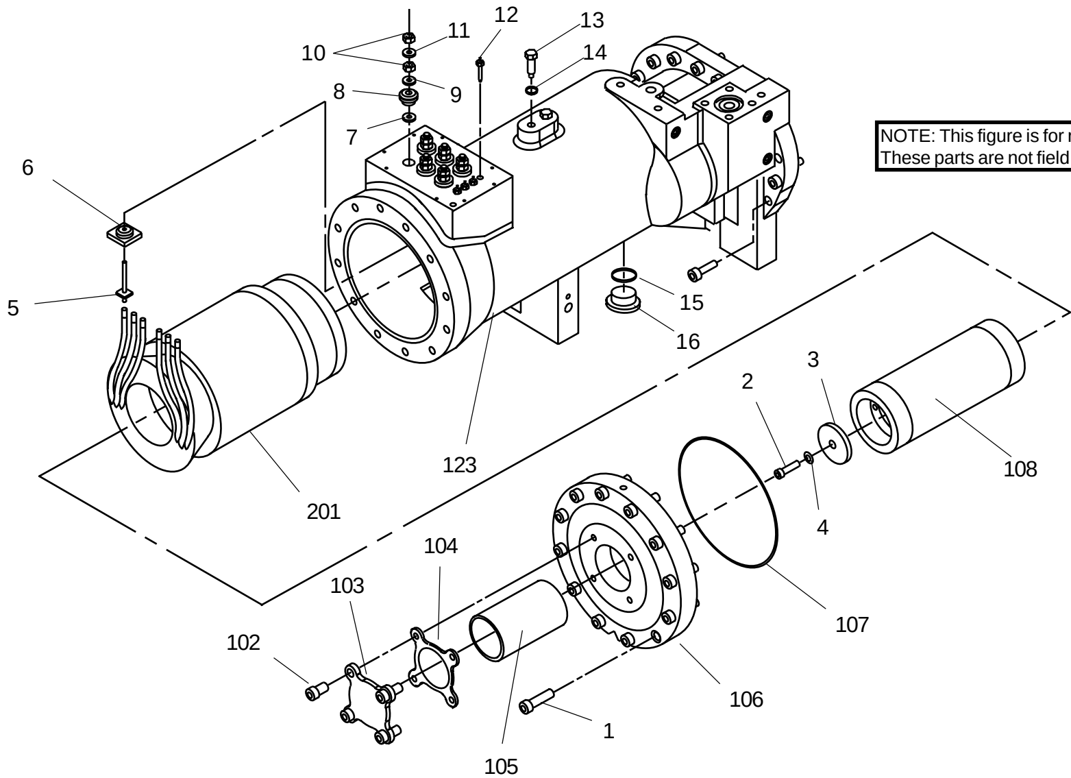
FIG. 9 – COMPRESSOR COMPONENTS - 145 MM COMPRESSOR SHOWN (REF. TABLE 10, PAGE 23 AND 24)
