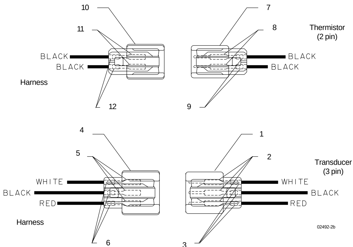
FIG. 17 – TRANSDUCER, TEMPERATURE SENSOR AND WIRE HARNESS CONNECTOR - FIELD REPLACEMENT PART NUMBERS (REF. TABLE 15)
