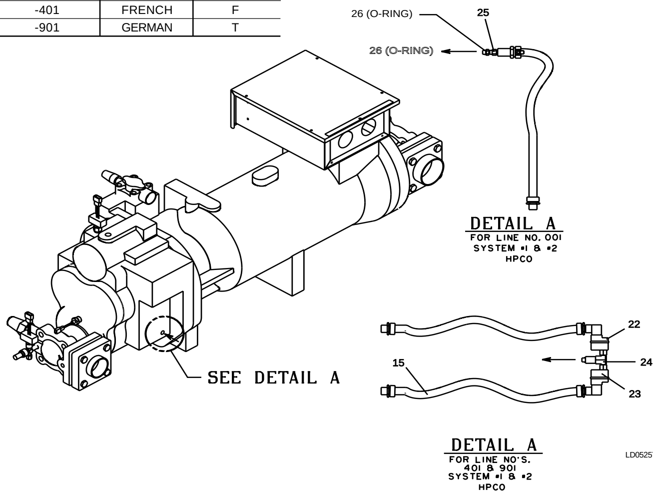
FIG. 6 – RELIEF VALVES AND HP CUTOUT SWITCH (REF. TABLE 7, PAGE 14)
