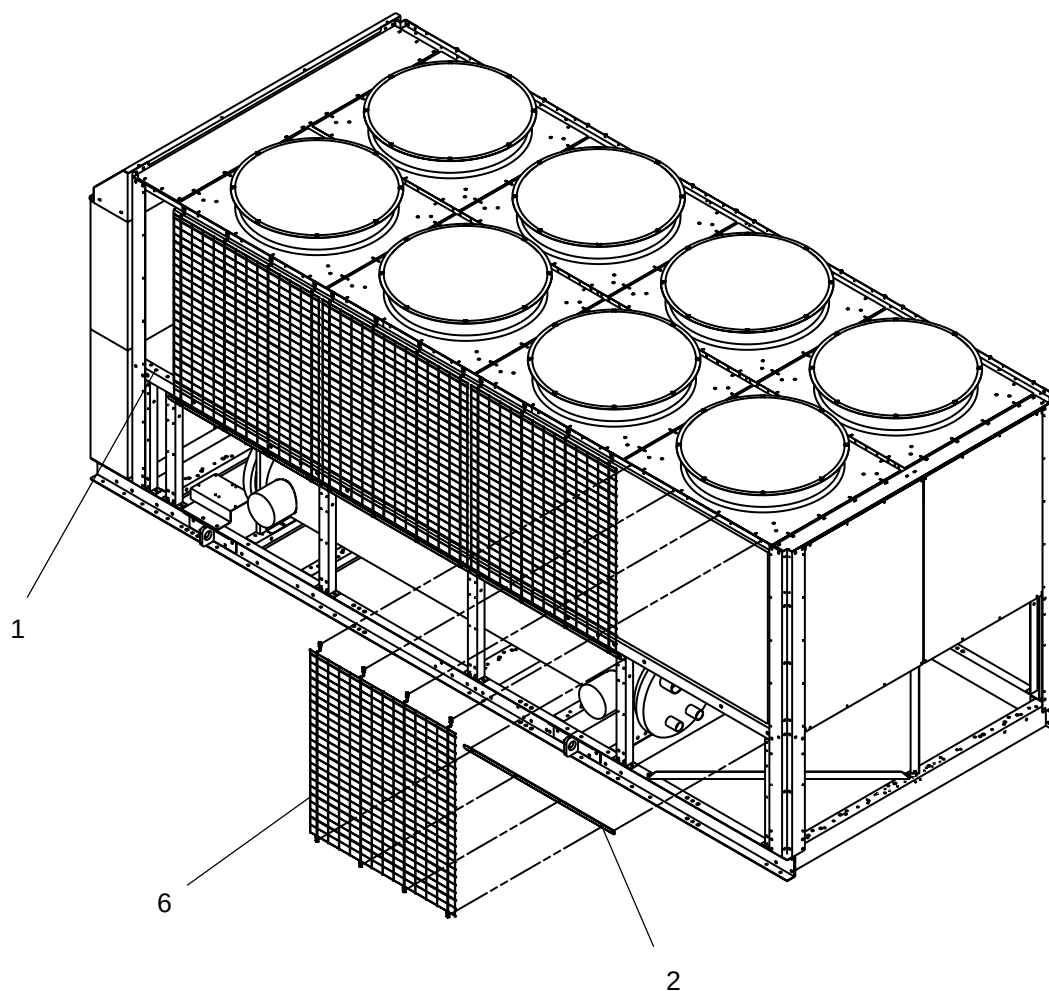
FIG. 26 – WIRE ENCLOSURE - 16'-0" KIT IS SHOWN.
