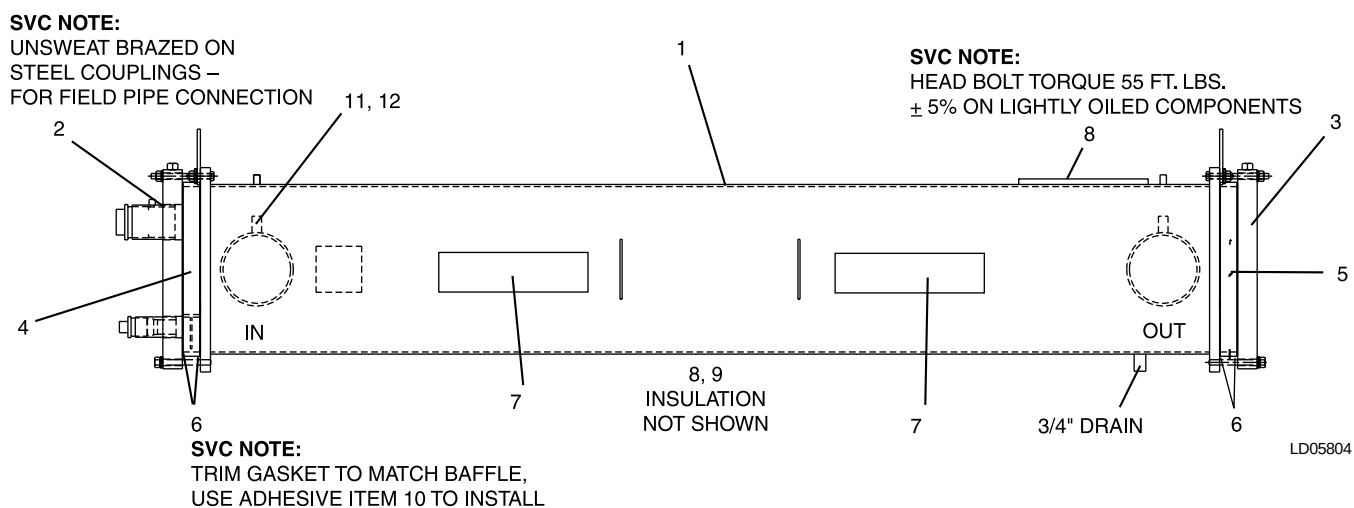
FIG. 1 – EVAPORATOR COMPONENTS
