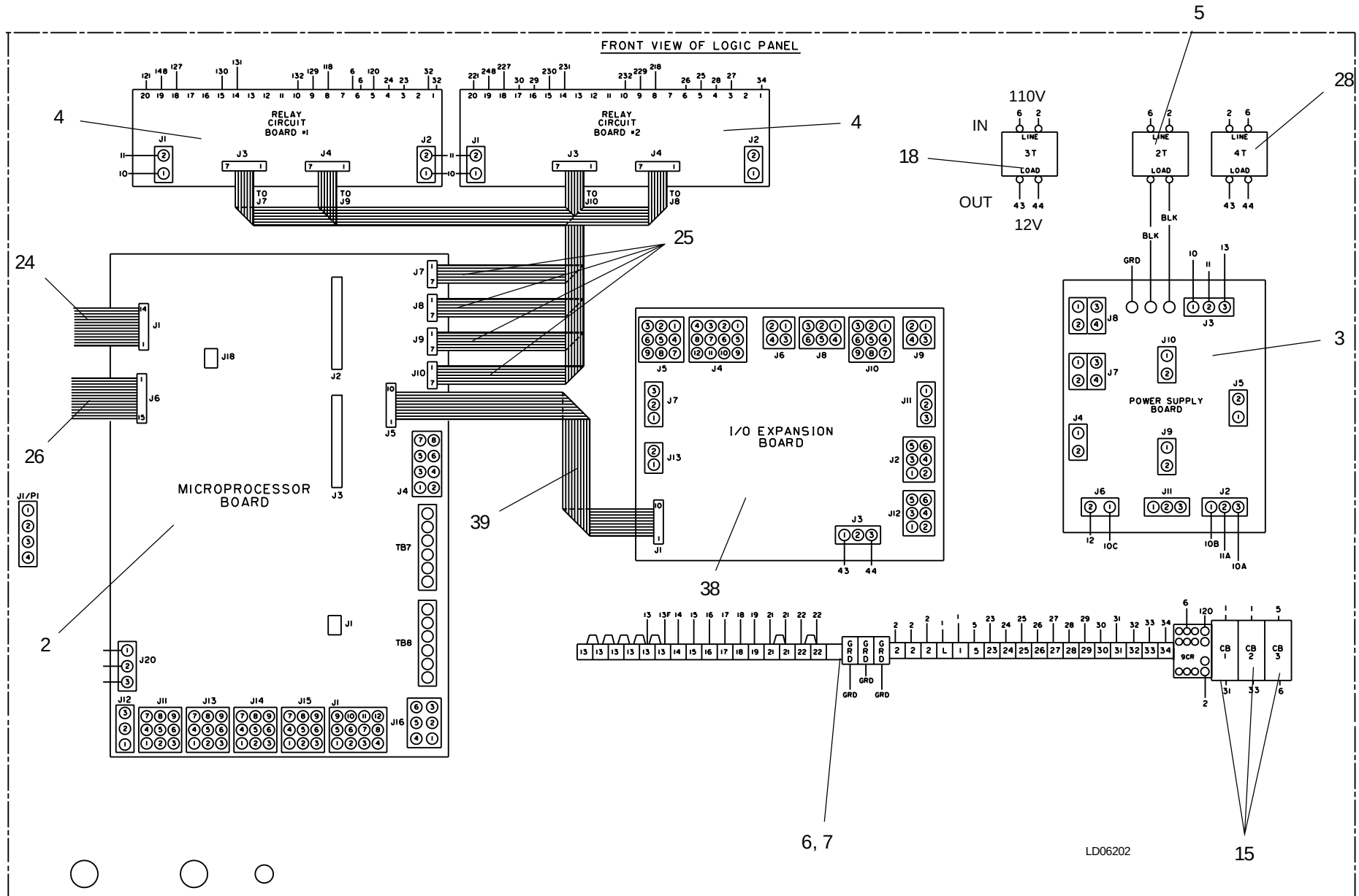
FIG. 13 – MICRO PANEL CONNECTION DIAGRAM (REF. TABLE 13, PAGE 26)
