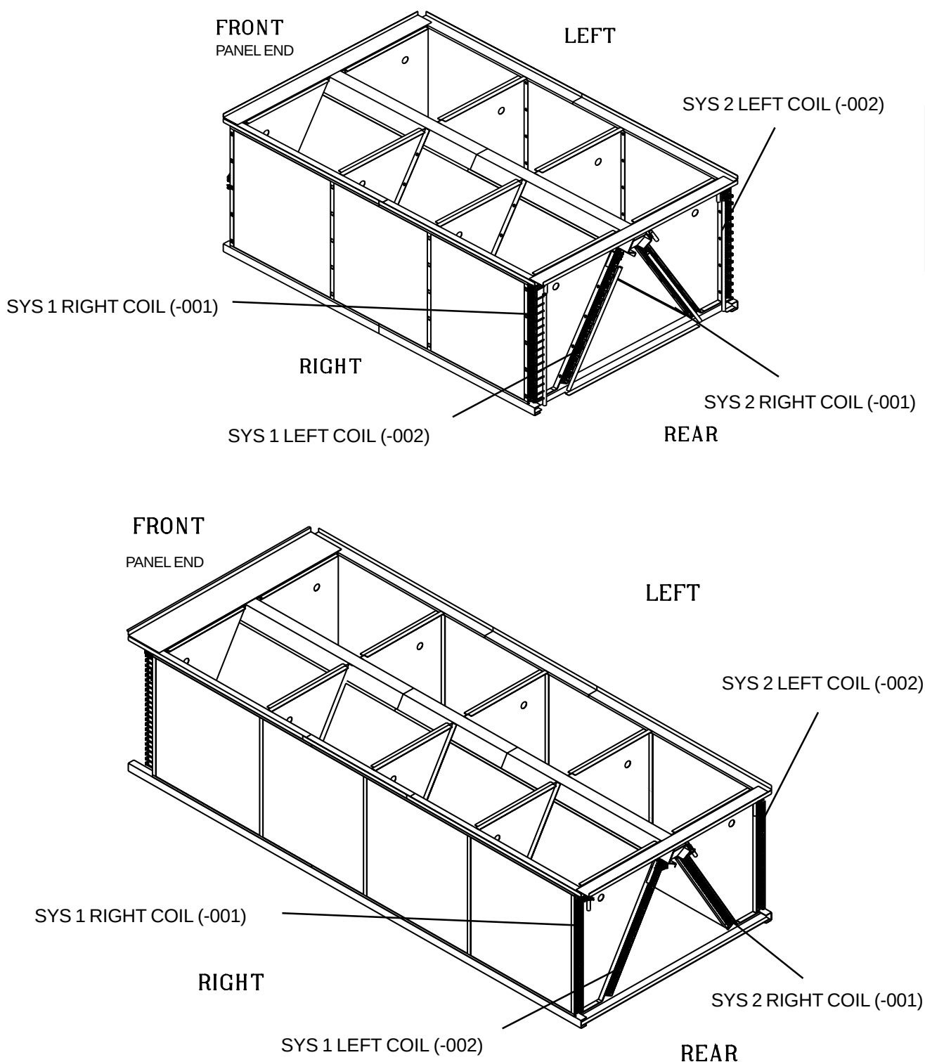
FIG. 3 – CONDENSER COIL LAYOUT - 12'-0" AND 16'-0" SHOWN
