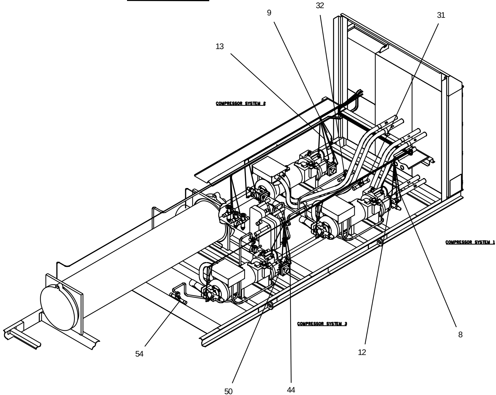
FIG. 16 – HARNESS LAYOUT (REF. TABLE 14, PAGES 29 AND 30)
