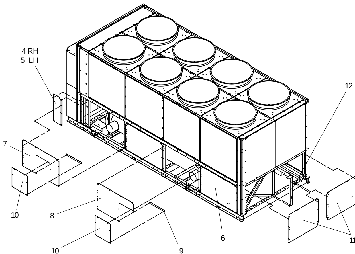
FIG. 28 – LOUVERED ENCLOSURE - 16'-0" KIT IS SHOWN.
