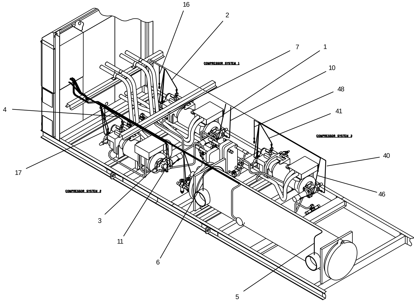
31 FIG. 15 – HARNESS LAYOUT (REF. TABLE 14, PAGES 29 AND 30)
