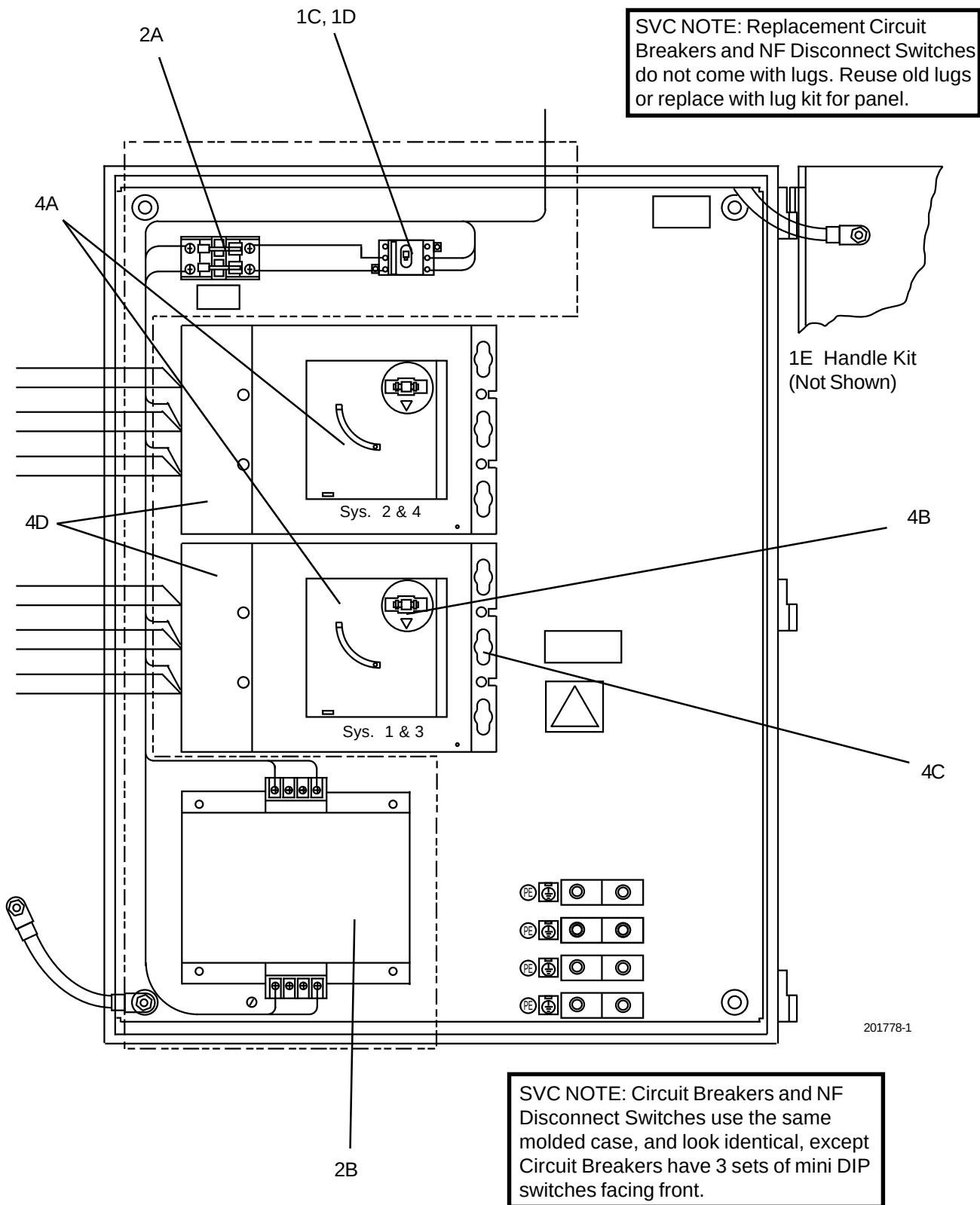
FIG. 24 – OPTION PANEL SHOWN WITH CIRCUIT BREAKER OR NON-FUSED DISCONNECT SWITCH (REF. TABLE 23, PAGES 48 AND 49)
