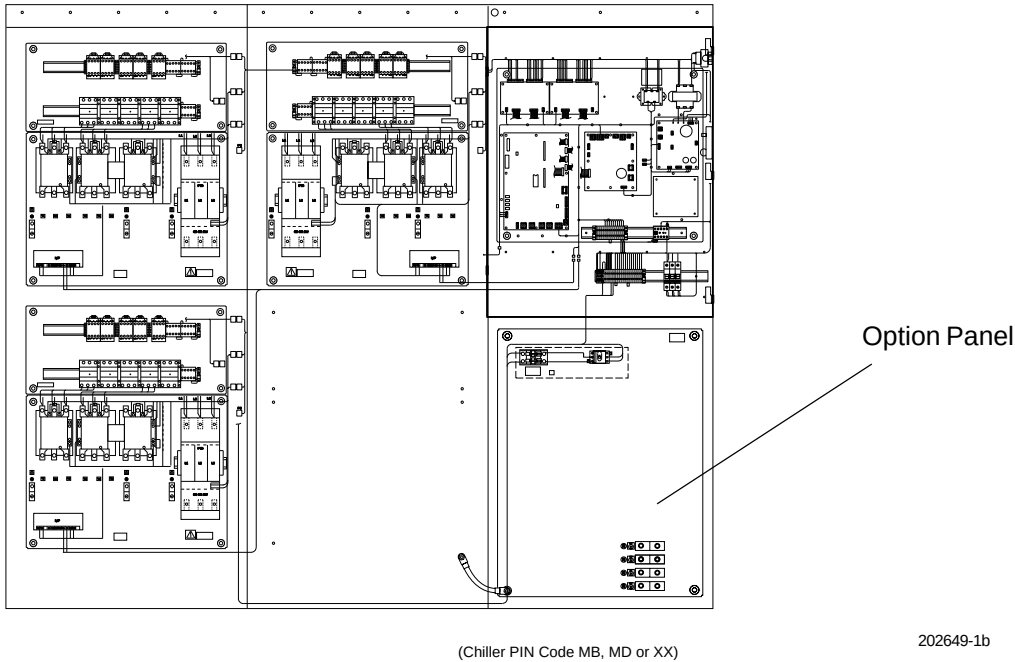
FIG. 22 – OPTION PANEL - (3-COMPRESSOR UNITS)
