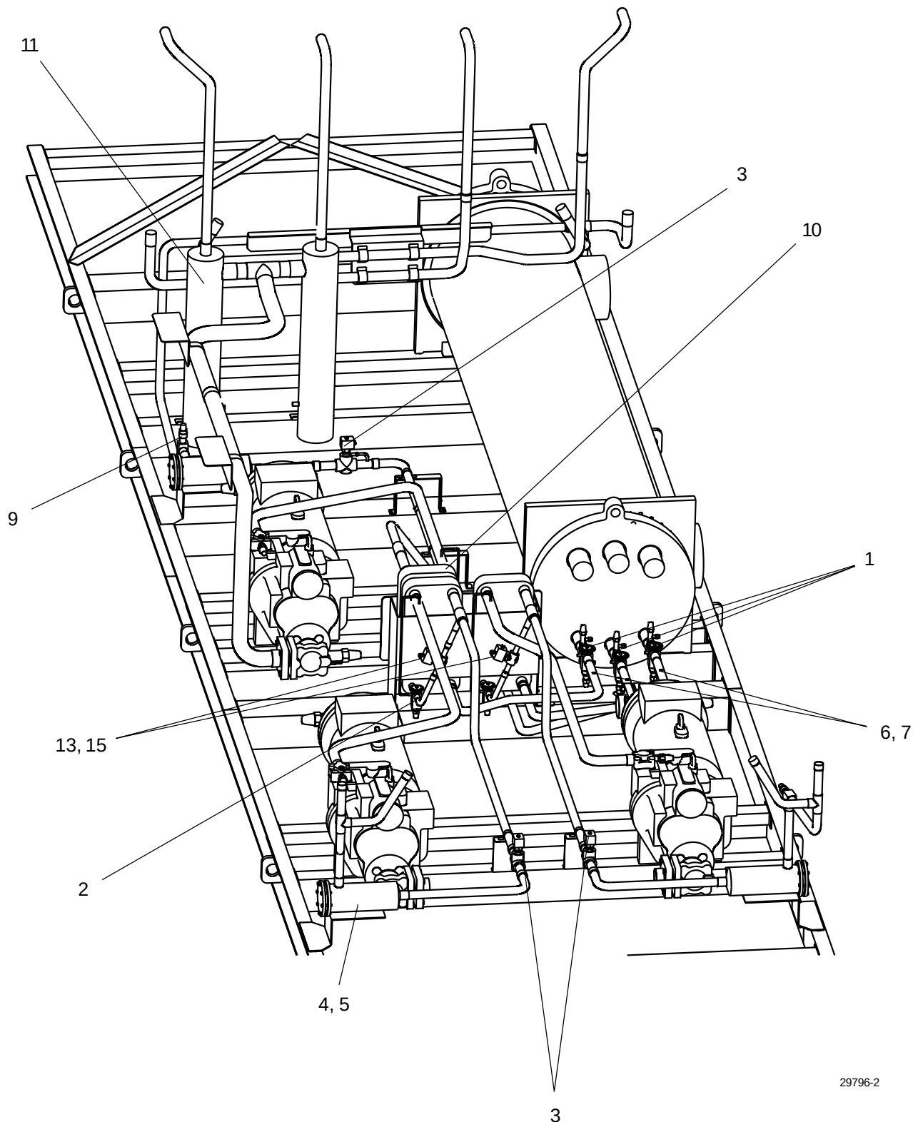
FIG. 7 – REFRIGERANT AND OIL PIPING COMPONENTS - MODEL YCAS0953 SHOWN (REF. TABLE 6, PAGE 10)
