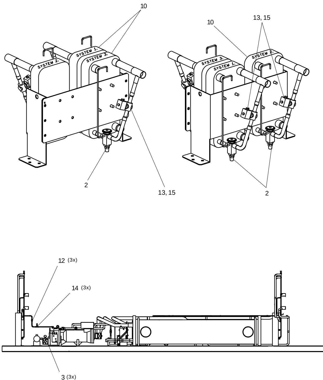
FIG. 8 – REFRIGERANT AND OIL PIPING COMPONENTS - MODEL YCAS0953 SHOWN (REF. TABLE 6, PAGE 10)
