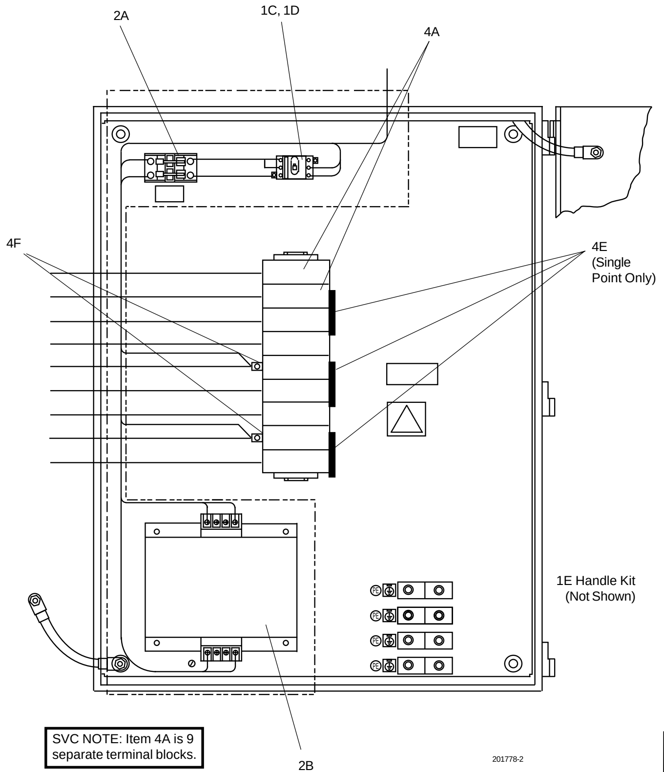
FIG. 25 – OPTION PANEL SHOWN WITH POWER TERMINAL BLOCK (REF. TABLE 23, PAGES 48 AND 49)
