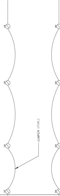
DETAIL "B" TYPICAL FOR INTERNALLY PROTECTED MOTORS
