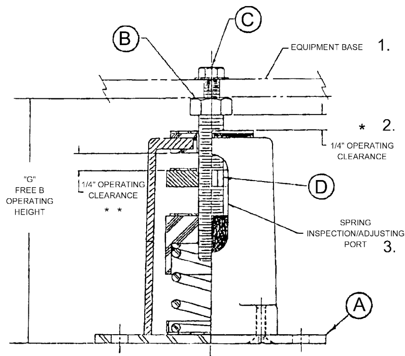
FIG. 38 – “AEQM” SPRING-FLEX MOUNTING
