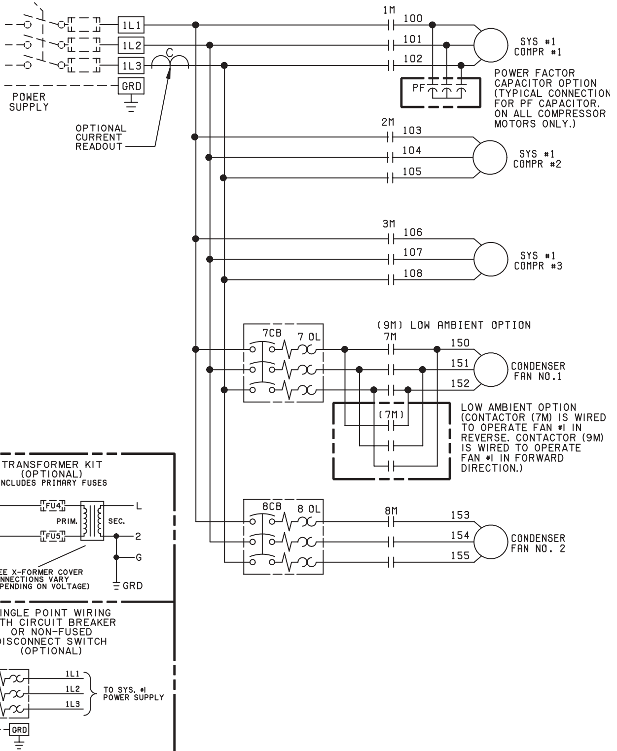
FIG. 21 – ELEMENTARY DIAGRAM, POWER CIRCUIT – YCAL0034E_
