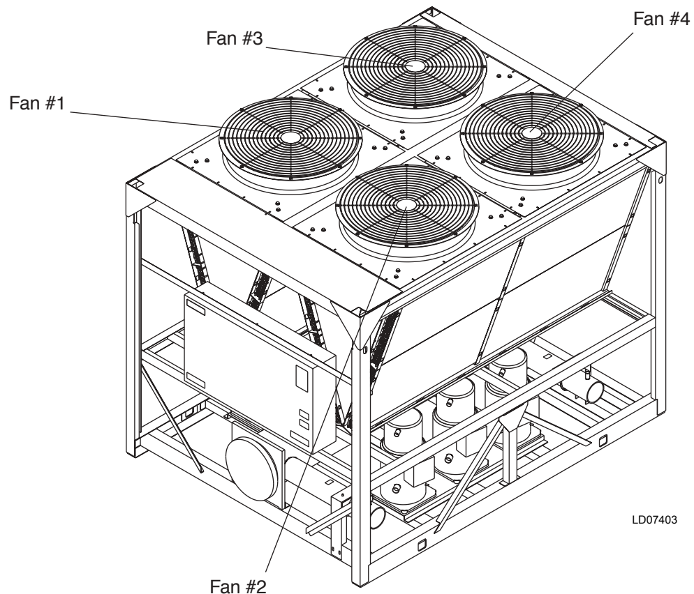
FIG. 9 – YCAL0014 – YCAL0080 FAN LOCATION (TYPICAL)
