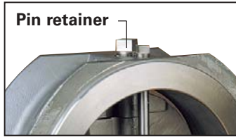
Conventional dual plate check valve design with pin retainers.
