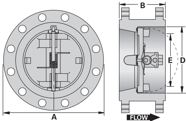
DIMENSIONS & WEIGHTS / PF & PG – Double Flanged Type – ASME Class 150
