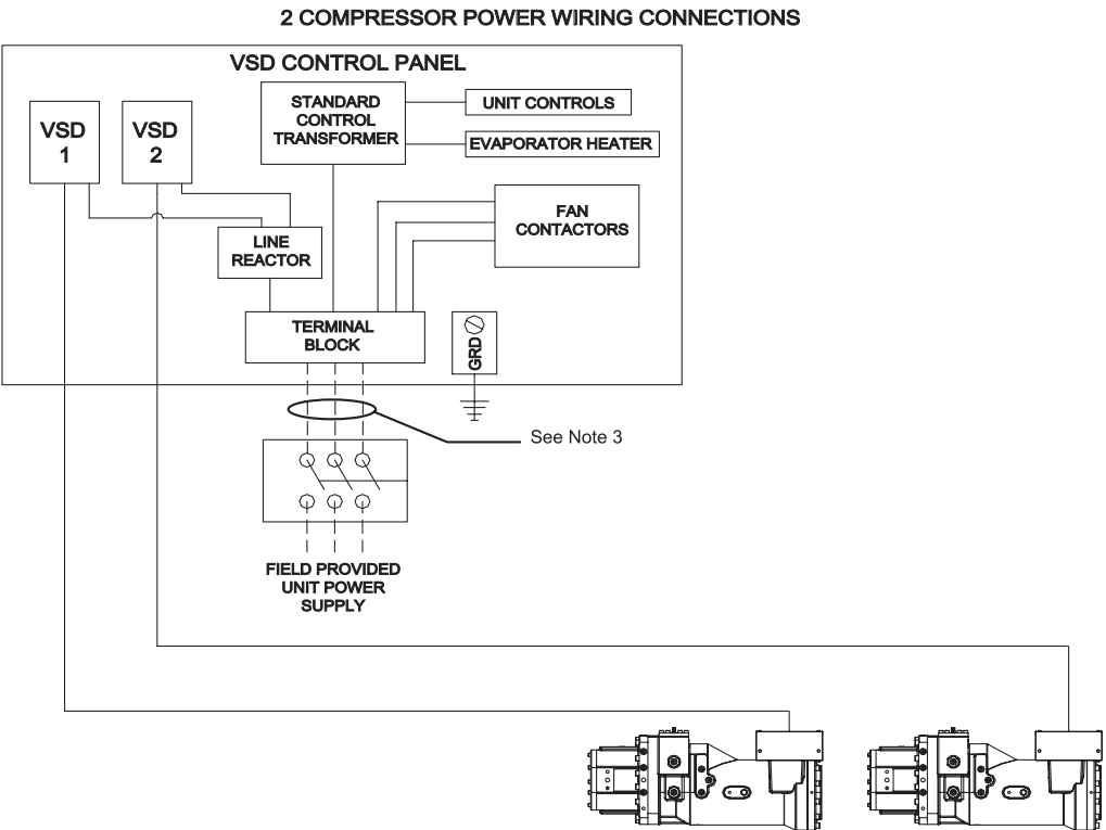
FIG. 2 – TWO COMPRESSOR WIRING DIAGRAM WITH TERMINAL BLOCK
