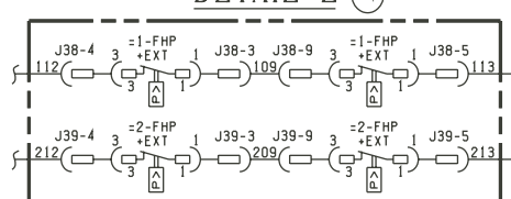
CONTROL ELEMENTARY DIAGRAM 2 COMPRESSOR YCAV/YCIV CHILLER 035-19905-001 REV. H
