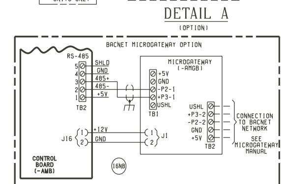
CONTROL ELEMENTARY DIAGRAM 2 COMPRESSOR YCAV/YCIV CHILLER 035-19905-001 REV. H
