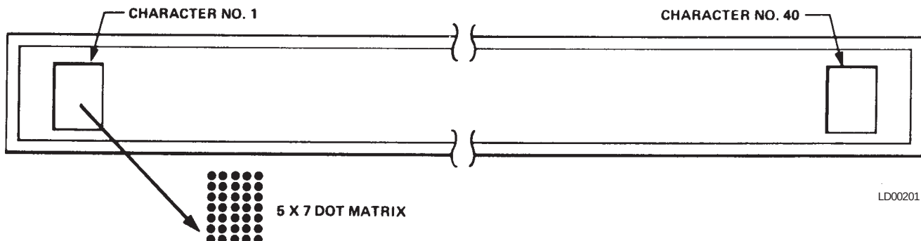
FIG. 29 – VACUUM FLUORESCENT DISPLAY
