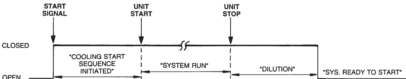
FIG. 18 – CONDENSER WATER PUMP CONTROL CONTACTS – RELAY BOARD TB4-55/56
