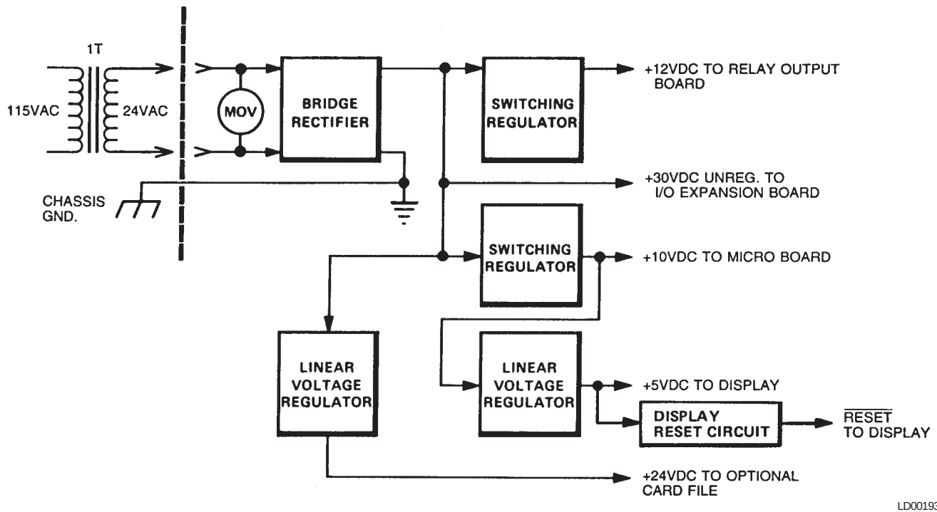
FIG. 19 – POWER SUPPLY BOARD BLOCK DIAGRAM
