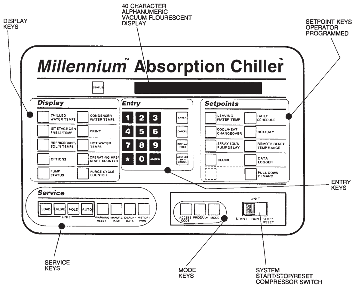
FIG. 1 – MILLENNIUM CONTROL CENTER KEYPAD
