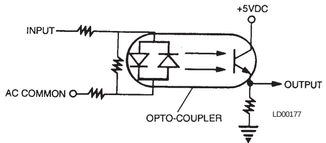
FIG. 6 – DETAILED SCHEMATIC REPRESENTATION DIGITAL INPUT BOARD
