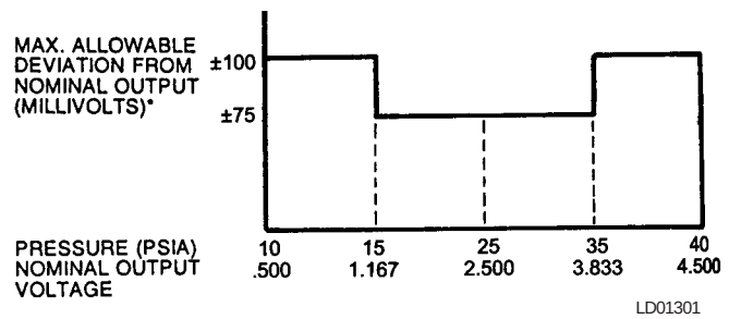
FIG. 27 – STEAM SUPPLY PRESS. TRANSDUCER YORK PART NO.025-29148-001
