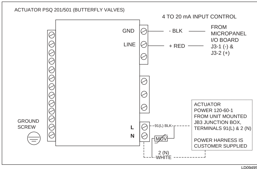
FIG. 2 - PSQ 201/501 BUTTERFLY VALVES
