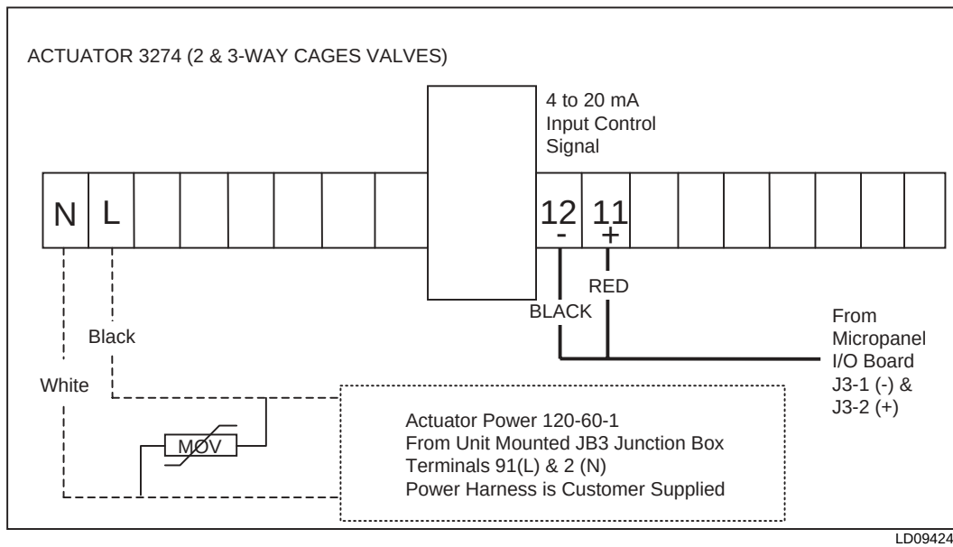
FIG. 1 - ACTUATOR WIRING , 2 & 3-WAY CAGE VALVES
