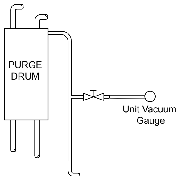
FIGURE 8 - BREAKING UNIT PRESSURE
