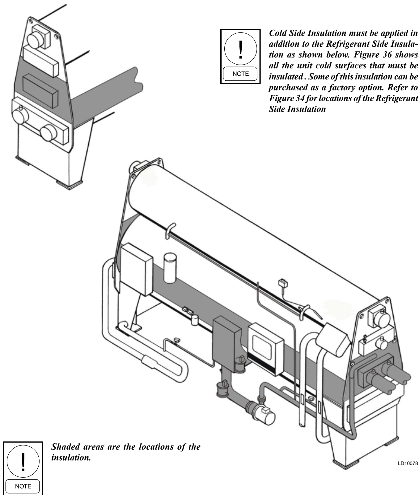
FIGURE 36 - REFRIGERANT SIDE AND COLD SIDE INSULATION
