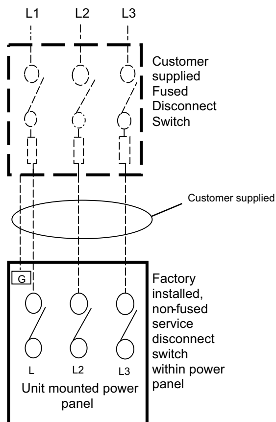
FIGURE 30 - INCOMING 3 PHASE POWER WIRING
