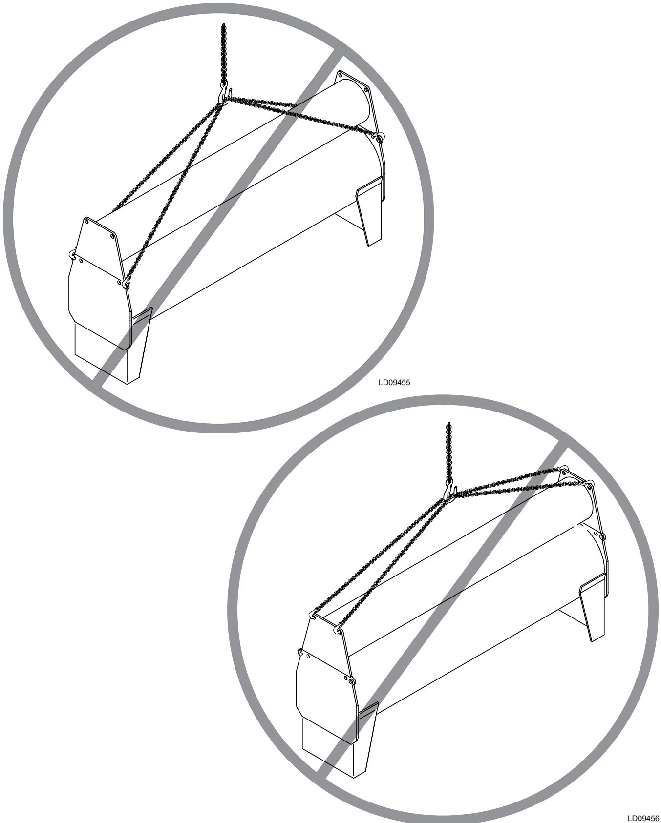
FIGURE 5 - INCORRECT ONE-PIECE UNIT LIFTING METHODS
