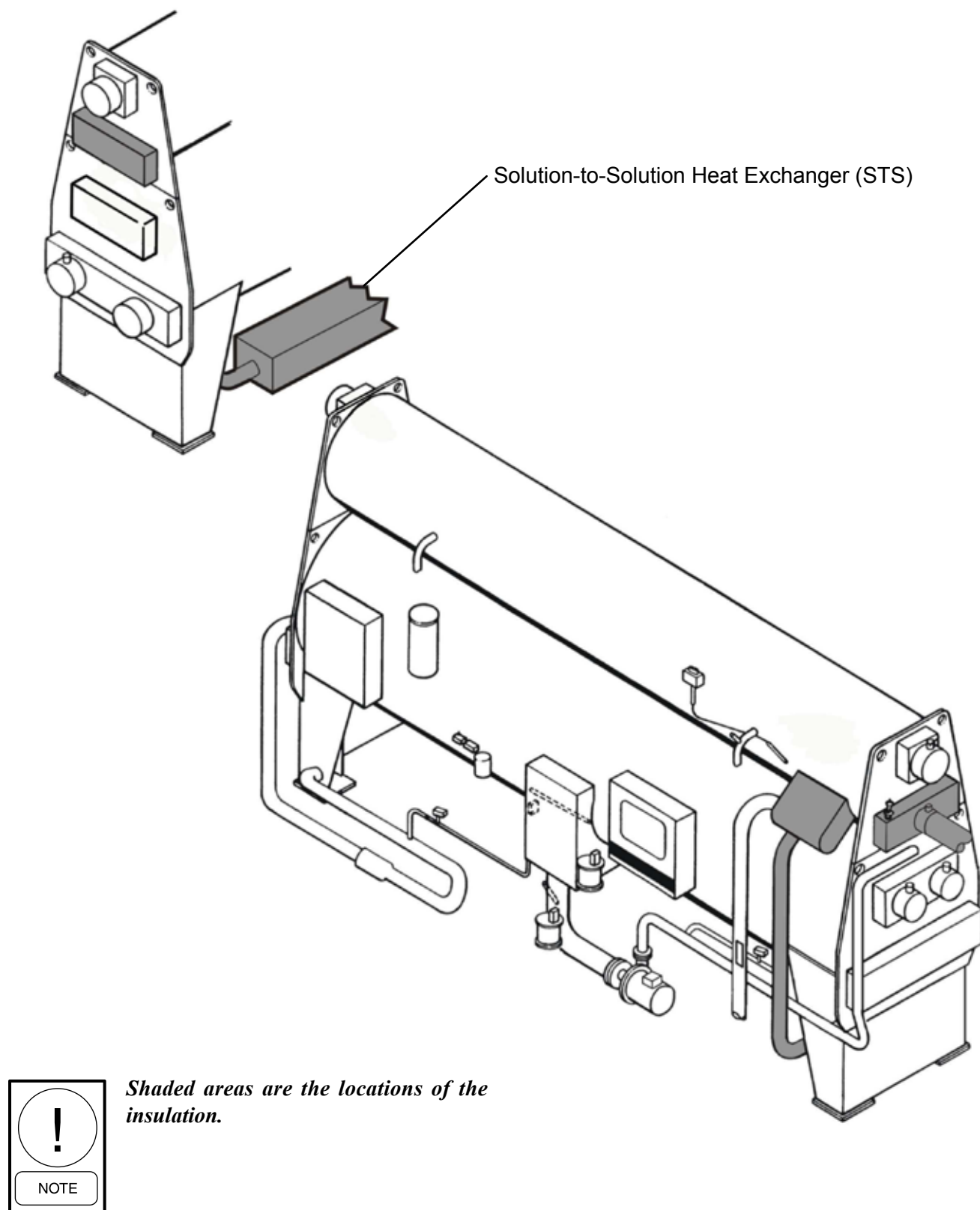
FIGURE 37 - HOT SURFACES INSULATION (FIELD SUPPLIED)
