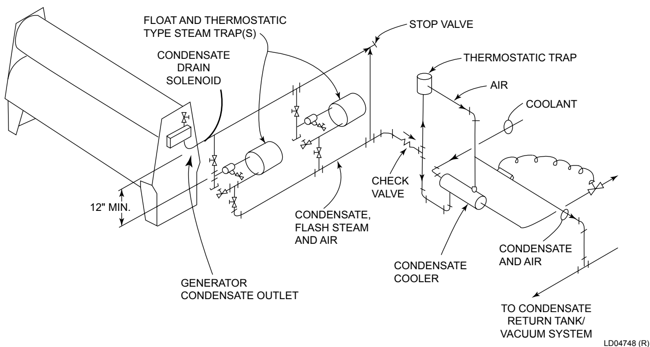
FIGURE 24 - SYSTEM 3 - VACUUM CONDENSATE RETURN SYSTEM WHEN INLET STEAM AND OUTLET CONDENSATE ARE UNDER VACUUM
