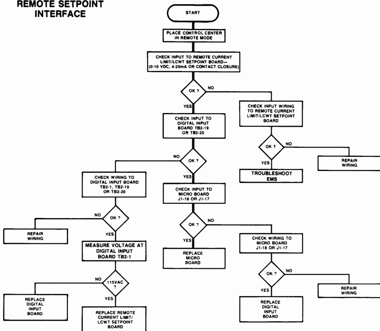
FIG. 52 — REMOTE SETPOINT INTERFACE
