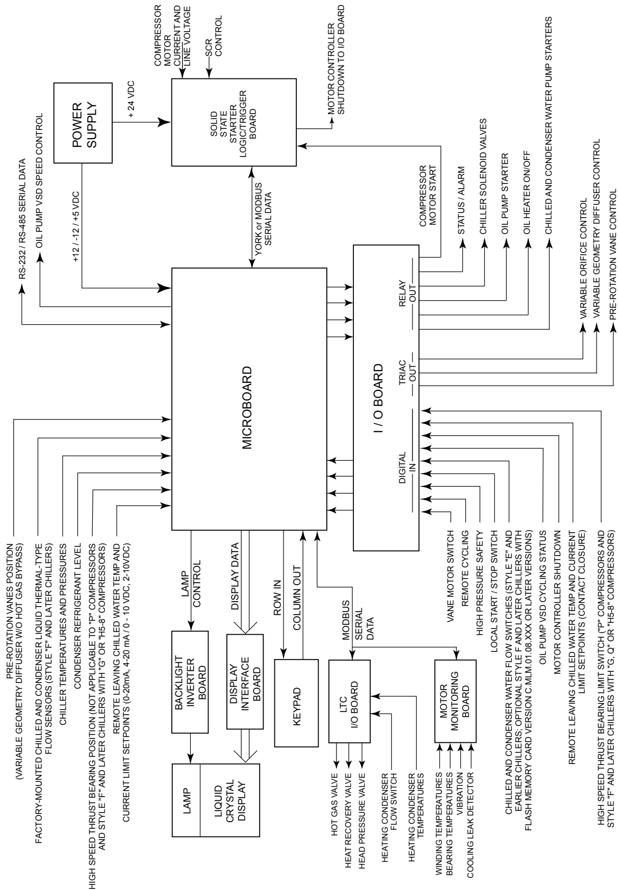
FIGURE 3 - OPTIVIEW™ CONTROL CENTER - MOD B SOLID STATE STARTER APPLICATIONS
