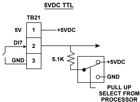
FIGURE 85 - +5VDC DIGITAL INPUT
