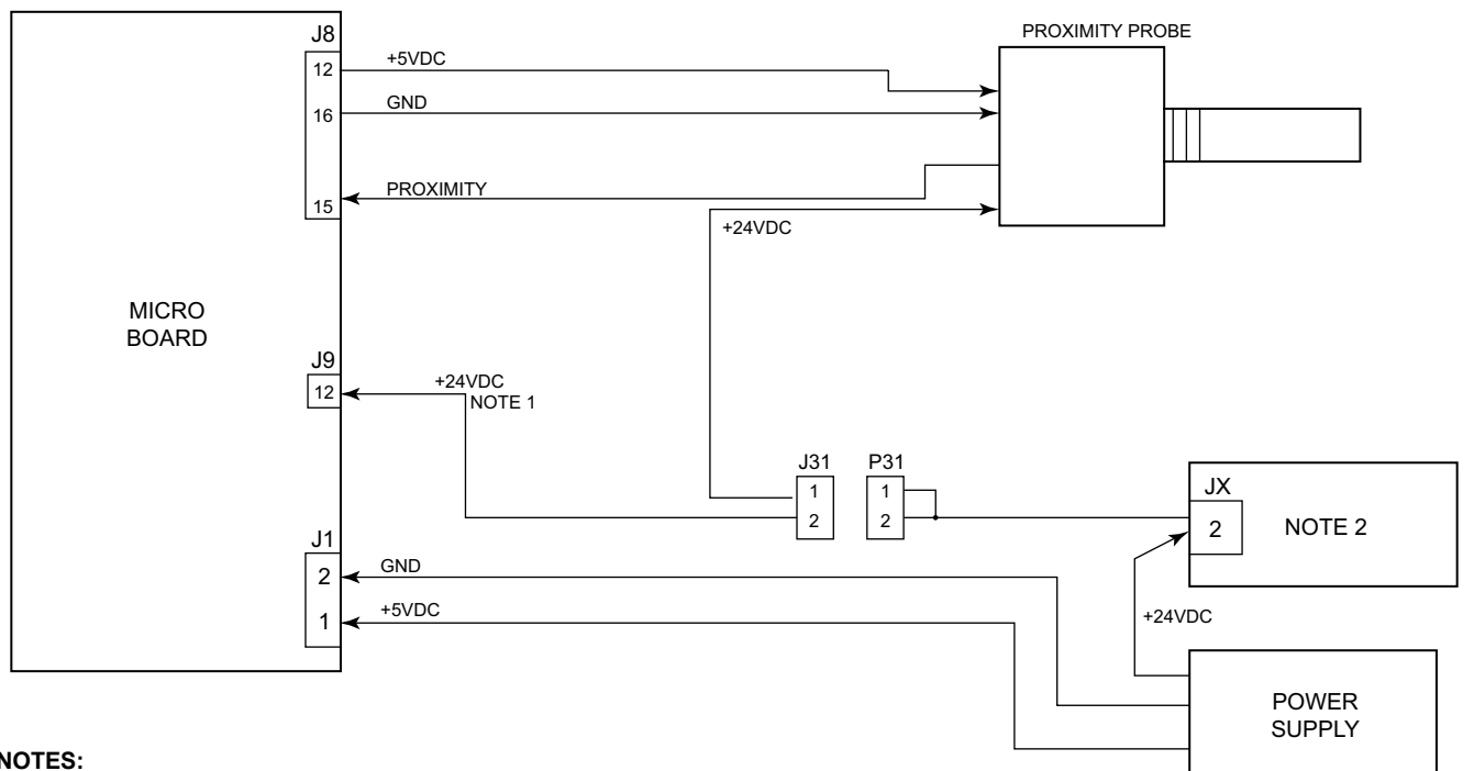
FIGURE 66 - PROXIMITY PROBE INTERFACE – PROBE PART NUMBER 025-30961-000
