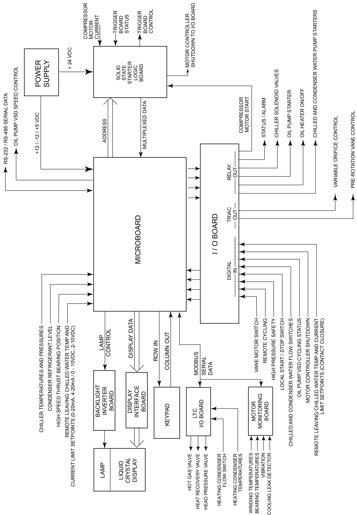
FIGURE 2 - OPTIVIEW™ CONTROL CENTER - MOD A SOLID STATE STARTER APPLICATIONS
