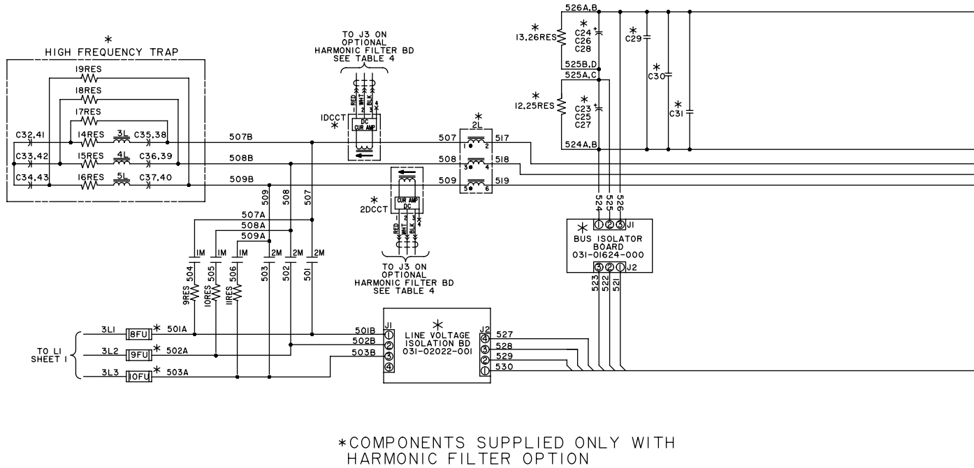
FIGURE 26 - HARMONIC FILTER WIRING DIAGRAM 608 HP FOR VSD MODELS GLOBAL DESIGN AFTER DECEMBER 2006
