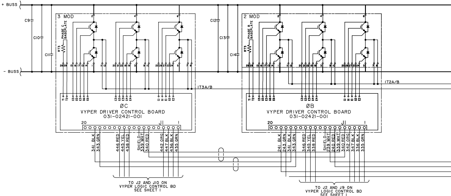
POWER ASSY ELEMENTARY
