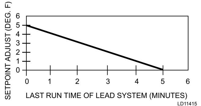
FIGURE 30 - SETPOINT ADJUST
