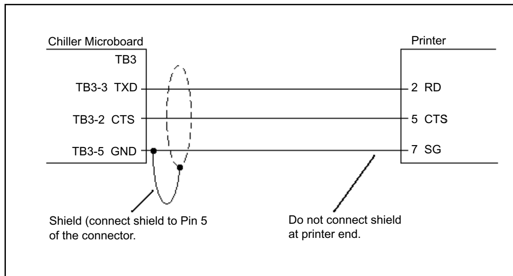
FIGURE 34 - PRINTER TO MICROBOARD ELECTRICAL CONNECTIONS
