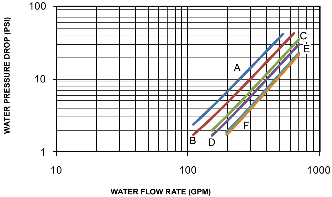
YLAA EVAPORATOR PRESSURE DROP (ENGLISH UNITS)
