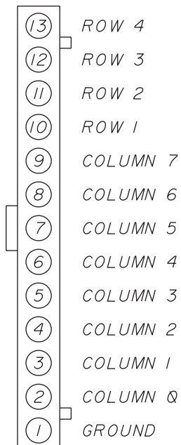
CONNECTOR PIN OUT
