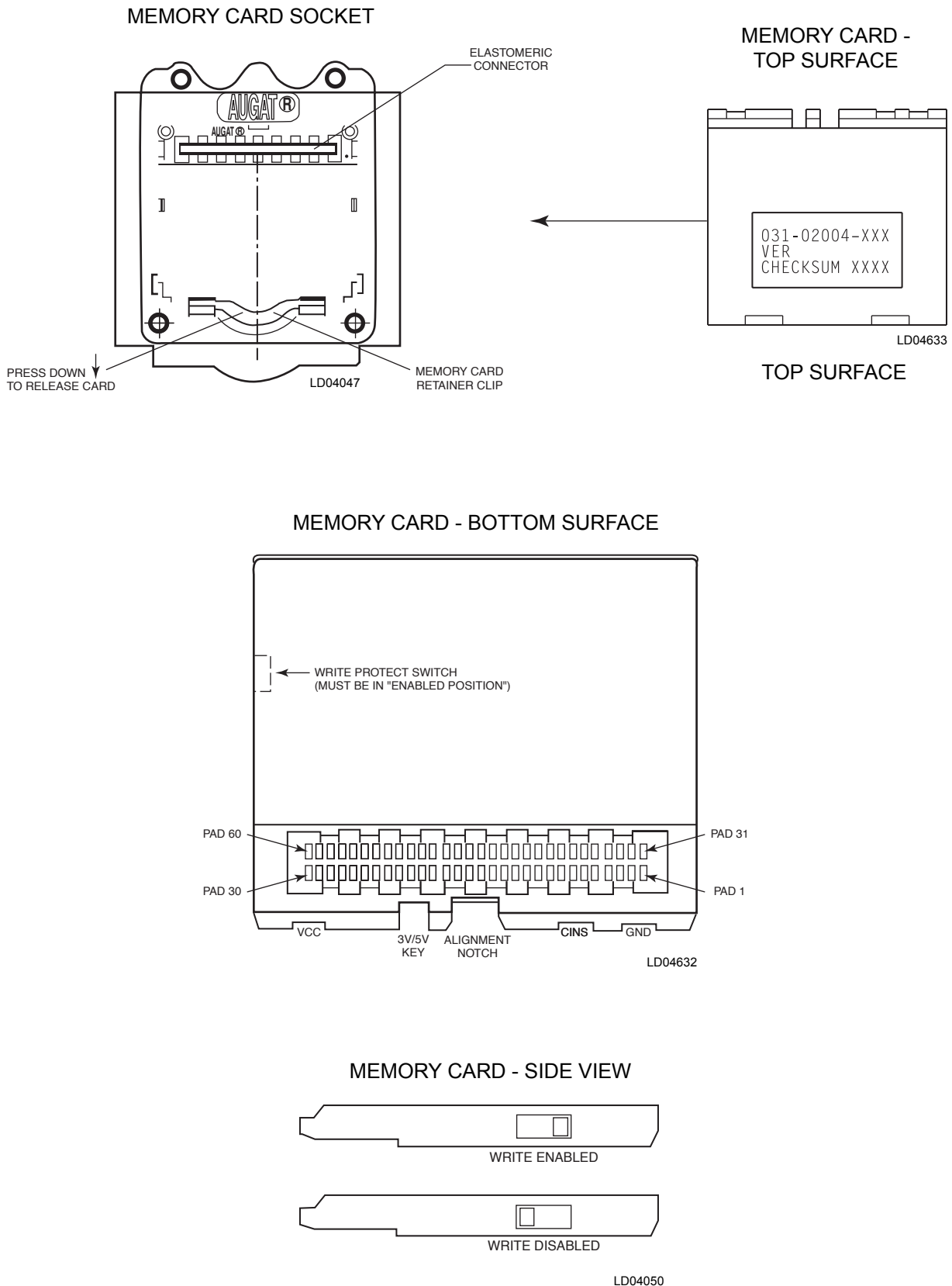
FIG. 8 – FLASH MEMORY CARD
