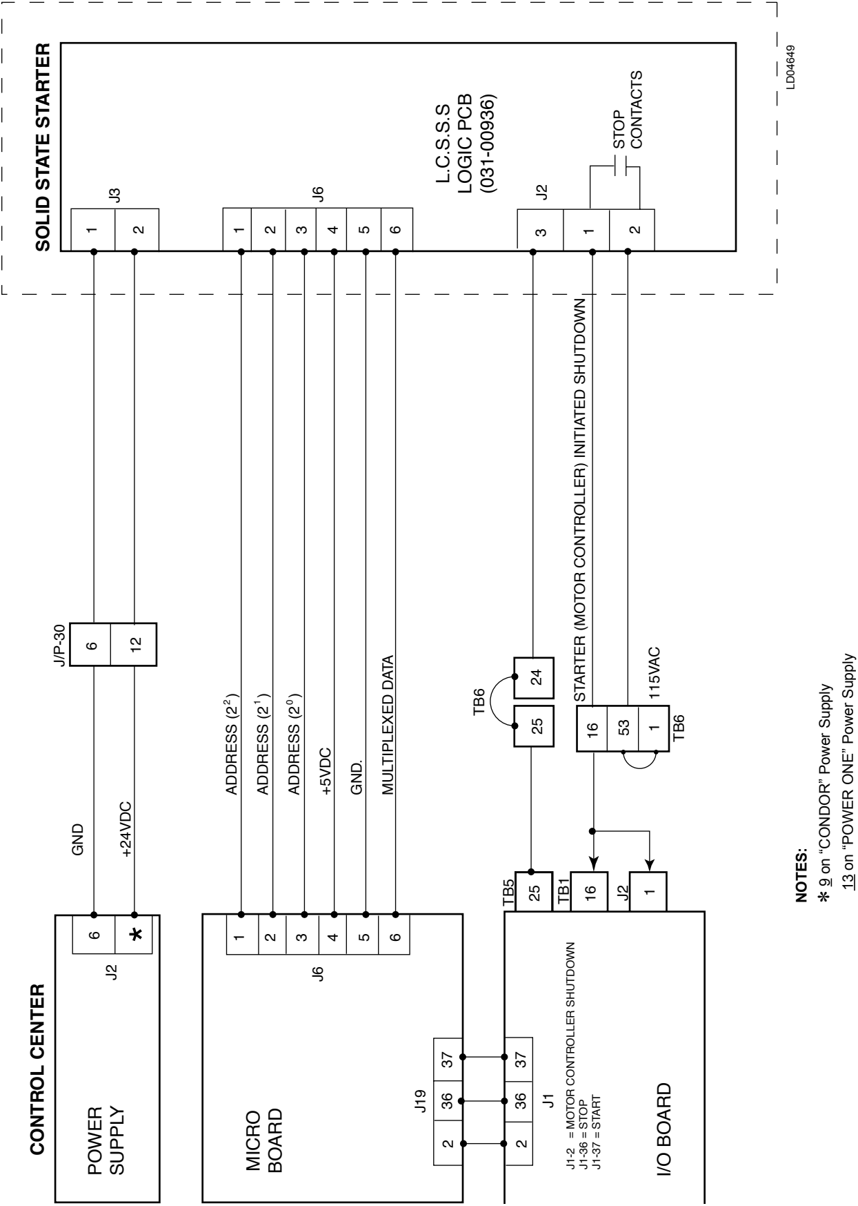
FIG. 41 – MOD "A" LIQUID COOLED SOLID STATE STARTER (LCSSS) - INTERFACE
