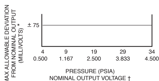
CONDENSER PRESSURE YORK PART NO. 025-29148-019
