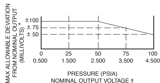
PURGE PRESSURE YORK PART NO. 025-29148-008
