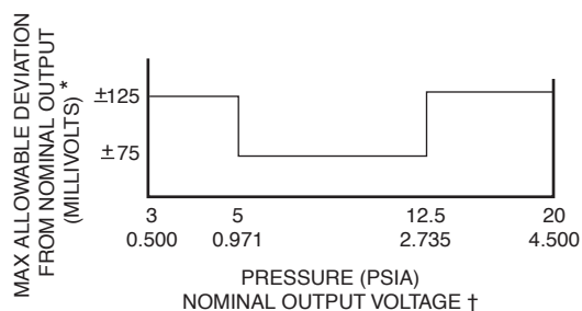
SUMP OIL PRESSURE YORK PART NO. 025-29148-003
