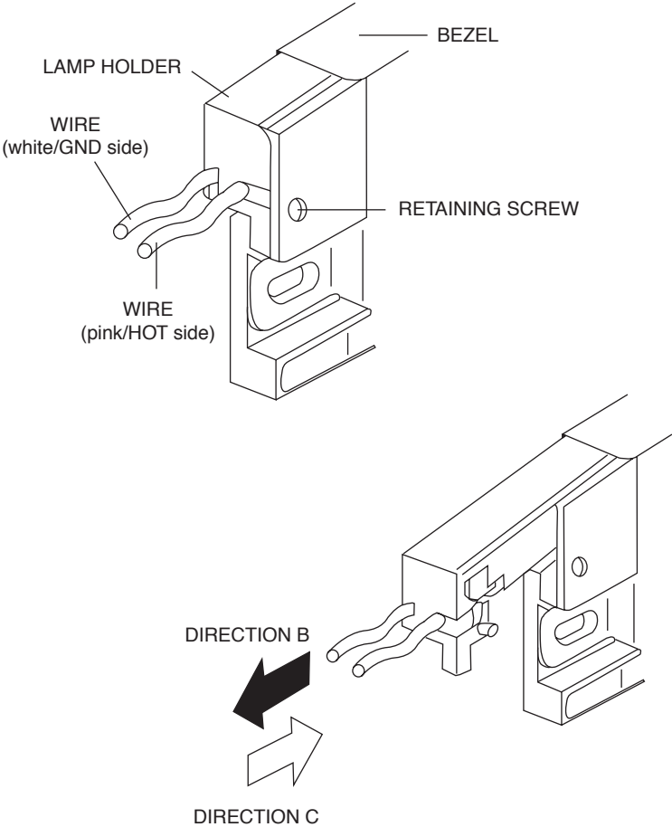
FIG. 27 – DISPLAY (LG SEMICON LP104V2-W) (031-02046-000) LAMP REPLACEMENT
