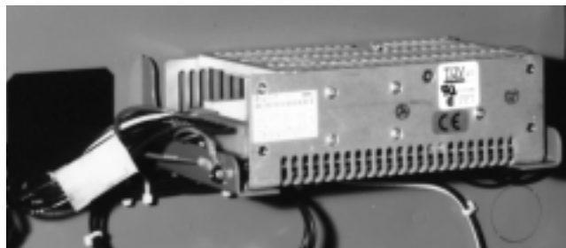
FIG. 34 – POWER SUPPLY
