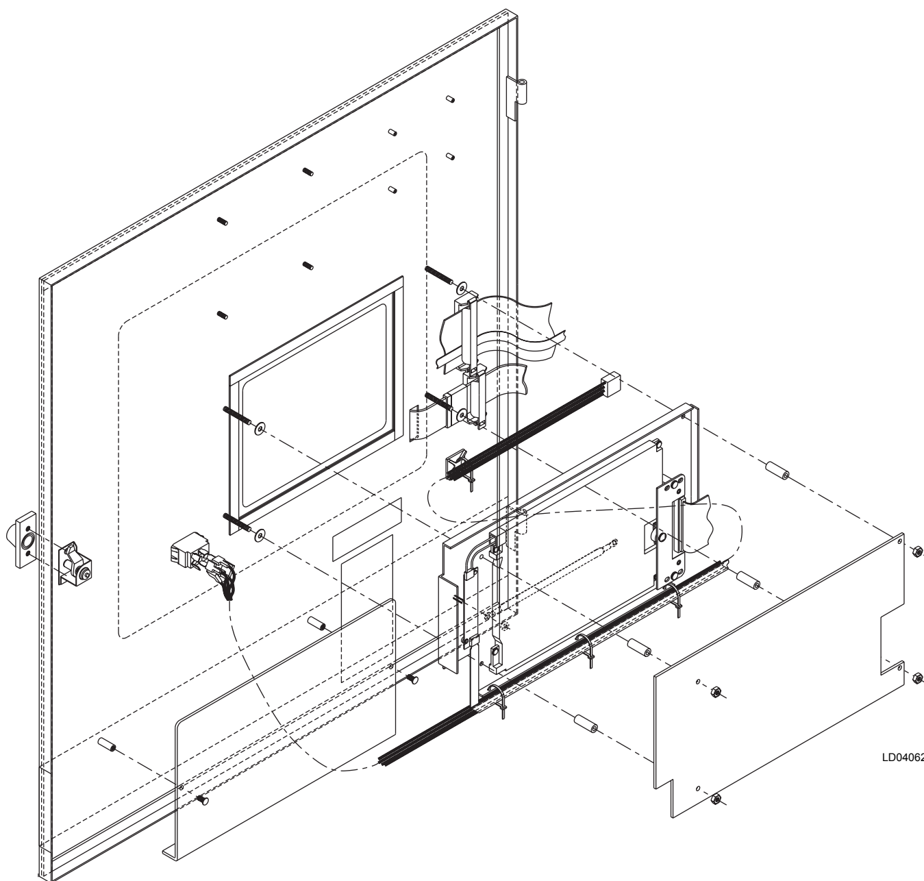
FIG. 18 – DISPLAY, MOUNTING
