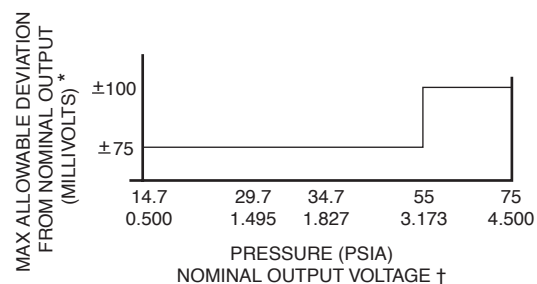
PUMP OIL PRESSURE YORK PART NO. 025-29148-004
