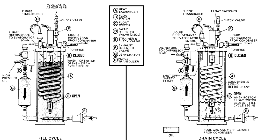
FIG. 46 – PURGE SYSTEM
