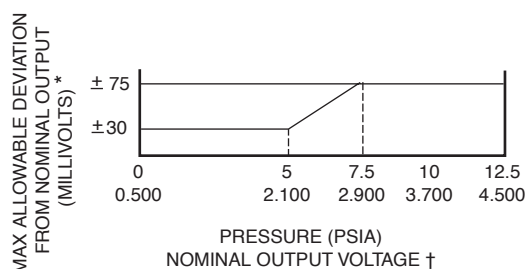
EVAPORATOR PRESSURE YORK PART NO. 025-29148-102
