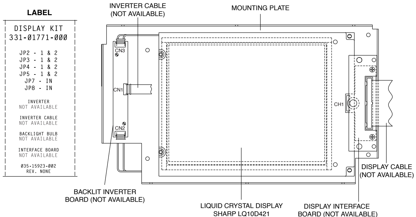
FIG. 19 – LIQUID CRYSTAL DISPLAY ASSEMBLY – SHARP LQ10D367/368 (031-01774-000) DISPLAY
