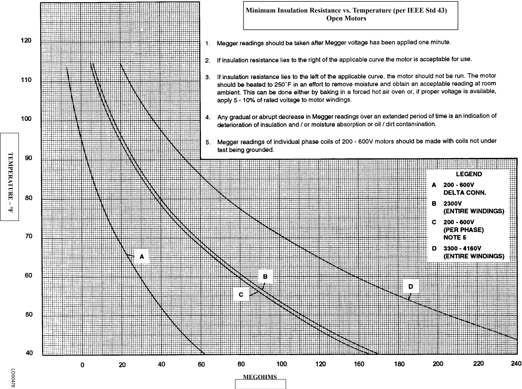
FIG. 66 – MOTOR STATOR TEMPERATURE AND INSULATION RESISTANCES
