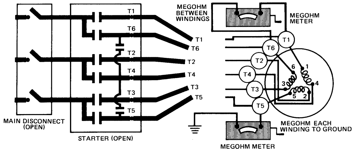
FIG. 65 – DIAGRAM, MEGGING MOTOR WINDINGS
